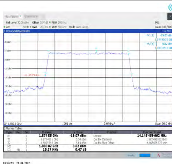
1-N25--15-15-M-9-CP-256QAM-Outer_Full-79@0-Ant0 0-14.145-15.270≤15-PASS
