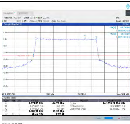
1-N25--15-15-M-6-CP-QPSK-Outer_Full-79@0-Ant0 -14.133-15.210≤15-PASS
