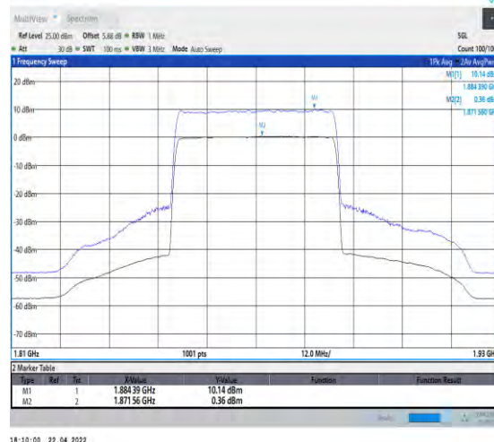
1-N25--15-40-L-2-CP-256QAM-Outer_Full-216@0-Ant0-9.78-100%-0.00-9.78-PASS-≤13
