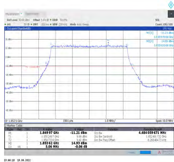
1-N25--15-5-L-2-DFT-PI2BPSK-Outer_Full-25@0-An t0-4.484-5.060-≤5-PASS
