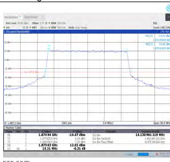
1-N25--15-15-M-7-CP-16QAM-Outer_Full-79@0-Ant0 0-14.131-15.210≤15-PASS
