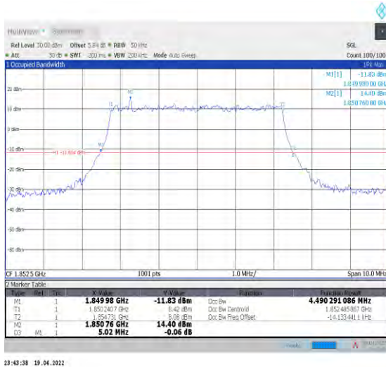
1-N25--15-5-L-1-DFT-QPSK-Outer_Full-25@0-Ant0-4.49-5.020-≤5-PASS
