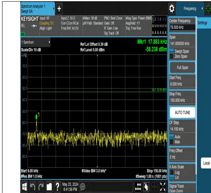
Band5_5MHz_QPSK_20425_1RB#0_0.009~0.15_0.009~0.15
