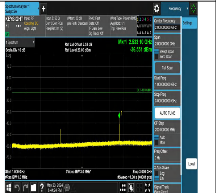
Band5_5MHz_QPSK_20625_1RB#0_1000~3000_1000~3000
