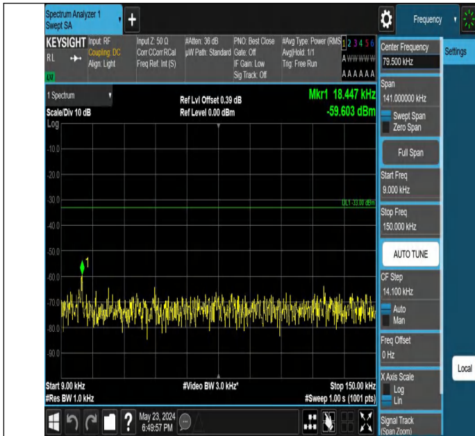
Band5_10MHz_QPSK_20525_1RB#0_0.009~0.15_0.009~0.15
