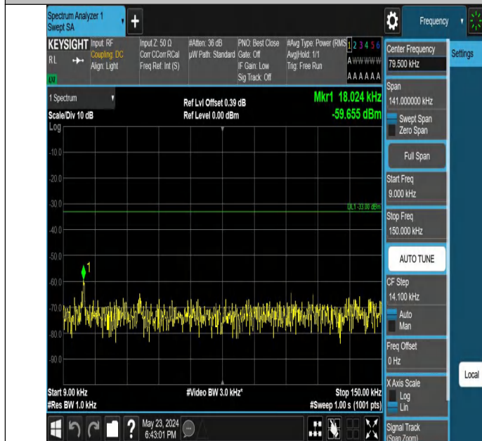
Band5_5MHz_QPSK_20525_1RB#0_0.009~0.15_0.009~0.15
