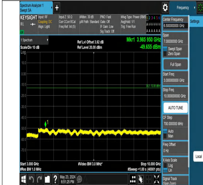
Band5_10MHz_QPSK_20600_1RB#0_3000~10000_3000~10000
