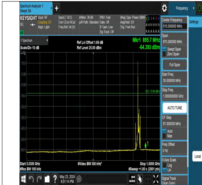
Band5_10MHz_QPSK_20600_1RB#0_30~1000_30~1000
