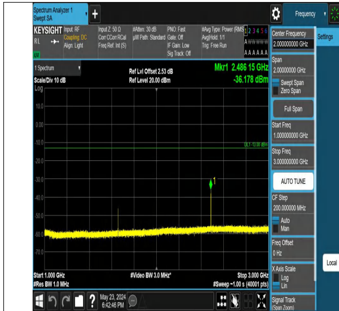
Band5_5MHz_QPSK_20425_1RB#24_1000~3000_1000~3000
