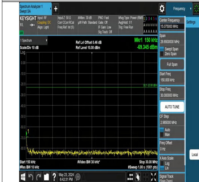
Band5_5MHz_QPSK_20425_1RB#24_0.15~30_0.15~30
