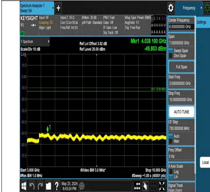
Band5_5MHz_QPSK_20525_1RB#0_3000~10000_3000~10000
