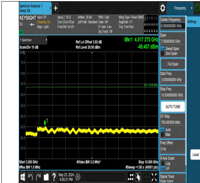
Band5_10MHz_QPSK_20525_1RB#0_3000~10000_3000~10000
