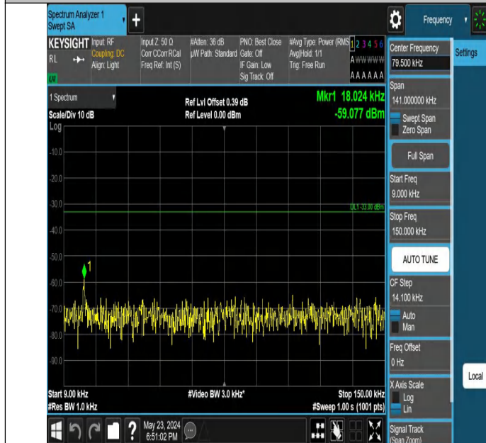
Band5_10MHz_QPSK_20600_1RB#0_0.009~0.15_0.009~0.15
