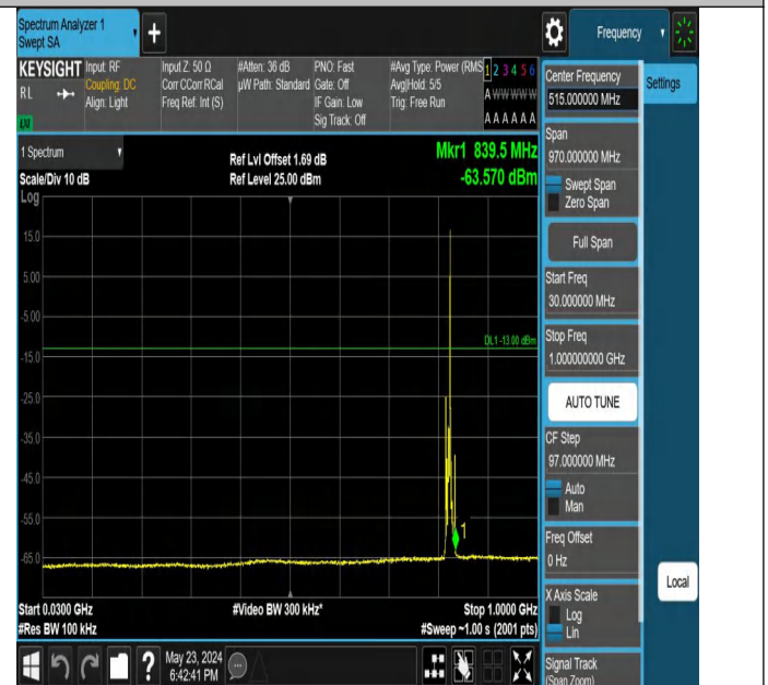
Band5_5MHz_QPSK_20425_1RB#24_30~1000_30~1000
