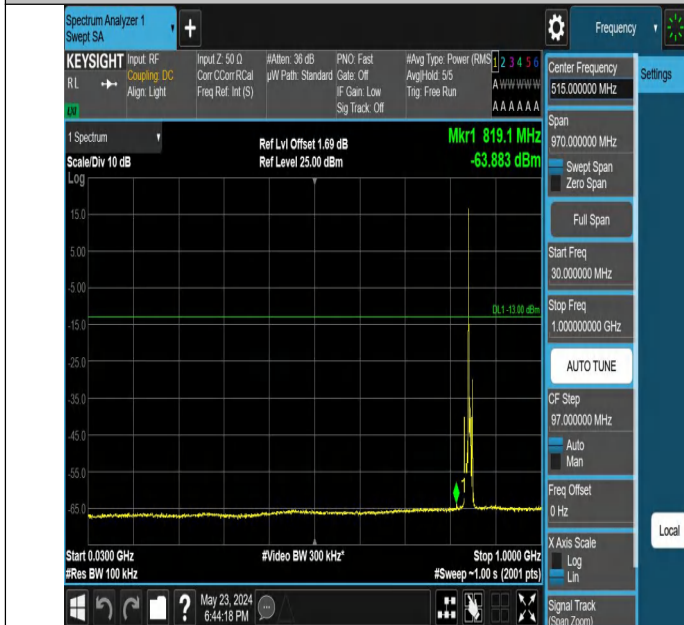
Band5_5MHz_QPSK_20625_1RB#0_30~1000_30~1000
