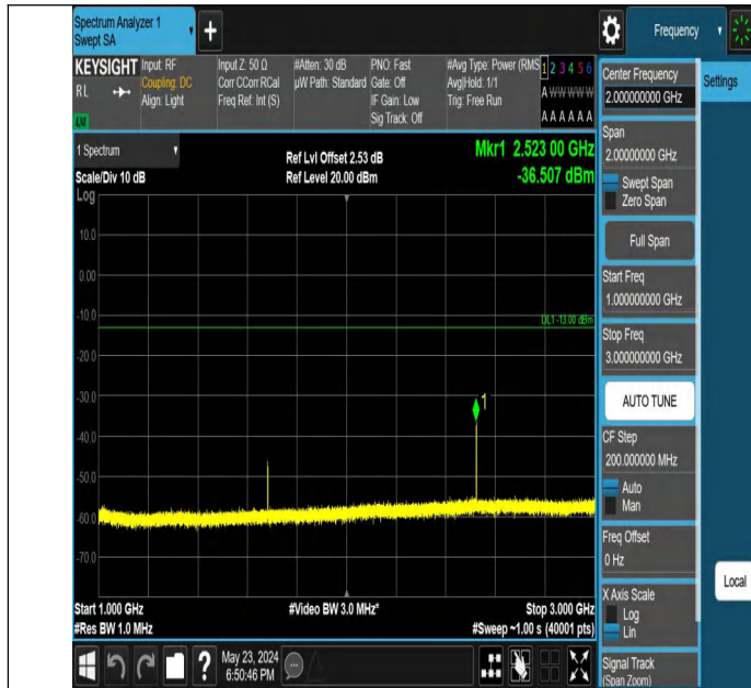
Band5_10MHz_QPSK_20525_1RB#49_1000~3000_1000~3000
