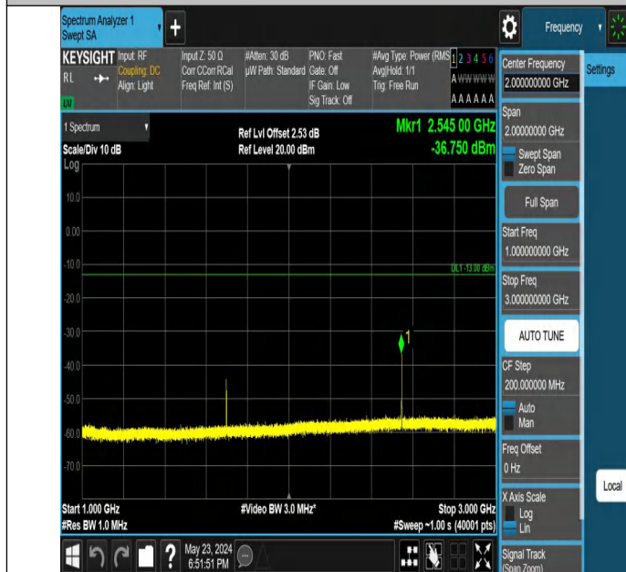
Band5_10MHz_QPSK_20600_1RB#49_1000~3000_1000~3000
