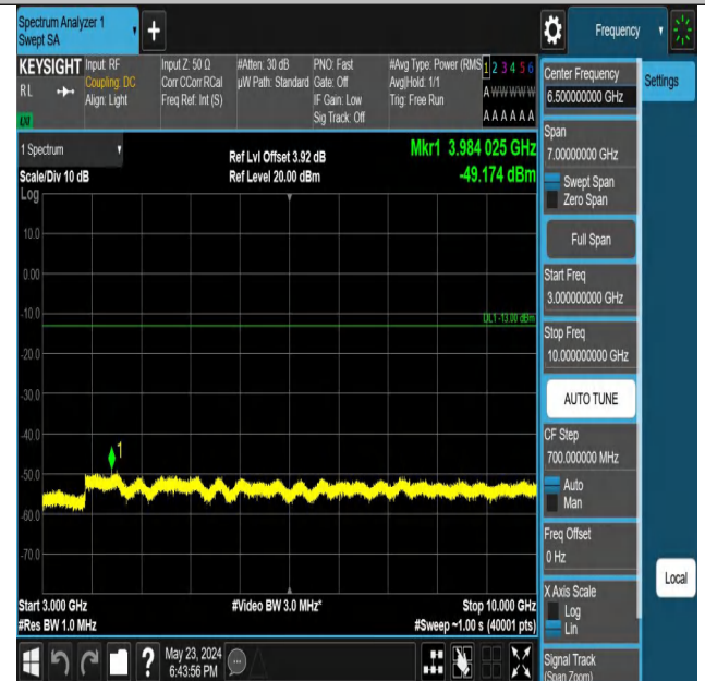
Band5_5MHz_QPSK_20525_1RB#24_3000~10000_3000~10000
