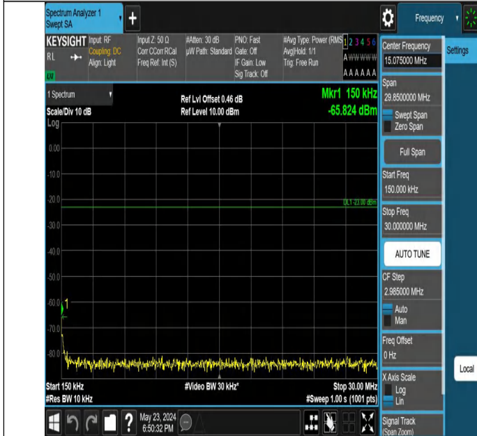
Band5_10MHz_QPSK_20525_1RB#49_0.15~30_0.15~30
