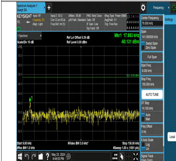
Band5_10MHz_QPSK_20450_1RB#0_0.009~0.15_0.009~0.15
