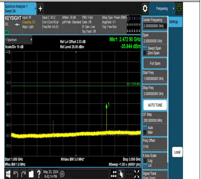
Band5_5MHz_QPSK_20425_1RB#0_1000~3000_1000~3000
