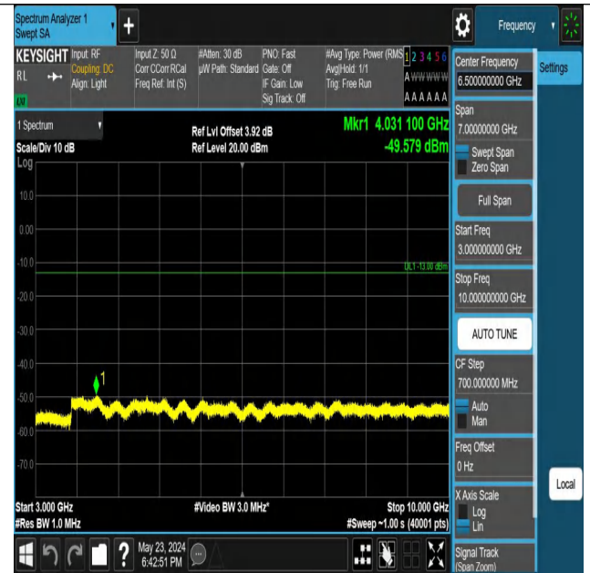
Band5_5MHz_QPSK_20425_1RB#24_3000~10000_3000~10000
