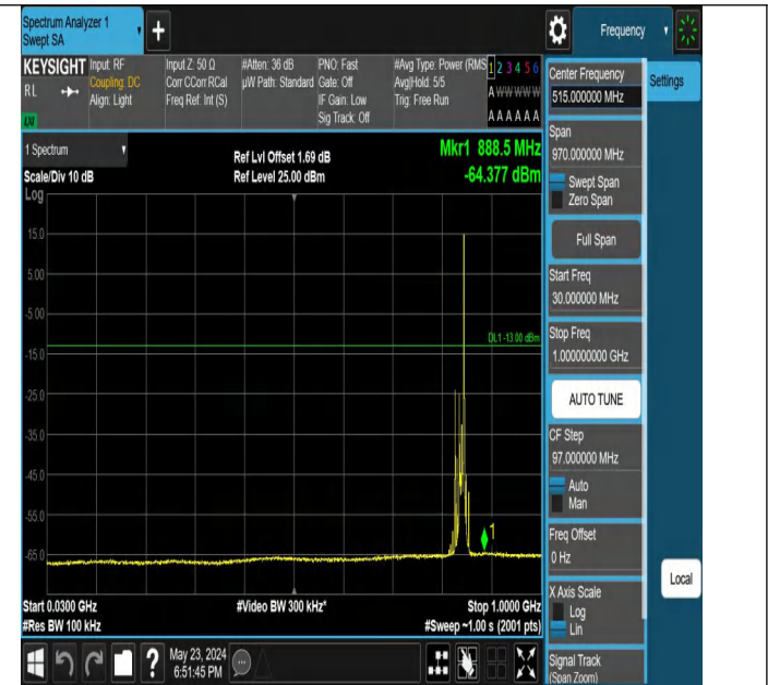
Band5_10MHz_QPSK_20600_1RB#49_30~1000_30~1000
