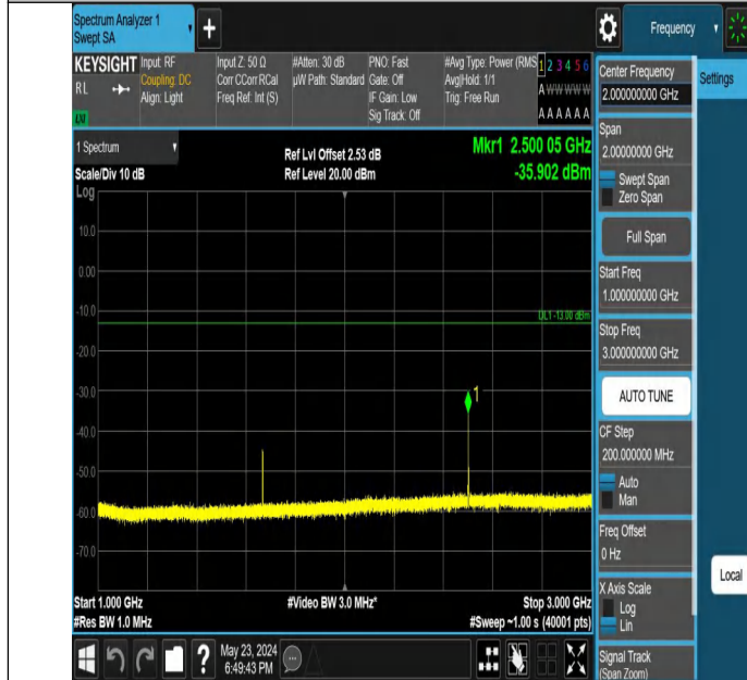
Band5_10MHz_QPSK_20450_1RB#49_1000~3000_1000~3000
