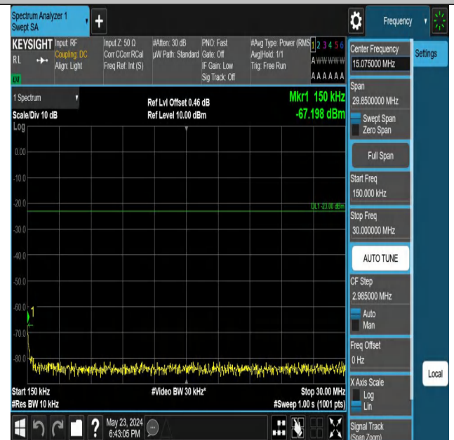
Band5_5MHz_QPSK_20525_1RB#0_0.15~30_0.15~30
