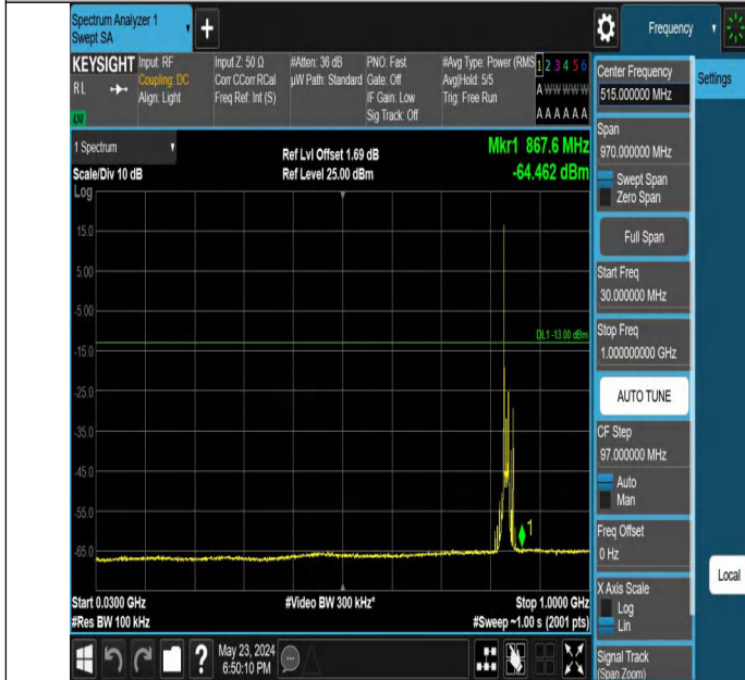
Band5_10MHz_QPSK_20525_1RB#0_30~1000_30~1000
