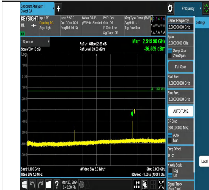
Band5_5MHz_QPSK_20525_1RB#24_1000~3000_1000~3000
