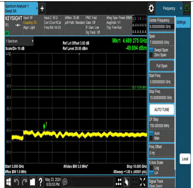
Band5_10MHz_QPSK_20525_1RB#49_3000~10000_3000~10000
