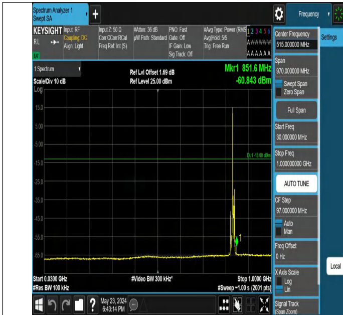
Band5_5MHz_QPSK_20525_1RB#0_30~1000_30~1000
