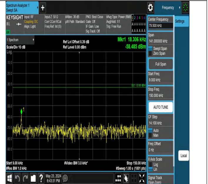
Band5_5MHz_QPSK_20525_1RB#24_0.009~0.15_0.009~0.15
