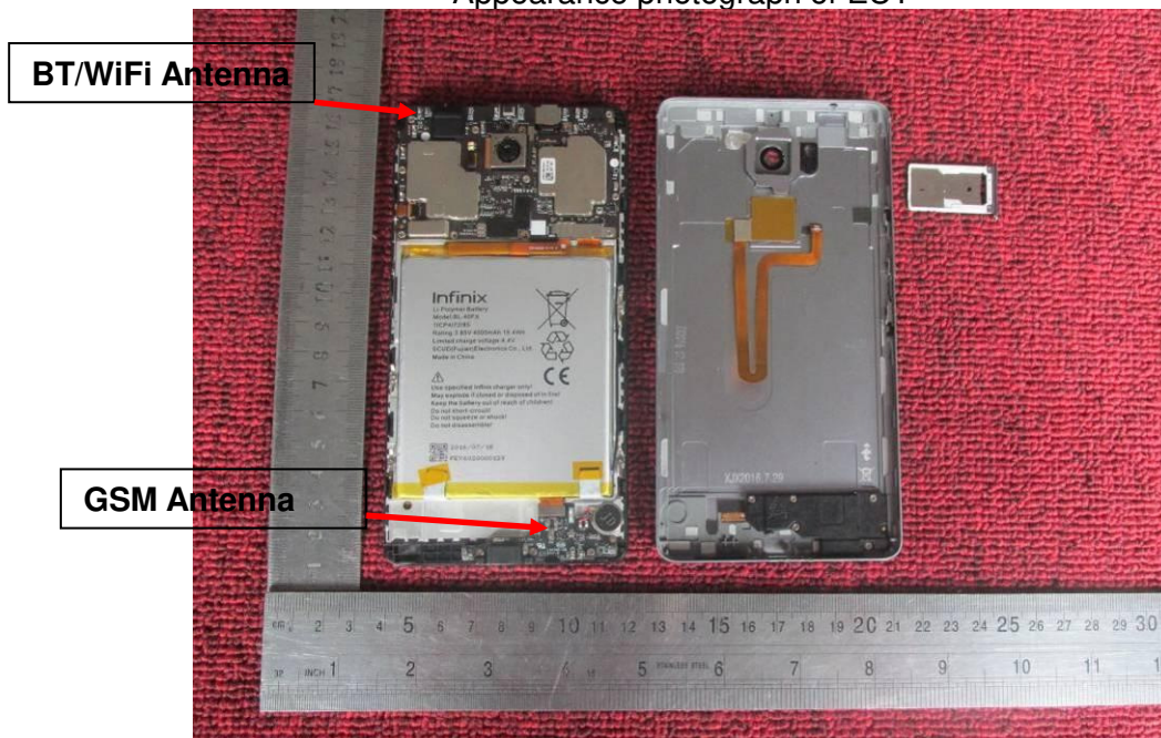
Appearance photograph of EUT
