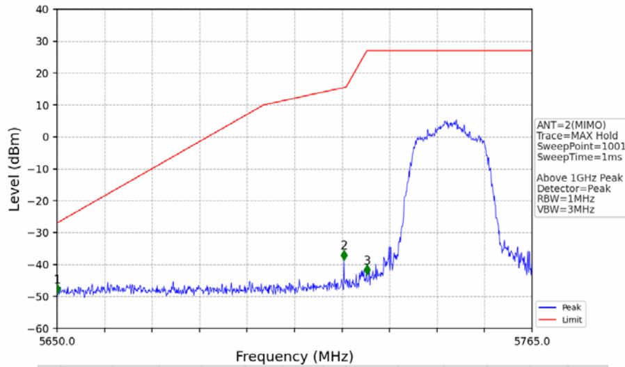
802.11ac(VHT20)_LCH_5745MHz_Ant2_NTNV
