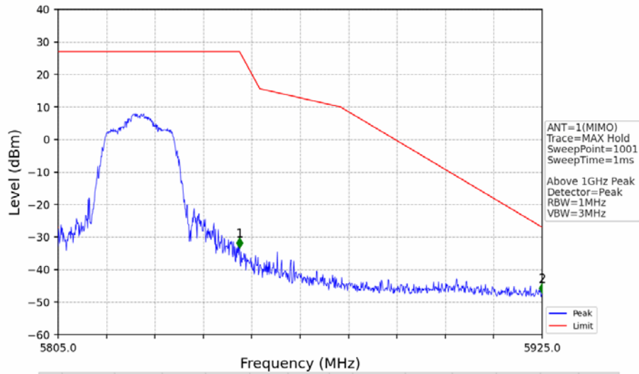
802.11ac(VHT20)_HCH_5825MHz_Ant1_NTNV
