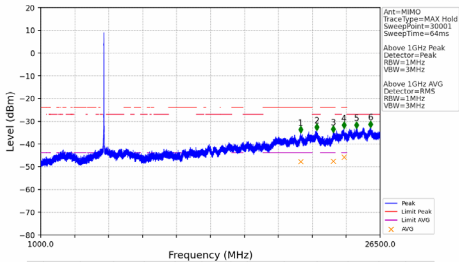
802.11ac(VHT20)_LCH_5745MHz_MIMO_NTNV
