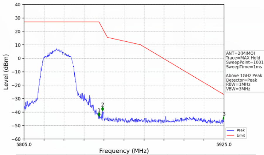
802.11ac(VHT20)_HCH_5825MHz_Ant2_NTNV
