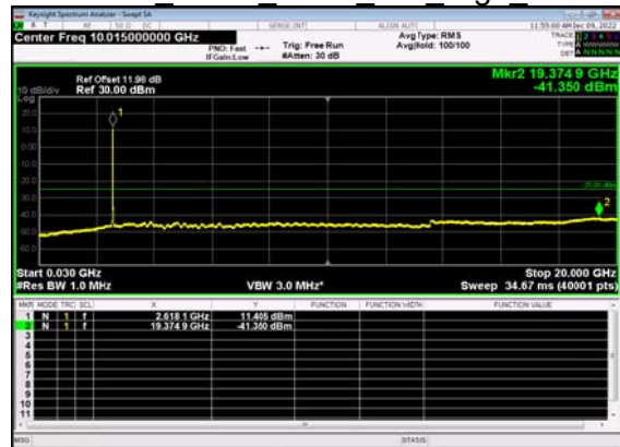
N38(15M)_DFT-s- OFDM BPSK Outer Full High CH
