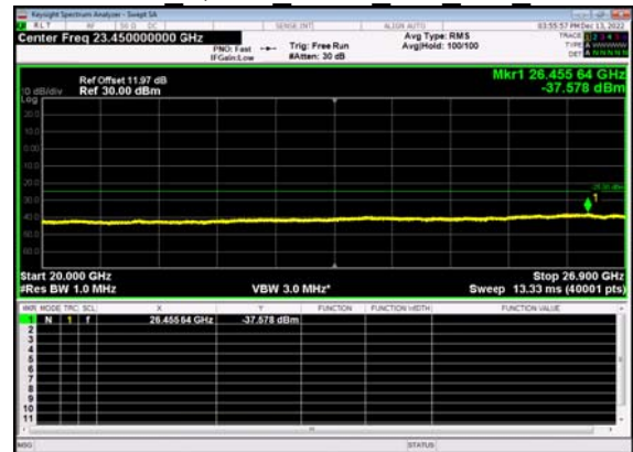
N41(10M)_DFT-s- OFDM QPSK Outer Full Mid CH
