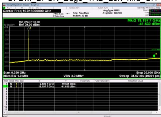
N41(10M)_DFT-s- OFDM BPSK Edge 1RB Left Mid CH
