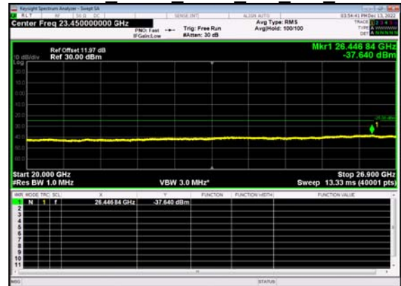
N41(10M)_DFT-s- OFDM BPSK Outer Full Mid CH
