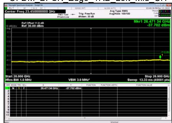
N41(10M)_DFT-s- OFDM BPSK Edge 1RB Left Mid CH
