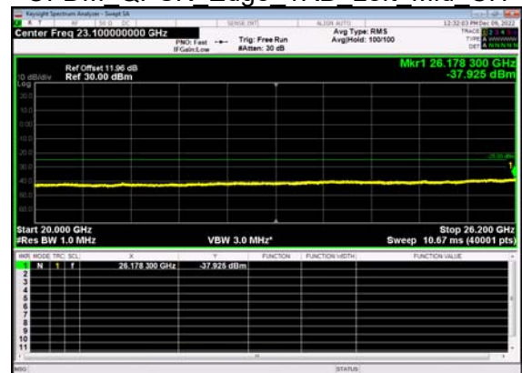
N38(40M)_DFT-s- OFDM QPSK Edge 1RB Left Mid CH
