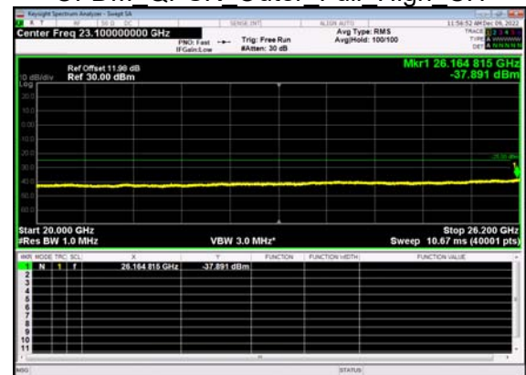
N38(15M)_DFT-s- OFDM QPSK Outer Full High CH
