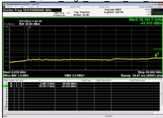
N41(10M)_DFT-s- OFDM QPSK Edge 1RB Left Low CH
