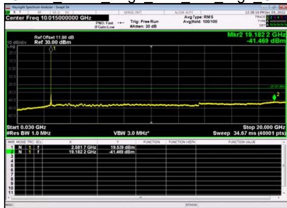
N38(40M)_DFT-s- OFDM BPSK Edge 1RB Left High CH
