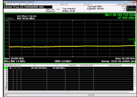
N38(40M)_DFT-s- OFDM BPSK Outer Full High CH
