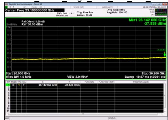
N38(20M)_DFT-s- OFDM BPSK Edge 1RB Left Mid CH
