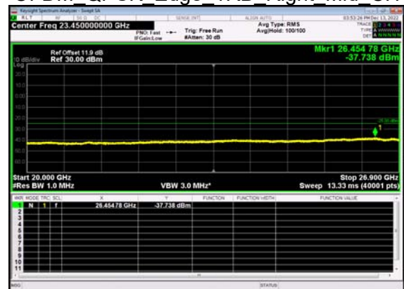
N41(10M)_DFT-s- OFDM QPSK Edge 1RB Right Mid CH
