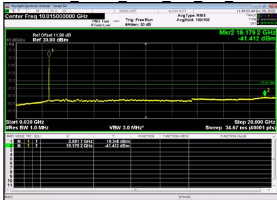
N38(15M)_DFT-s- OFDM QPSK Outer Full Mid CH
