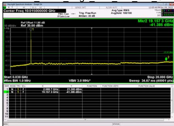
N38(20M)_DFT-s- OFDM BPSK Edge 1RB Left Mid CH
