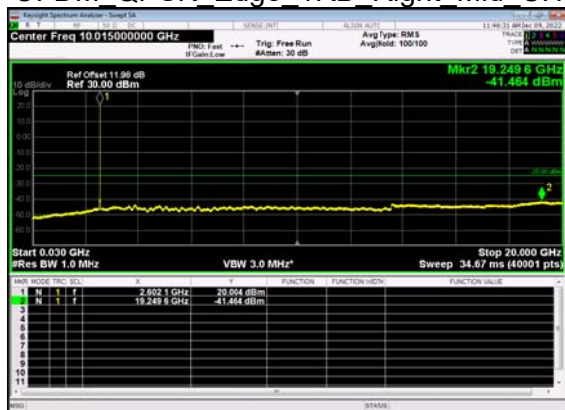
N38(15M)_DFT-s- OFDM QPSK Edge 1RB Right Mid CH
