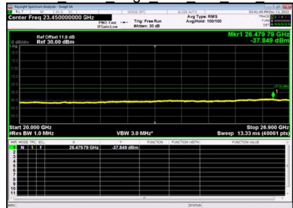
N41(10M)_DFT-s- OFDM BPSK Edge 1RB Left Low CH
