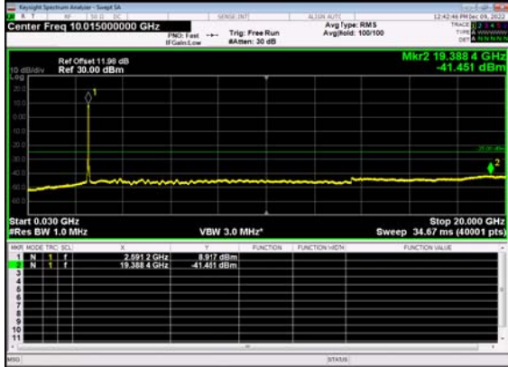
N38(40M)_DFT-s- OFDM BPSK Outer Full High CH
