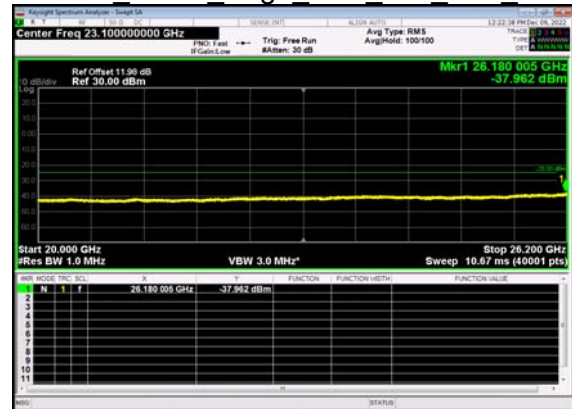
N38(40M)_DFT-s- OFDM BPSK Edge 1RB Left Low CH
