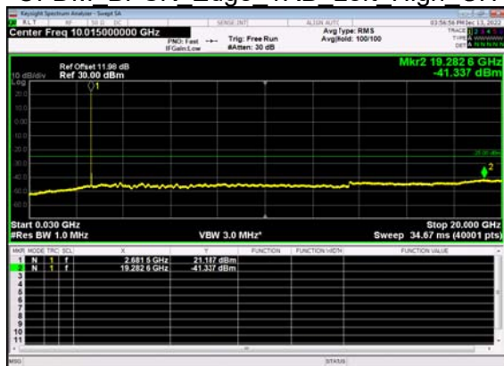
N41(10M)_DFT-s- OFDM BPSK Edge 1RB Left High CH
