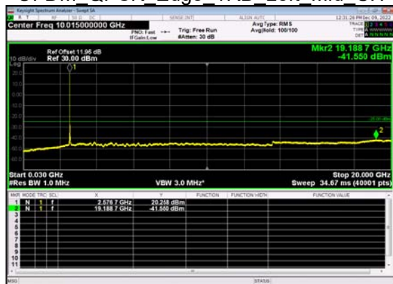
N38(40M)_DFT-s- OFDM QPSK Edge 1RB Left Mid CH
