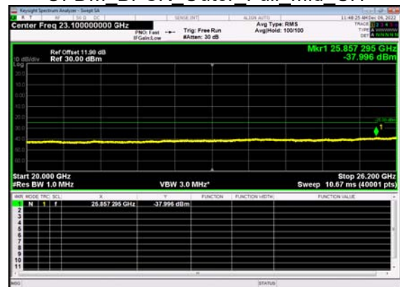
N38(15M)_DFT-s- OFDM BPSK Outer Full Mid CH
