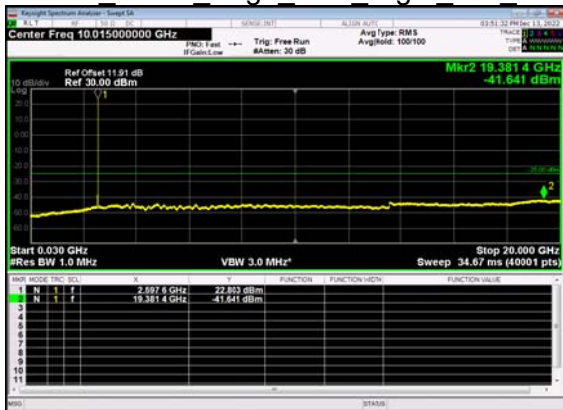
N41(10M)_DFT-s- OFDM BPSK Edge 1RB Right Mid CH
