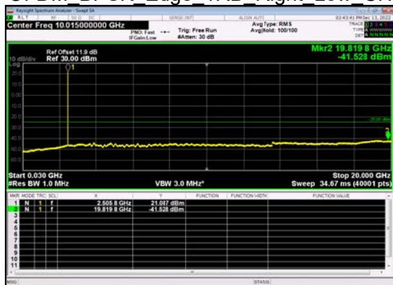
N41(10M)_DFT-s- OFDM BPSK Edge 1RB Right Low CH
