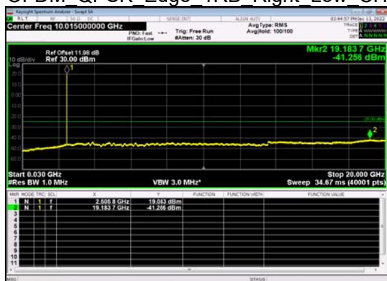
N41(10M)_DFT-s- OFDM QPSK Edge 1RB Right Low CH
