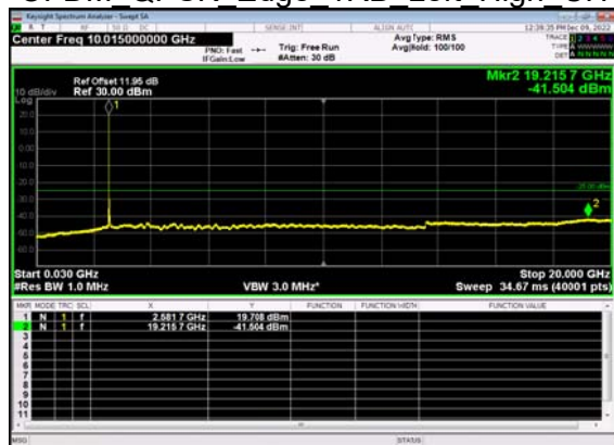
N38(40M)_DFT-s- OFDM QPSK Edge 1RB Left High CH
