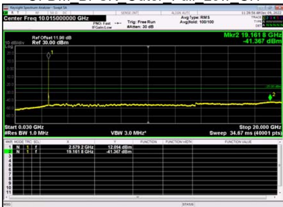
N38(15M)_DFT-s- OFDM BPSK Outer Full Low CH
