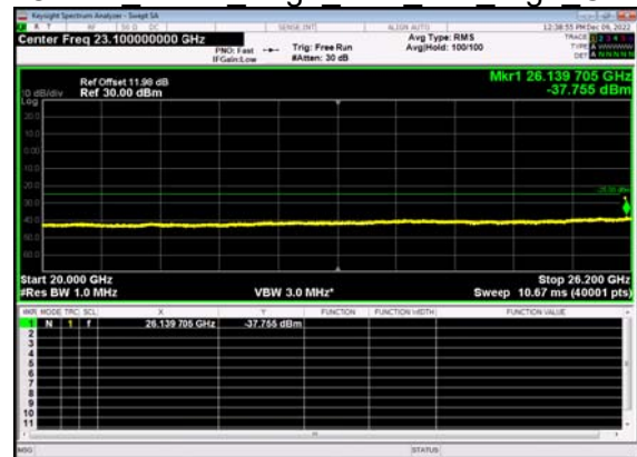
N38(40M)_DFT-s- OFDM BPSK Edge 1RB Left High CH
