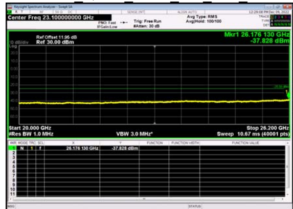
N38(40M)_DFT-s- OFDM QPSK Outer Full Low CH
