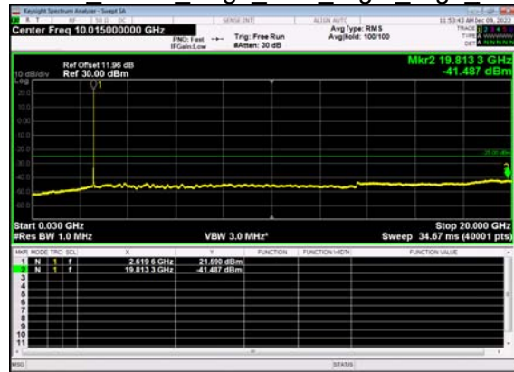
N38(15M)_DFT-s- OFDM QPSK Edge 1RB Right High CH
