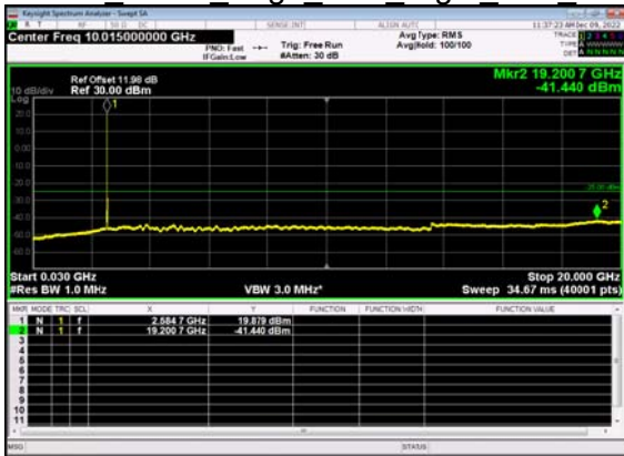
N38(15M)_DFT-s- OFDM BPSK Edge 1RB Right Low CH
