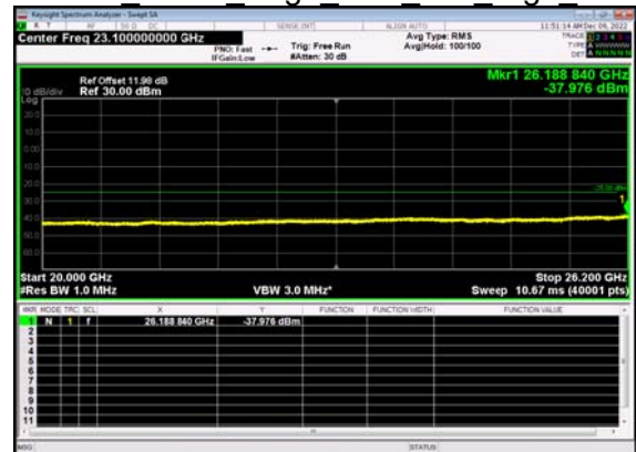
N38(15M)_DFT-s- OFDM BPSK Edge 1RB Left High CH
