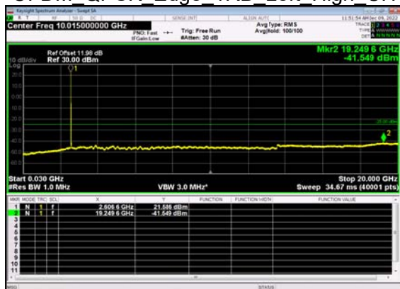
N38(15M)_DFT-s- OFDM QPSK Edge 1RB Left High CH
