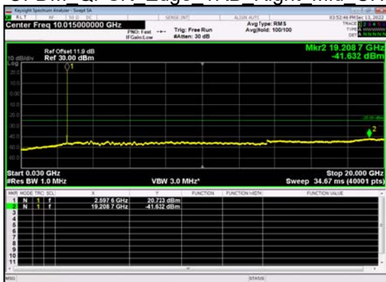
N41(10M)_DFT-s- OFDM QPSK Edge 1RB Right Mid CH
