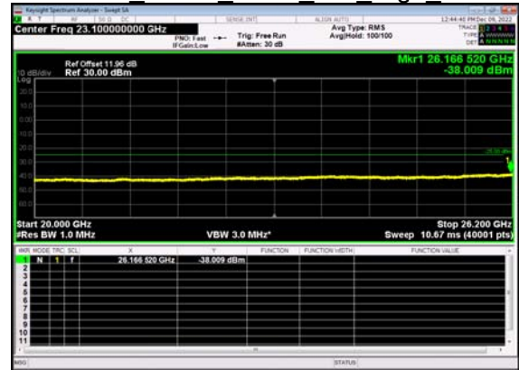
N38(40M)_DFT-s- OFDM QPSK Outer Full High CH
