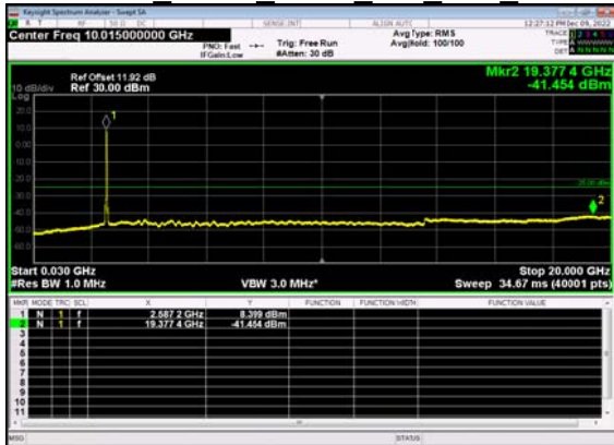
N38(40M)_DFT-s- OFDM BPSK Outer Full Low CH
