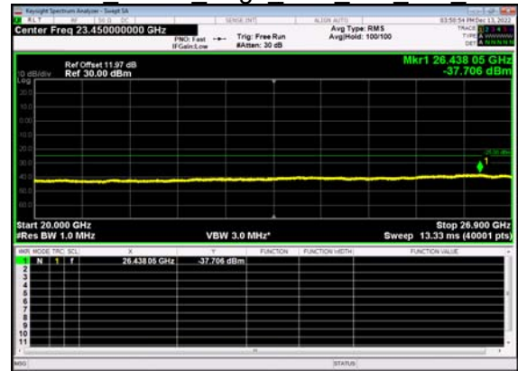
N41(10M)_DFT-s- OFDM QPSK Edge 1RB Left Mid CH
