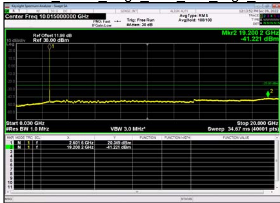
N38(20M)_DFT-s- OFDM BPSK Edge 1RB Left High CH
