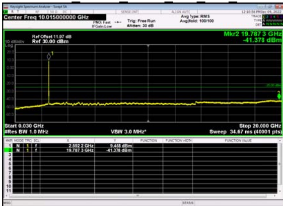
N38(20M)_DFT-s- OFDM BPSK Outer Full Mid CH
