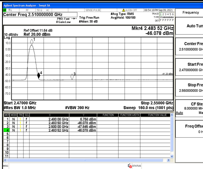
2DH5_Ant3_High_2480_Peak
