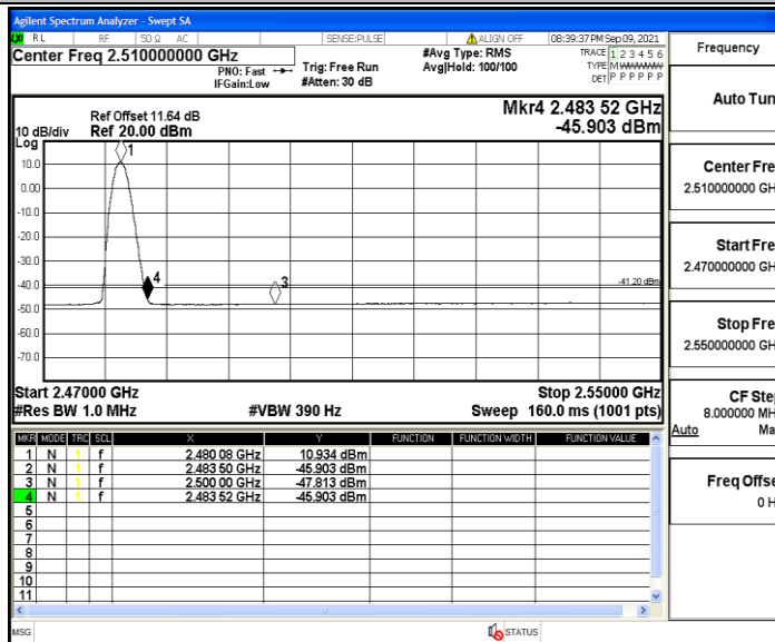
DH5_Ant3_High_2480_Peak
