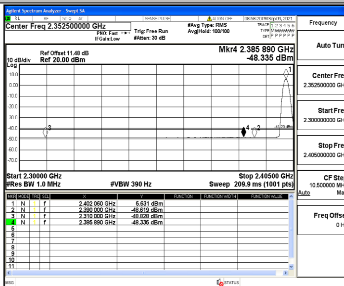
3DH5_Ant3_Low_2402_Peak
