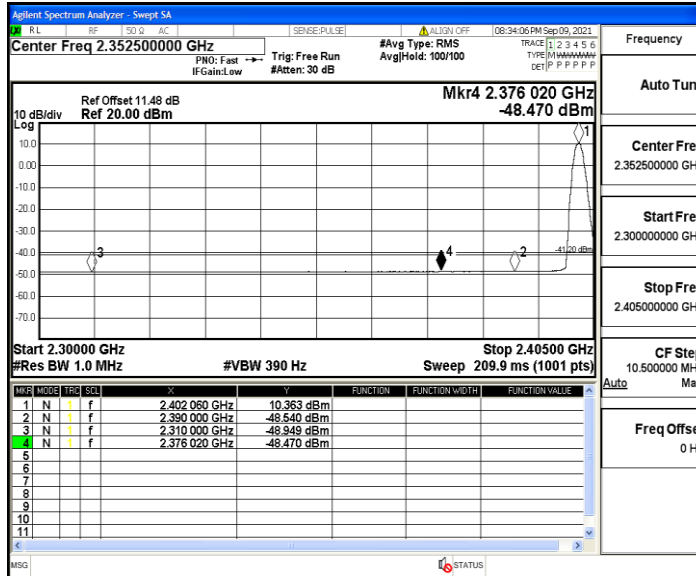
DH5_Ant3_Low_2402_Peak
