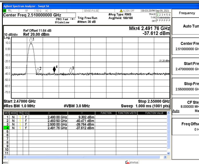
3DH5_Ant3_High_2480_Peak
