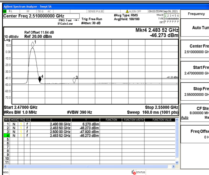
3DH5_Ant3_High_2480_Peak
