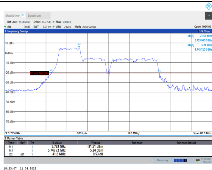
11AX40 Ant9 5755 242Tone RU61
