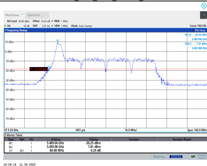
11AX80 Ant9 5530 106Tone RU53
