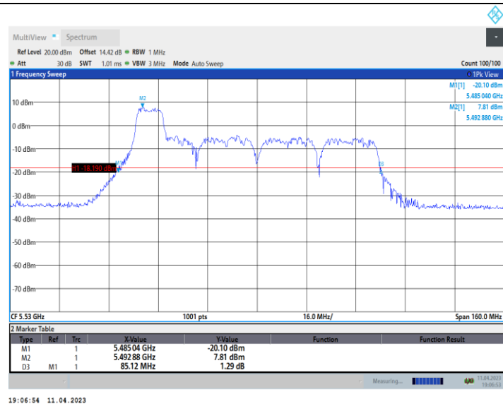
11AX80 Ant9 5530 242Tone RU61
