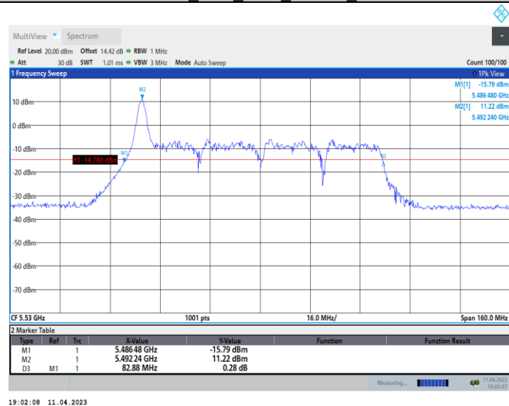
11AX80 Ant9 5530 52Tone RU37
