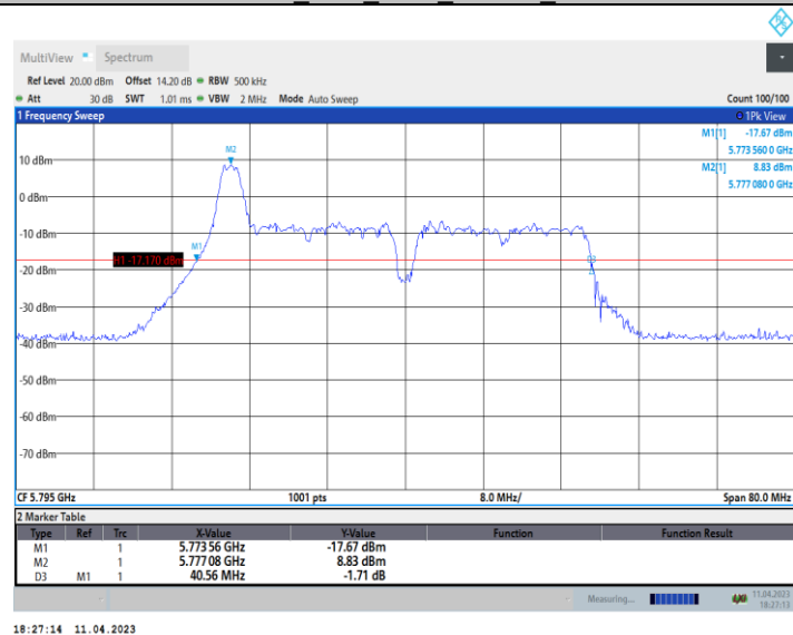
11AX40 Ant9 5795 52Tone RU37
