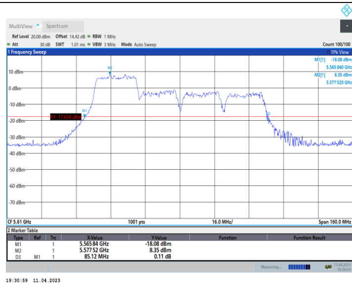
11AX80 Ant9 5610 484Tone RU65
