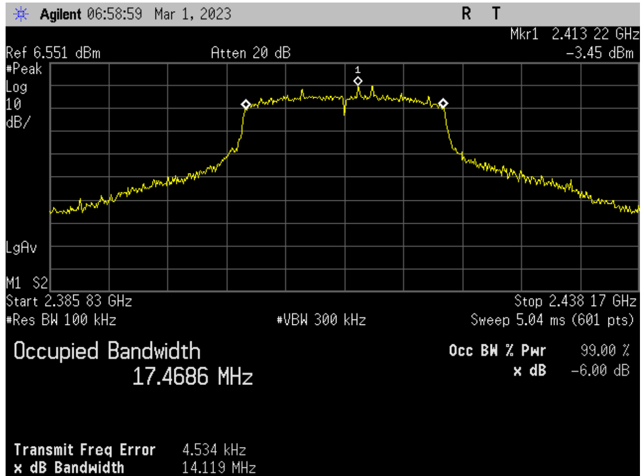
Figure 21: WIFI_Low Ch_2412MHz_20MHz BW_n-mode_Occupied Bandwidth_-6dB_Port 1.
