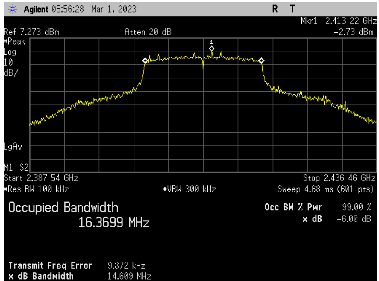
Figure 19: WIFI_Low Ch_2412MHz_20MHz BW_g-mode_Occupied Bandwidth_-6dB_Port 1.
