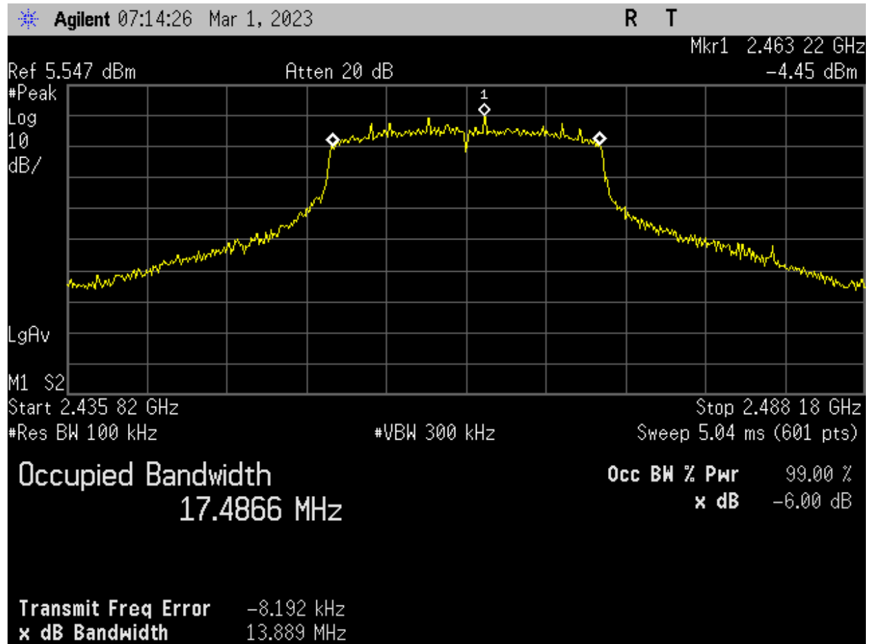
Figure 15: WIFI_High Ch_2462MHz_20MHz BW_n-mode_Occupied Bandwidth_-6dB_Port 1.
