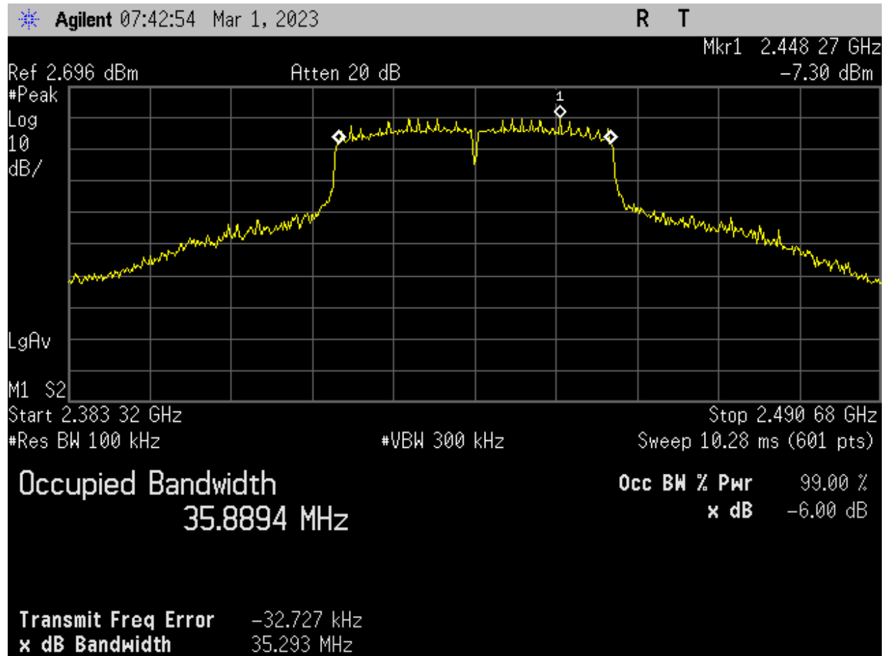
Figure 31: WIFI_Mid Ch_2437MHz_40MHz BW_n-mode_Occupied Bandwidth_-6dB_Port 1.
