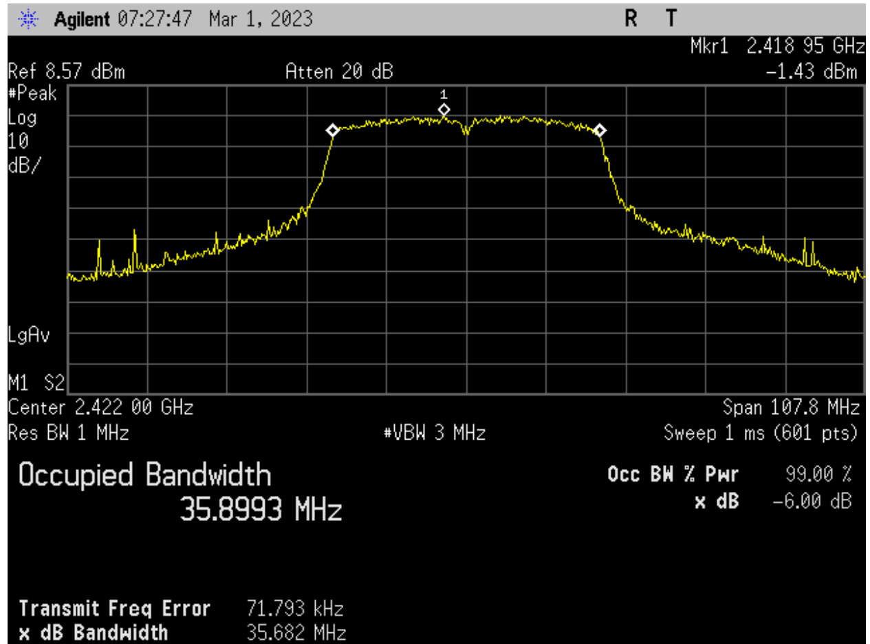
Figure 24: WIFI_Low Ch_2422MHz_40MHz BW_n-mode_Occupied Bandwidth_99 percent_Port 1.
