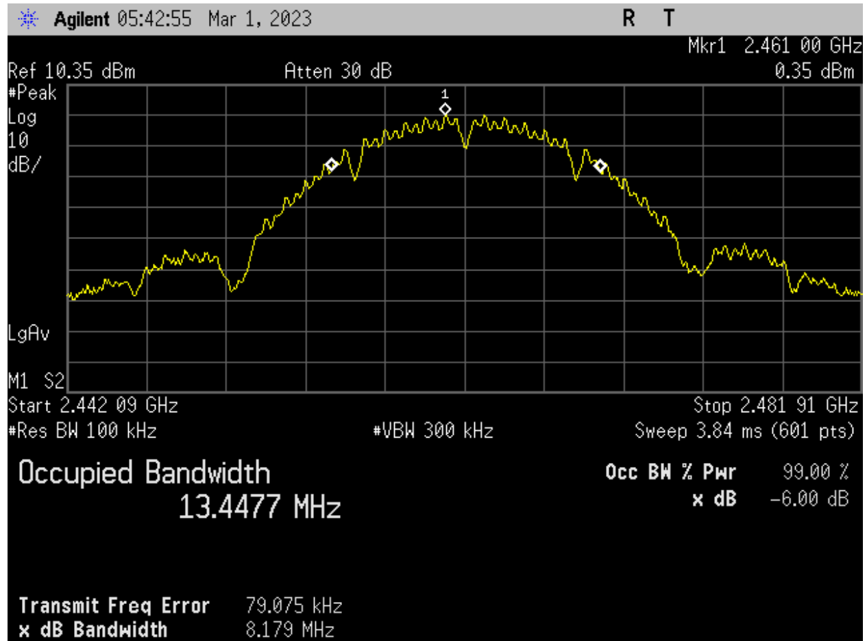
Figure 11: WIFI_High Ch_2462MHz_20MHz BW_b-mode_Occupied Bandwidth_-6dB_Port 1.
