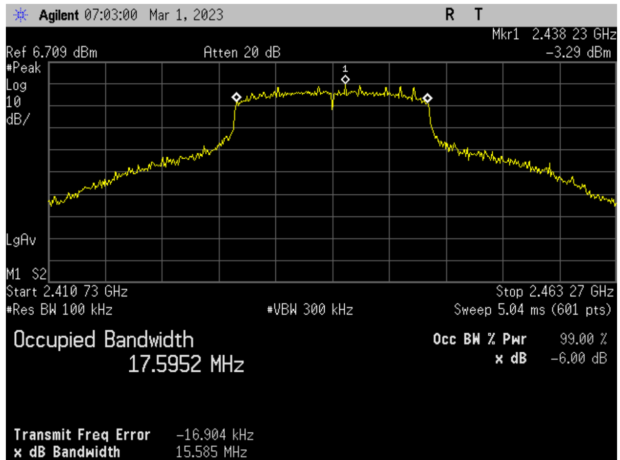
Figure 29: WIFI_Mid Ch_2437MHz_20MHz BW_n-mode_Occupied Bandwidth_-6dB_Port 1.
