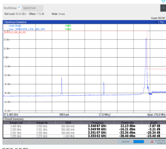
1-N78-3450-3550--30-90-H-5-CP-QPSK-Edge_1RB_R ight-1@244-Ant0-PASS-see graph
