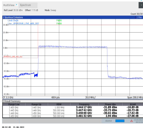
1-N78-3450-3550--30-100-L-3-DFT-PI2BPSK-Out er_Full-270@0-Ant0-PASS-see graph
