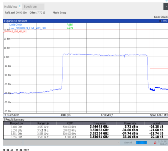
1-N78-3450-3550--30-90-H-3-DFT-PI2BPSK-Outer _Full-240@0-Ant0-PASS-see graph
