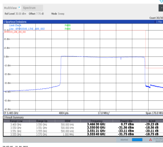
1-N78-3450-3550--30-90-H-6-CP-QPSK-Outer_Fu ll-245@0-Ant0-PASS-see graph
