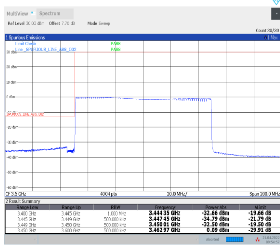
1-N78-3450-3550--30-100-L-6-CP-QPSK-Outer_F ull-273@0-Ant0-PASS-see graph
