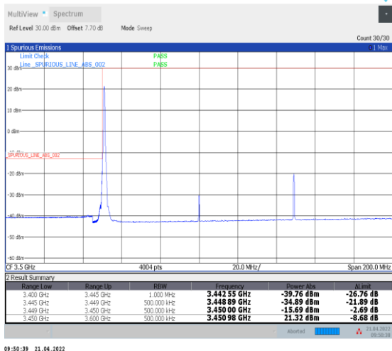
1-N78-3450-3550--30-100-L-1-DFT-PI2BPSK-Edge_1 RB_Left-1@0-Ant0-PASS-see graph
