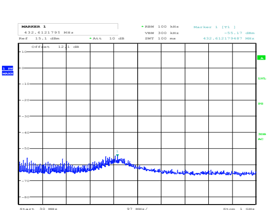
Figure 8.3-7: Conducted spurious emissions, Low channel
