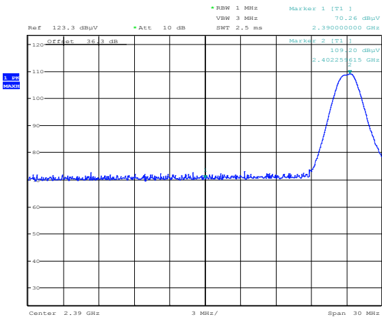
Figure 8.3-3: Conducted Band edge emission, low channel
