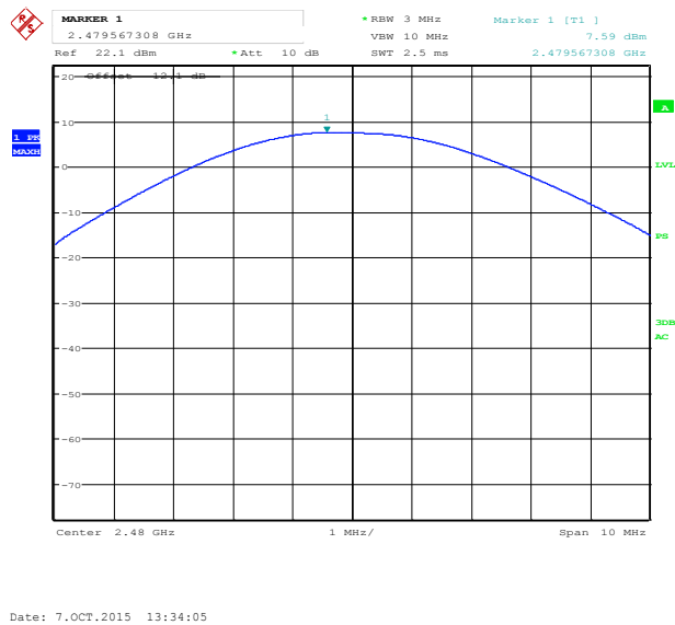
Figure 8.2-3: High Channel
