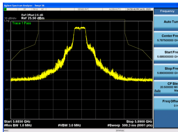
5785MHz with 2*2 CDD PK
