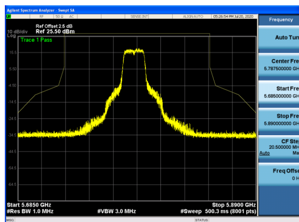
5785MHz with 4*4 Beamforming PK
