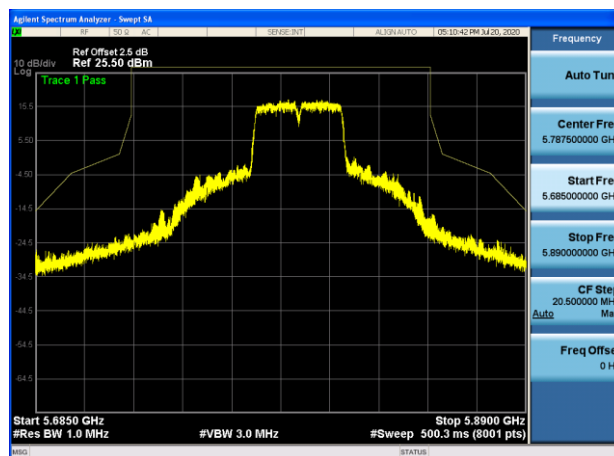
5795MHz with 2*2 Beamforming PK
