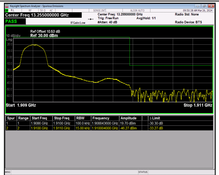
Band2_1.4MHz_QPSK_19193_1RB#0
