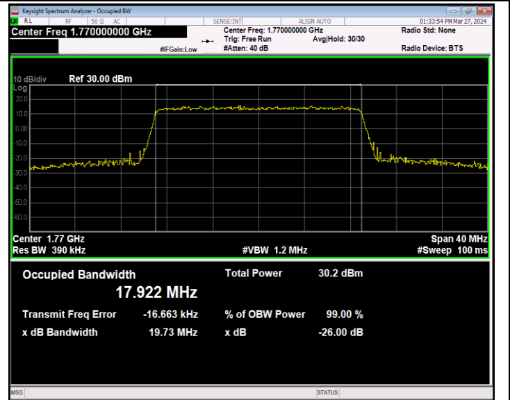
Band66-20MHz-64QAM-132572-100RB#0-PASS
