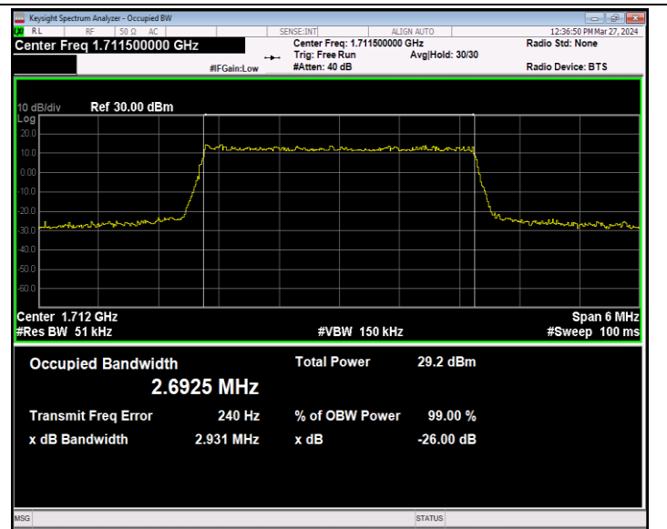
Band66-3MHz-64QAM-131987-15RB#0-PASS
