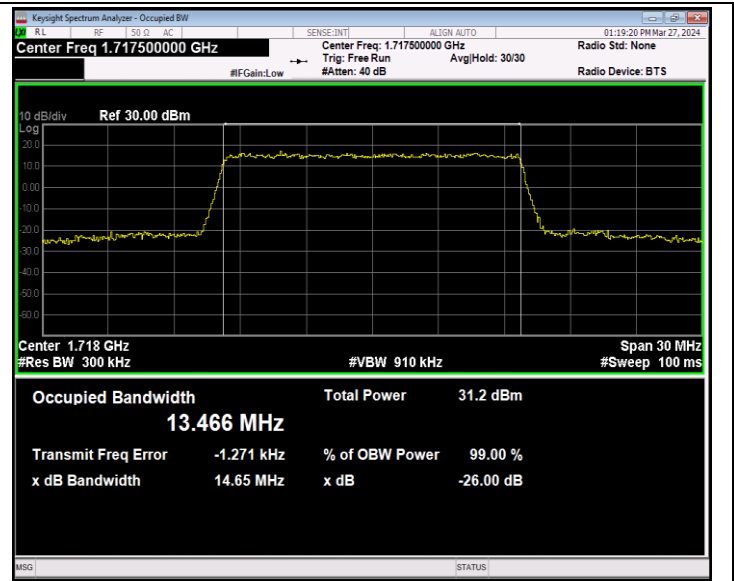
Band66-15MHz-16QAM-132047-75RB#0-PASS
