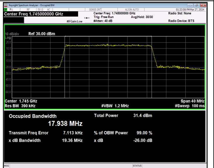
Band66-20MHz-16QAM-132322-100RB#0-PASS
