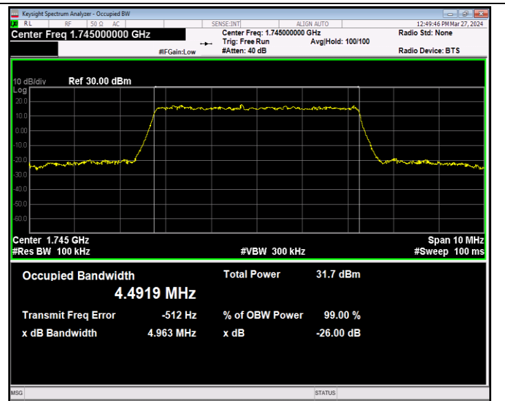
Band66-5MHz-QPSK-132322-25RB#0-PASS
