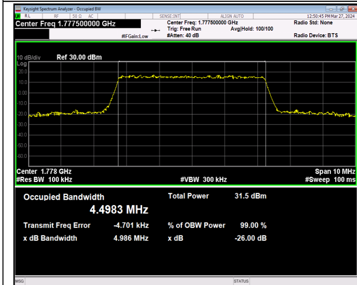
Band66-5MHz-QPSK-132647-25RB#0-PASS
