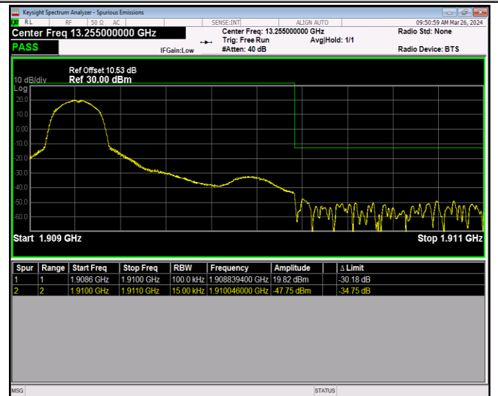
Band2_1.4MHz_64QAM_19193_1RB#0
