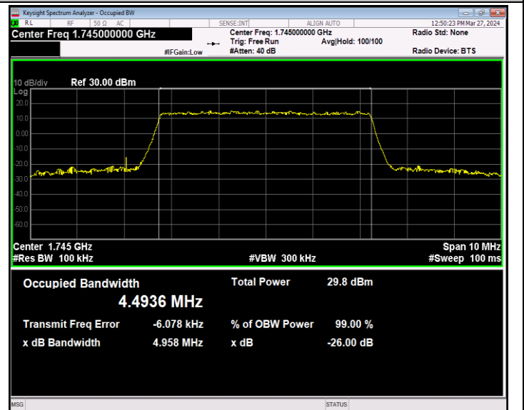
Band66-5MHz-16QAM-132322-25RB#0-PASS
