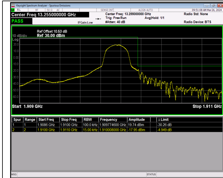
Band2_1.4MHz_QPSK_19193_1RB#5
