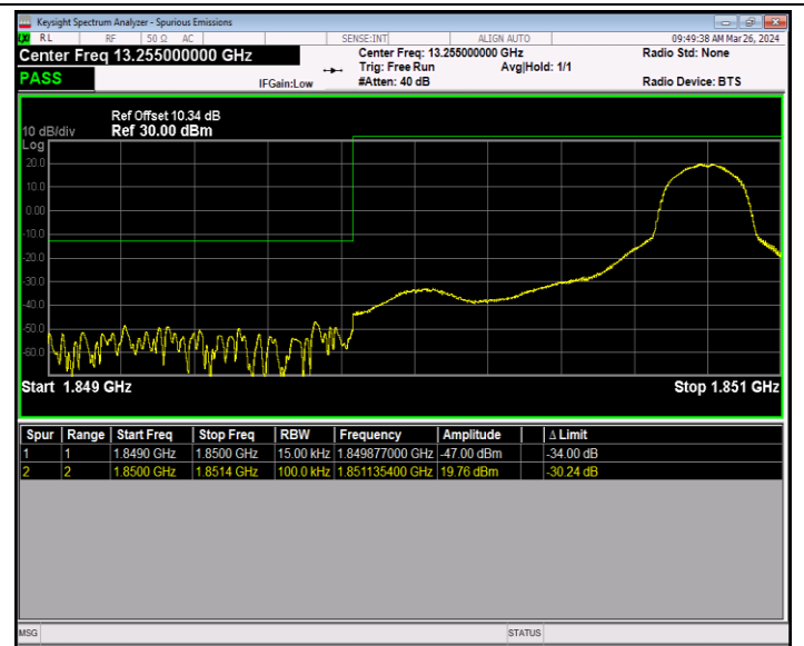
Band2_1.4MHz_QPSK_18607_1RB#5
