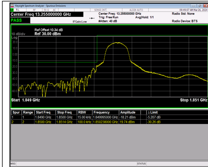
Band2_1.4MHz_QPSK_18607_1RB#0
