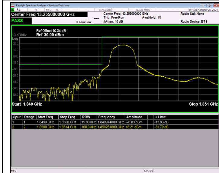
Band2_1.4MHz_16QAM_18607_1RB#0
