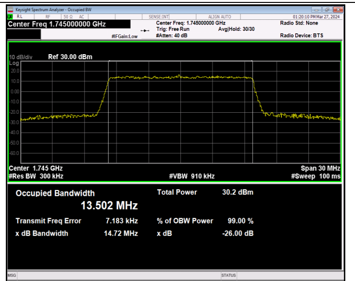
Band66-15MHz-64QAM-132322-75RB#0-PASS
