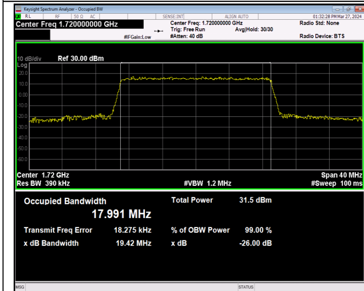
Band66-20MHz-16QAM-132072-100RB#0-PASS
