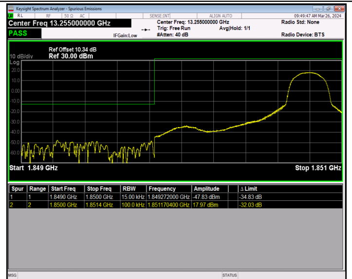
Band2_1.4MHz_16QAM_18607_1RB#5
