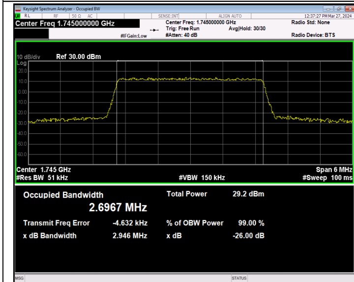
Band66-3MHz-64QAM-132322-15RB#0-PASS
