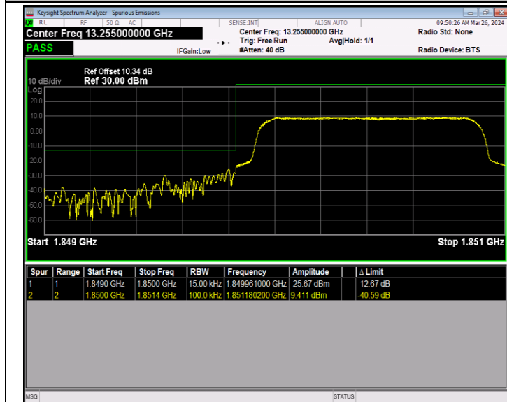
Band2_1.4MHz_64QAM_18607_6RB#0
