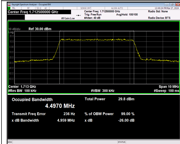
Band66-5MHz-16QAM-131997-25RB#0-PASS
