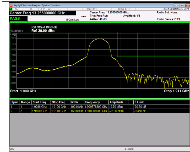
Band2_1.4MHz_64QAM_19193_1RB#5
