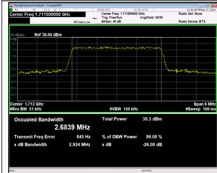
Band66-3MHz-16QAM-131987-15RB#0-PASS
