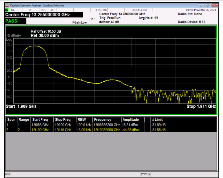
Band2_1.4MHz_16QAM_19193_1RB#0
