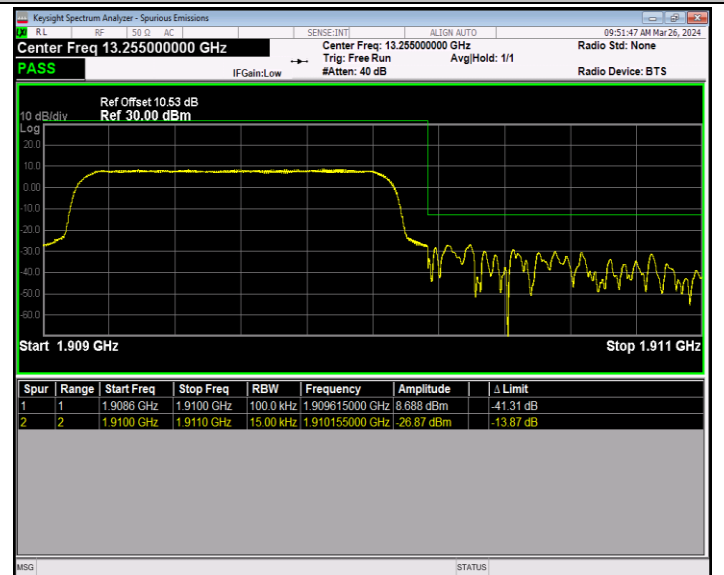
Band2_1.4MHz_16QAM_19193_6RB#0
