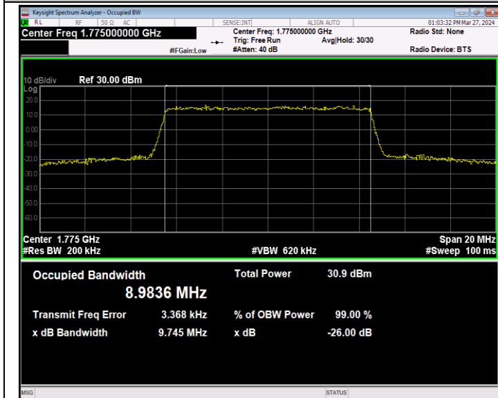
Band66-10MHz-16QAM-132622-50RB#0-PASS
