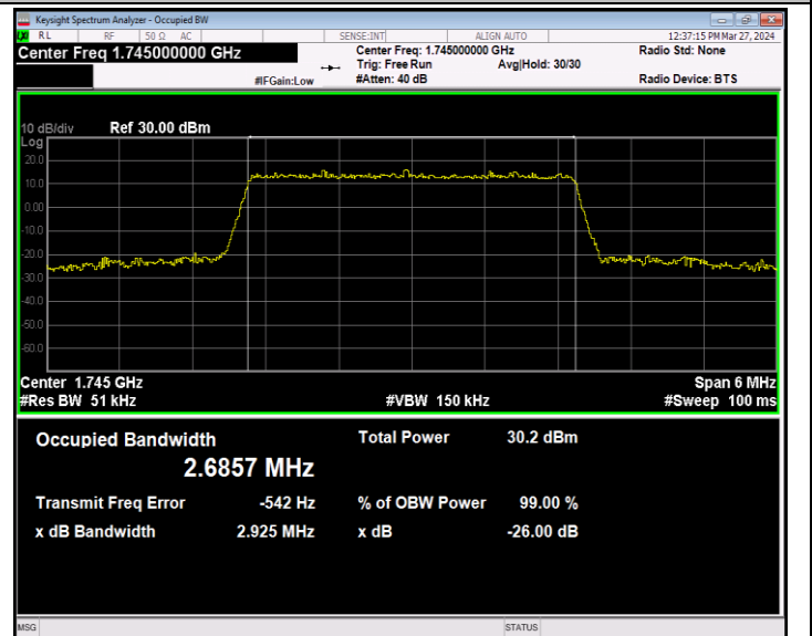
Band66-3MHz-16QAM-132322-15RB#0-PASS
