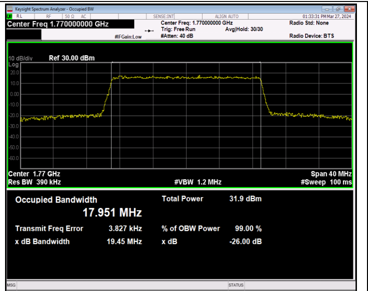
Band66-20MHz-QPSK-132572-100RB#0-PASS
