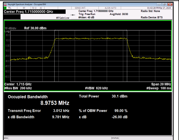
Band66-10MHz-64QAM-132022-50RB#0-PASS
