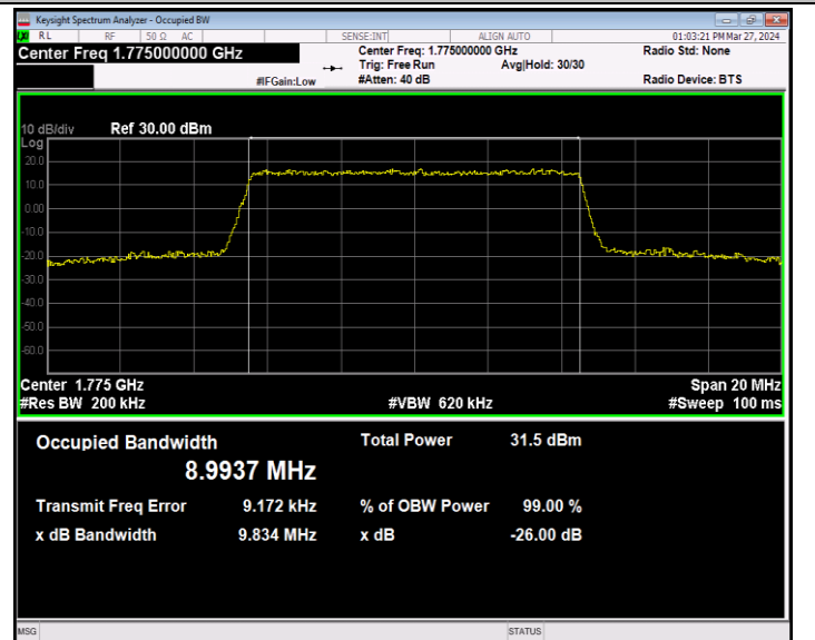
Band66-10MHz-QPSK-132622-50RB#0-PASS
