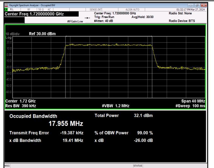
Band66-20MHz-QPSK-132072-100RB#0-PASS
