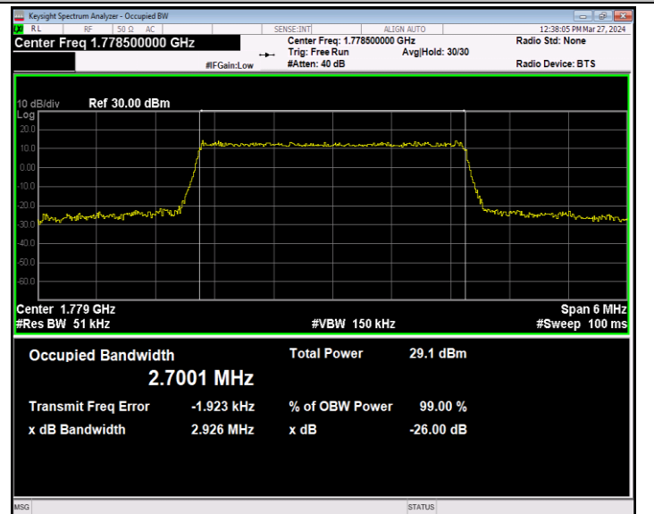
Band66-3MHz-64QAM-132657-15RB#0-PASS
