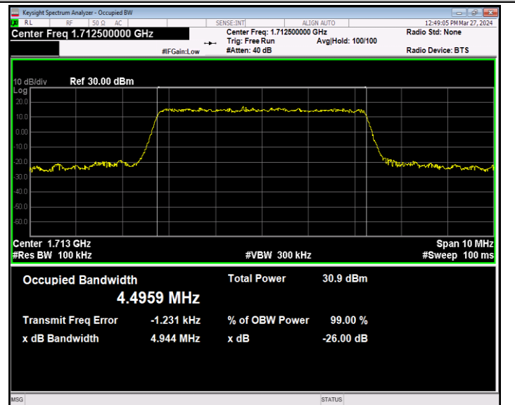
Band66-5MHz-16QAM-131997-25RB#0-PASS
