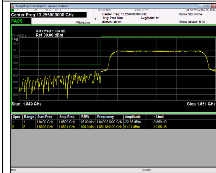
Band2_1.4MHz_QPSK_18607_6RB#0
