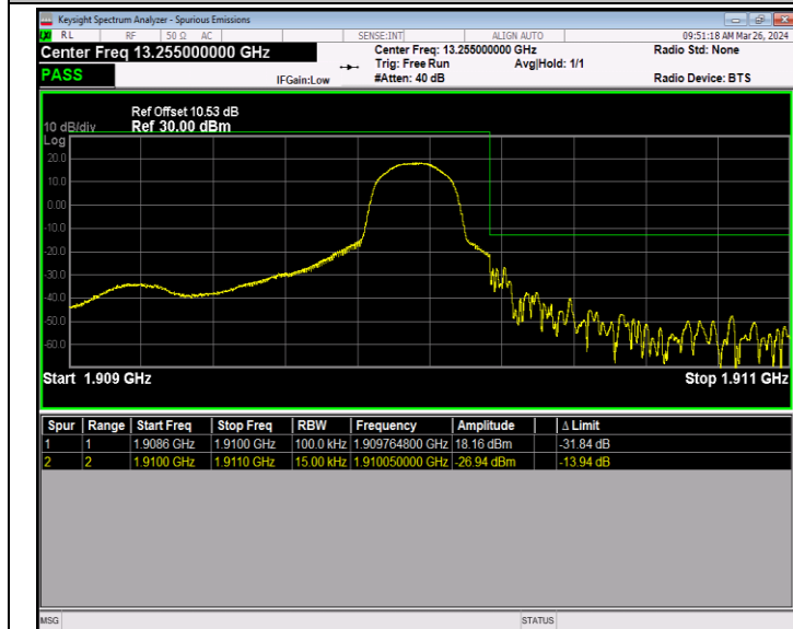
Band2_1.4MHz_16QAM_19193_1RB#5
