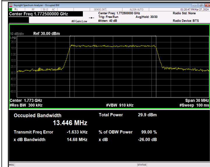
Band66-15MHz-64QAM-132597-75RB#0-PASS
