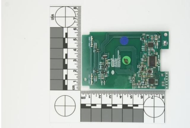
PCBA Top View
