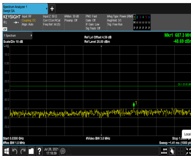
Band66-1.4MHz-QPSK-131979:30~1000MHz
