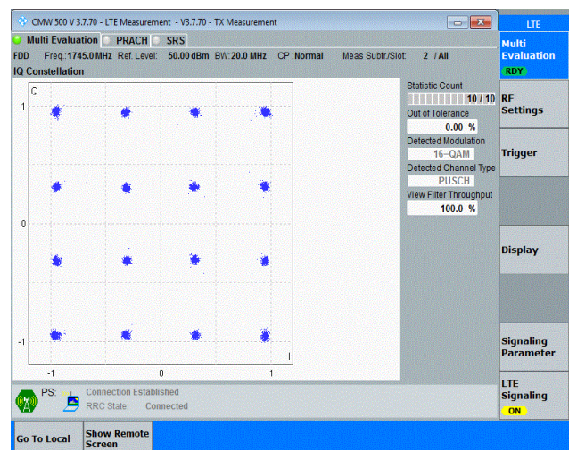
Band66-20MHz-16QAM-132322-100RB#0
