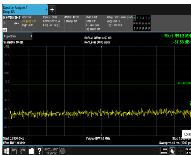
Band66-1.4MHz-QPSK-132322:30~1000MHz
