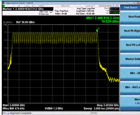
280k Number of hopping Frequencies = 43
