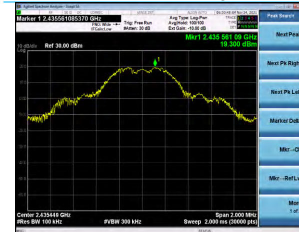
500k Reference Level – Mid Ch
