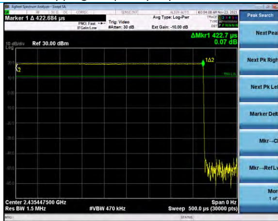
500k dwell time = 423 μs
