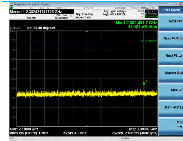
280k Low Ch 2310-2390 MHz Peak
