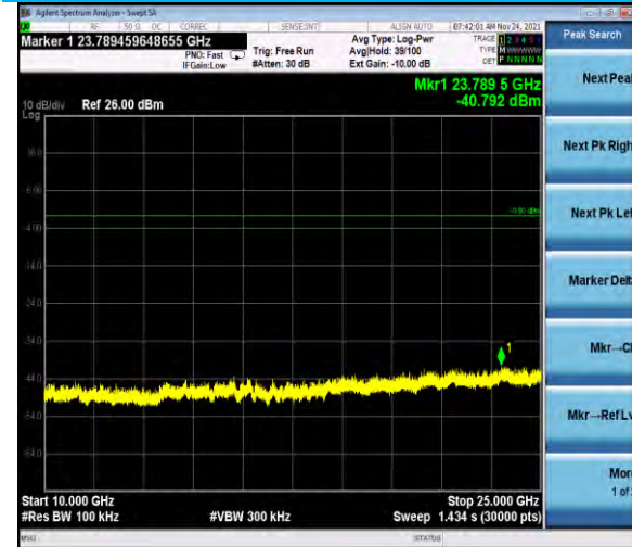
280k – High Ch – Spurious
