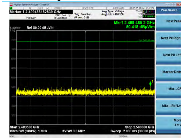
500k High Ch 2483.5-2500 MHz Peak
