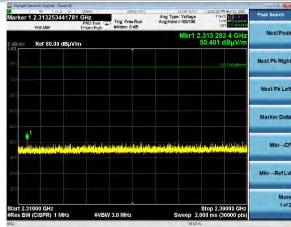
500k Hopping 2310-2390 MHz Peak
