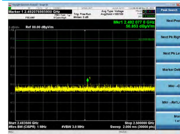
280k High Ch 2483.5-2500 MHz Peak
