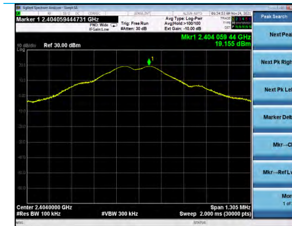
280k Reference Level – Low Ch
