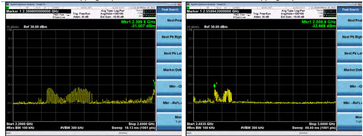
500k – Hopping – Spurious
