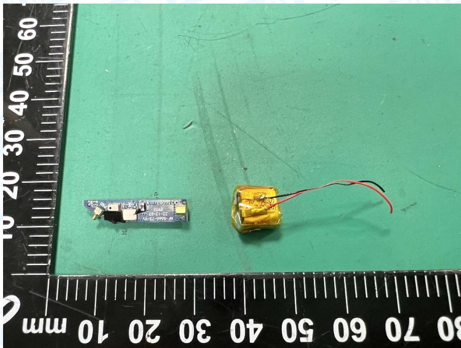
Photo 9 Appearance of PCB & Battery
