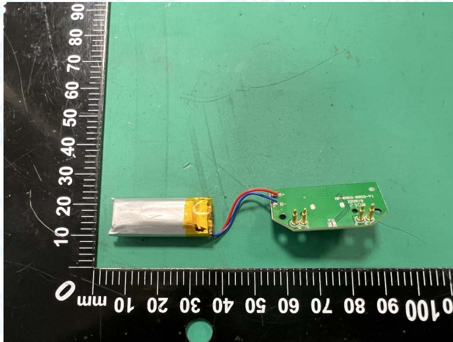
Photo 12 Appearance of PCB& Battery
