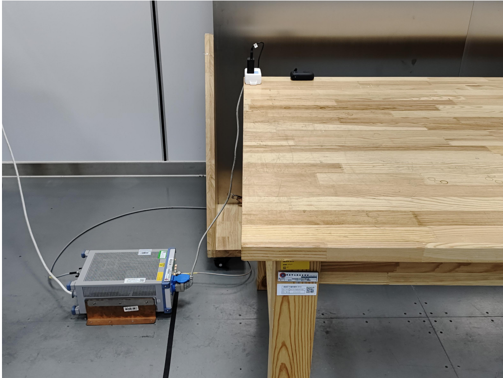
PART 15B AC power-line conducted emissions_150KHz-30MHz
