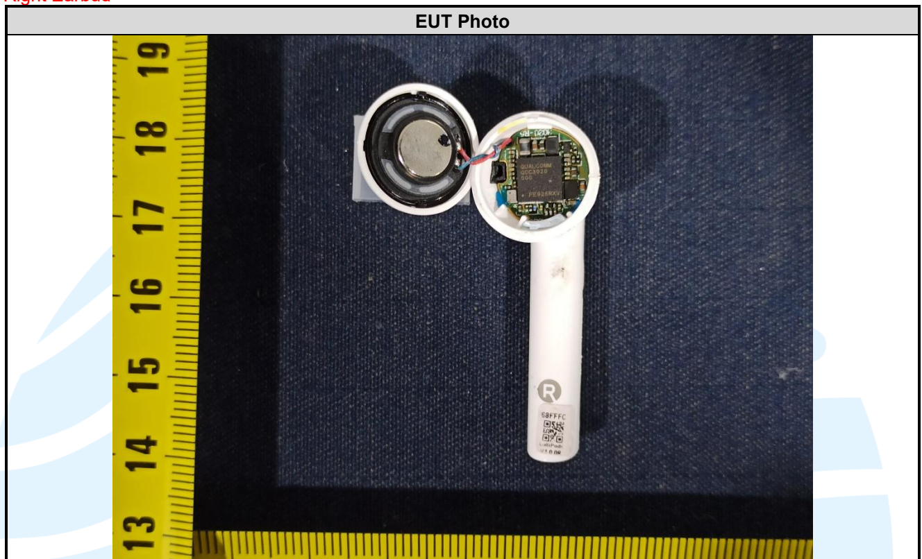
Right Earbud
