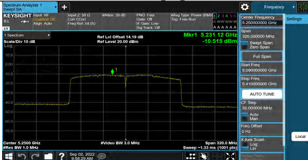
11AX160MIMO Ant3 5250
