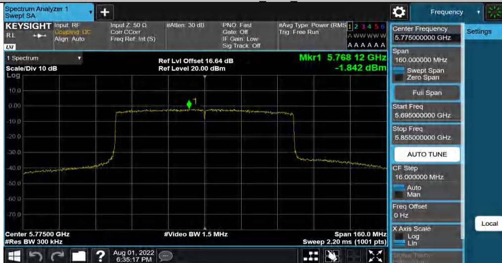
11AX80MIMO Ant2 5775
