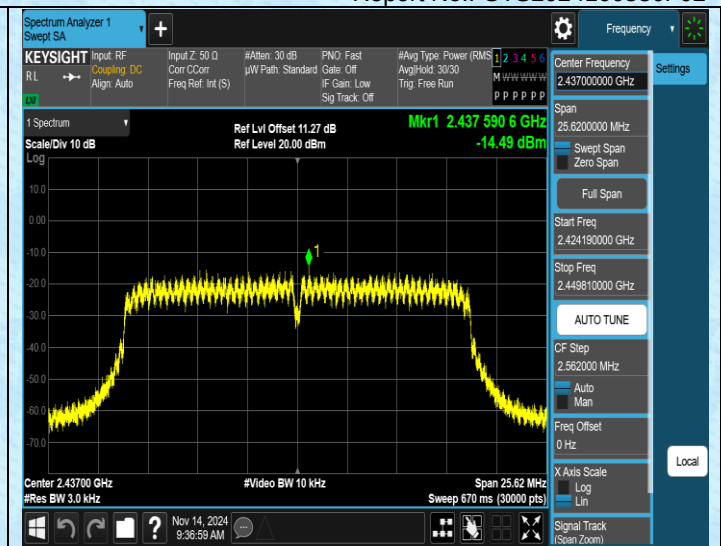
11N20SISO-Ant1-2437-PASS
