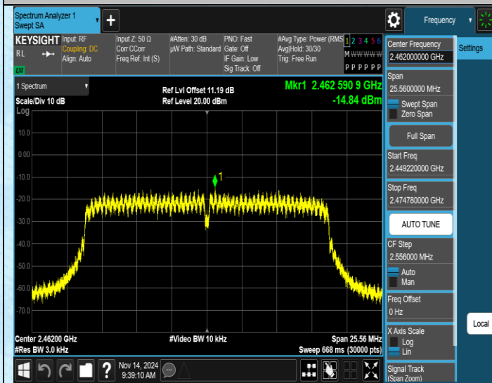
11N20SISO-Ant1-2462-PASS
