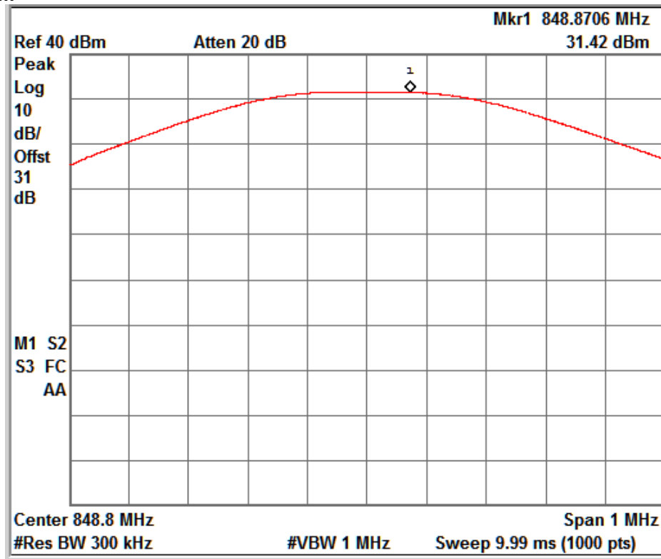
GSM_Voice_Channel No. 251
