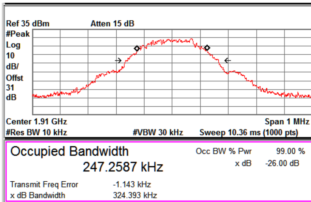
GSM_Voice_Channel No. 810
