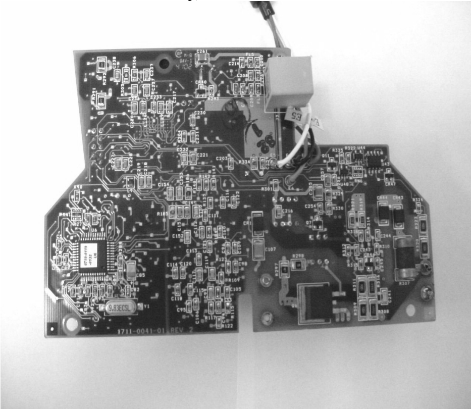
Printed Circuit Card Assembly, Bottom View
