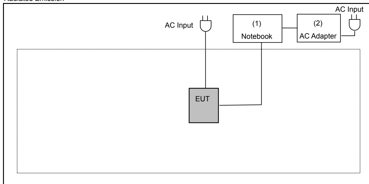
Radiated Emission
