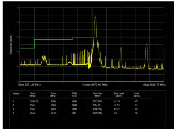
LTE Band 38 16QAM 15MHz CH-Low, 100%RB
