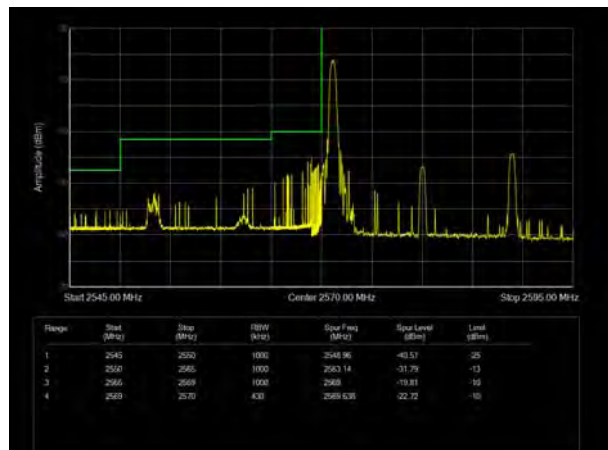
LTE Band 38 16QAM 20MHz CH-Low, 1 RB
