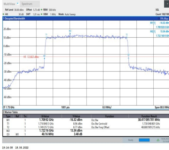
1-N66--15-40-L-6-CP-QPSK-Outer_Full-216@0-Ant1 -38.417-40.160-≤40-PASS
