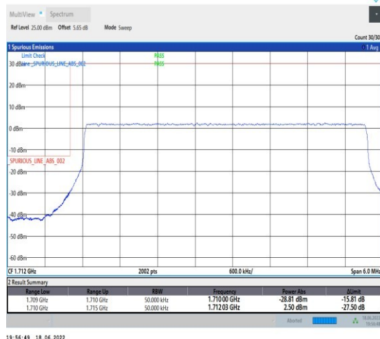
1-N66--15-5-L-6-CP-QPSK-Outer_Full-25@0-Ant1-seegraph-PASS-see graph
