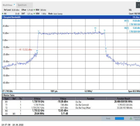
1-N66--15-30-M-6-CP-QPSK-Outer_Full-160@0-Ant 1-28.487-29.640-≤30-PASS
