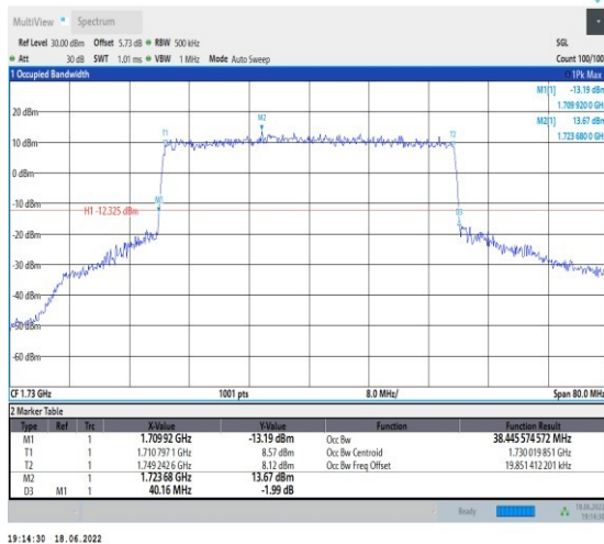
1-N66--15-40-L-8-CP-64QAM-Outer_Full-216@0-Ant t1-38.446-40.160-≤40-PASS
