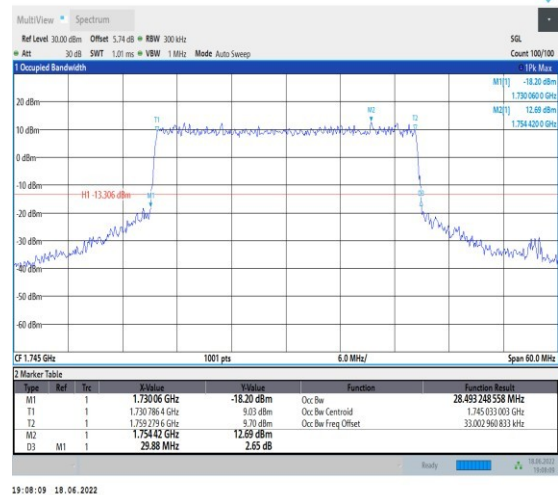
1-N66--15-30-M-7-CP-16QAM-Outer_Full-160@0-A nt1-28.493-29.880-≤30-PASS
