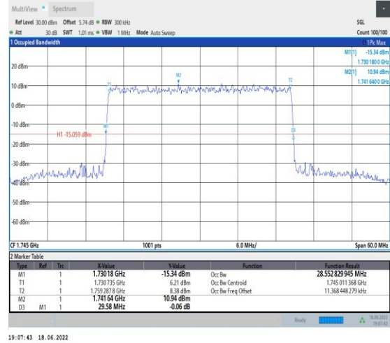
1-N66--15-30-M-5-DFT-256QAM-Outer_Full-160@0- Ant1-28.553-29.580-≤30-PASS
