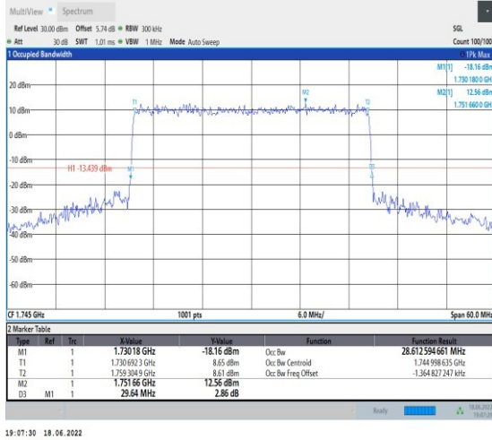
1-N66--15-30-M-4-DFT-64QAM-Outer_Full-160@0-A nt1-28.613-29.640-≤30-PASS
