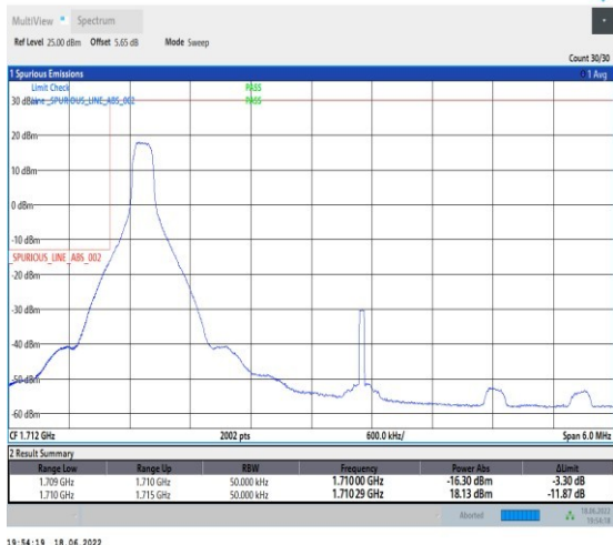
1-N66--15-5-L-1-DFT-PI2BPSK-Edge_1RB_Left-1@0-Ant1-seegraph-PASS-see graph
