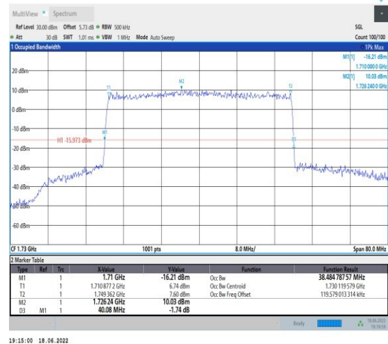
1-N66--15-40-L-9-CP-256QAM-Outer_Full-216@0-Ant1 nt1-38.485-40.080-≤40-PASS
