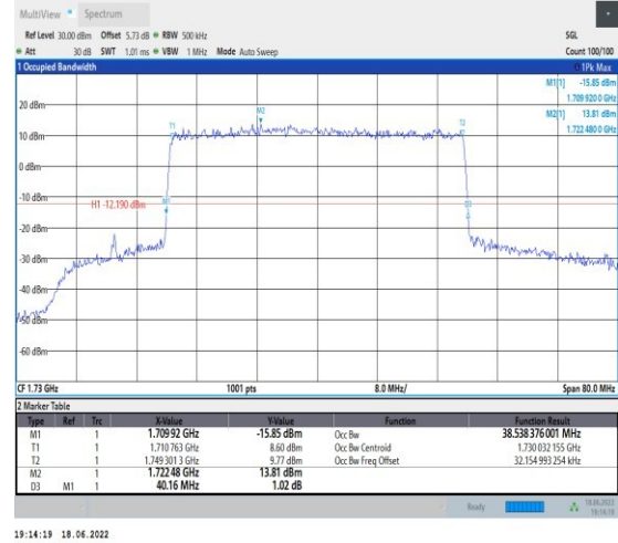
1-N66--15-40-L-7-CP-16QAM-Outer_Full-216@0-An t1-38.538-40.160-≤40-PASS
