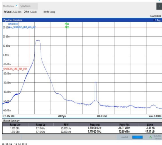
1-N66--15-5-L-4-CP-QPSK-Edge_1RB_Left-1@0-Ant1-seegraph-PASS-see graph
