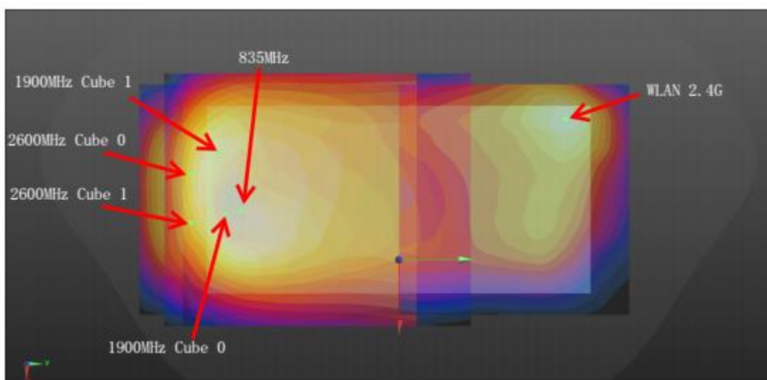
Back for WWAN+WWAN2.4GHz _5mm
