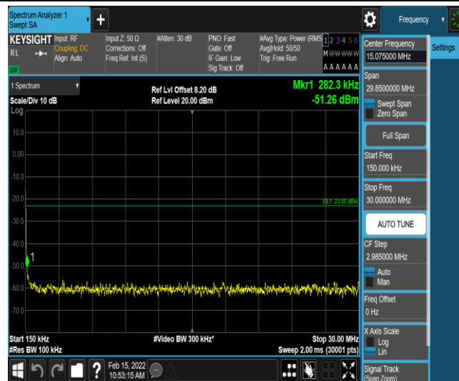
Band12-5MHz-QPSK-23095-1-0-Low-0.15-30--51.26-PASS
