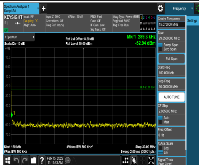
Band12-10MHz-QPSK-23130-1-0-High-0.15-30--52.94-PASS
