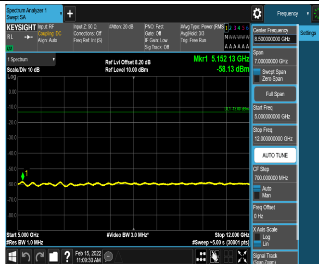
Band12-10MHz-QPSK-23095-1-0-Low-5000-12000--58.13-PASS
