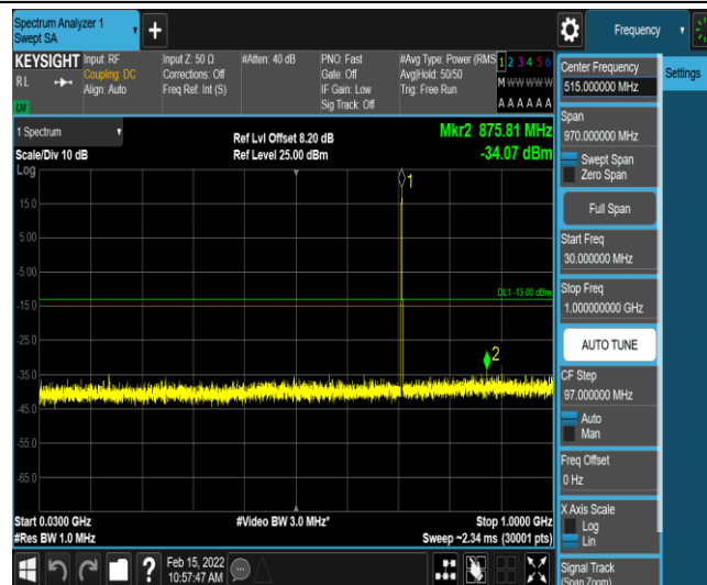
Band12-5MHz-16QAM-23155-1-0-High-30-1000--34.07-PASS
