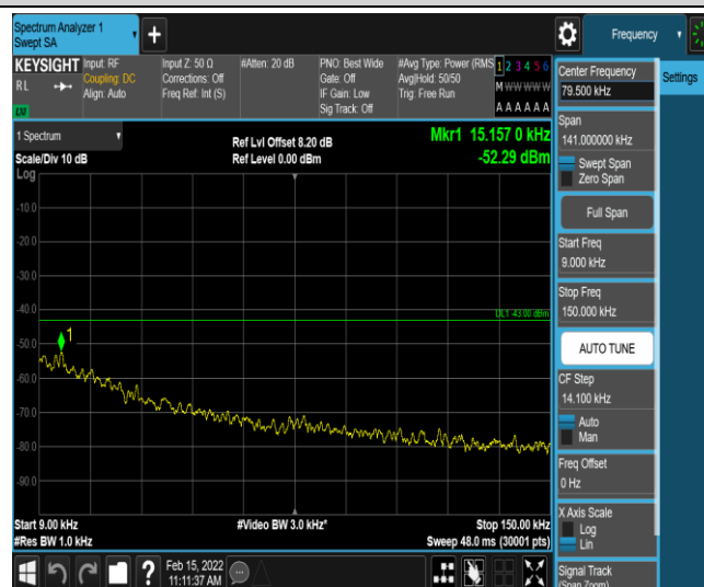
Band12-10MHz-QPSK-23130-1-0-High-0.009-0.15--52.3-PASS
