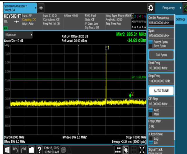
Band12-5MHz-QPSK-23155-1-0-High-30-1000--34.69-PASS
