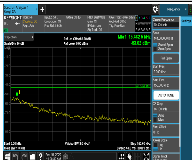
Band12-10MHz-QPSK-23095-1-0-Low-0.009-0.15--53.02-PASS
