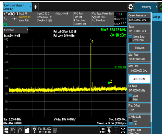
Band12-10MHz-QPSK-23095-1-0-Low-30-1000--34.18-PASS
