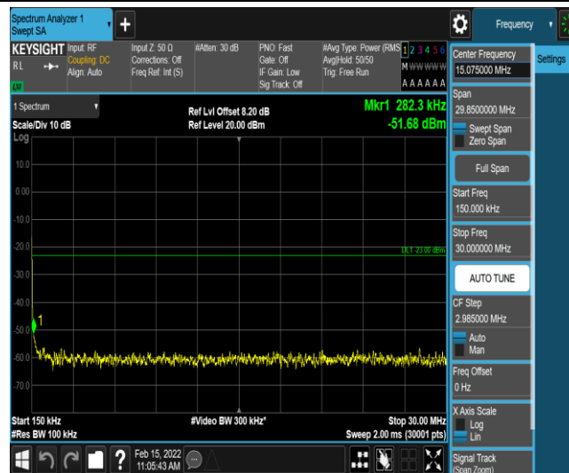
Band12-10MHz-QPSK-23060-1-0-Low-0.15-30--51.68-PASS
