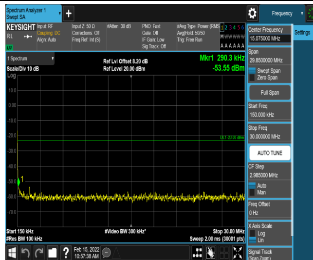
Band12-5MHz-16QAM-23155-1-0-High-0.15-30--53.55-PASS
