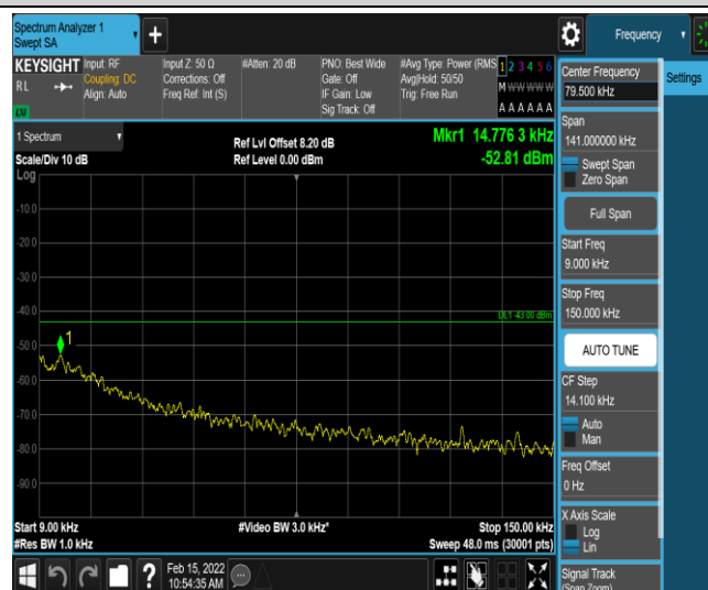
Band12-5MHz-16QAM-23095-1-0-Low-0.009-0.15--52.81-PASS
