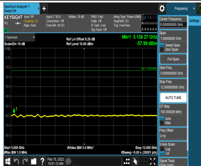
Band12-5MHz-QPSK-23035-1-0-Low-5000-12000--57.99-PASS
