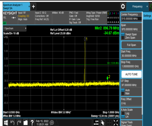
Band12-10MHz-QPSK-23060-1-0-Low-30-1000--34.67-PASS
