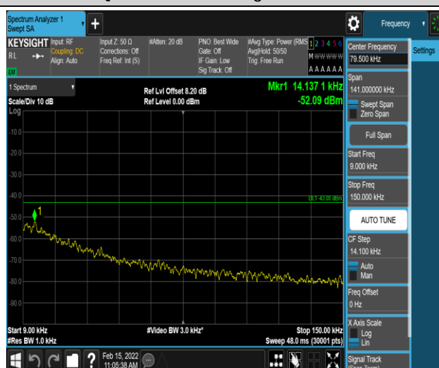
Band12-10MHz-QPSK-23060-1-0-Low-0.009-0.15--52.09-PASS
