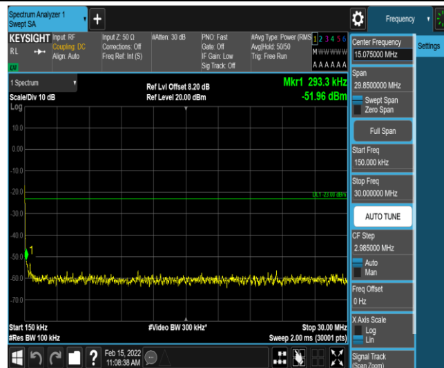
Band12-10MHz-QPSK-23095-1-0-Low-0.15-30--51.96-PASS
