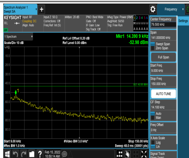
Band12-5MHz-QPSK-23035-1-0-Low-0.009-0.15--52.98-PASS
