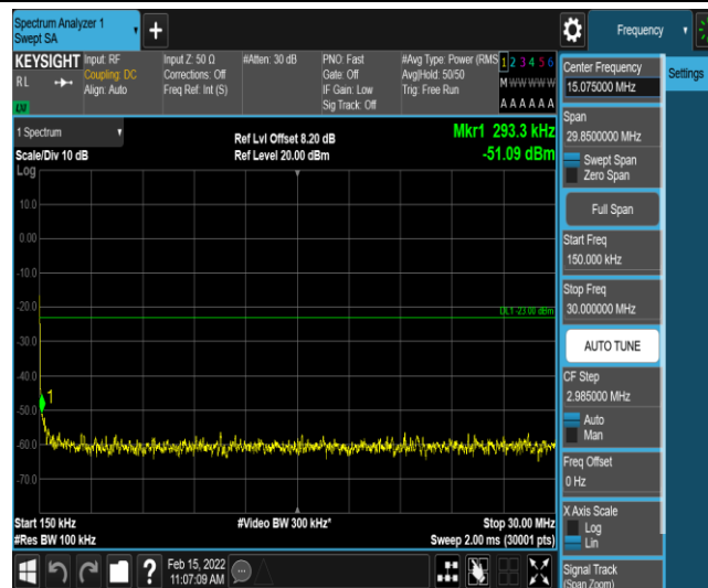
Band12-10MHz-16QAM-23060-1-0-Low-0.15-30--51.1-PASS
