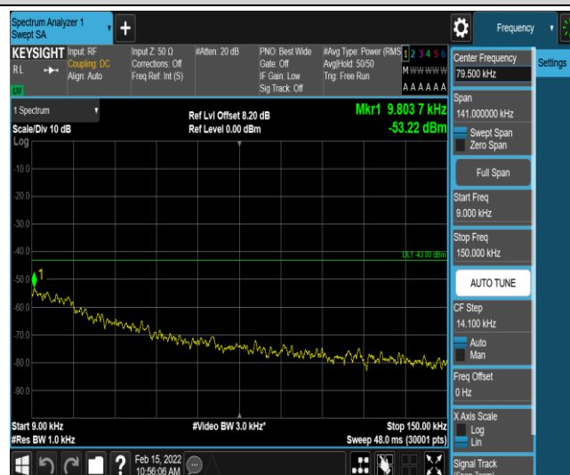
Band12-5MHz-QPSK-23155-1-0-High-0.009-0.15--53.22-PASS
