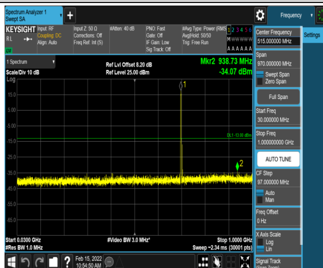
Band12-5MHz-16QAM-23095-1-0-Low-30-1000--34.08-PASS
