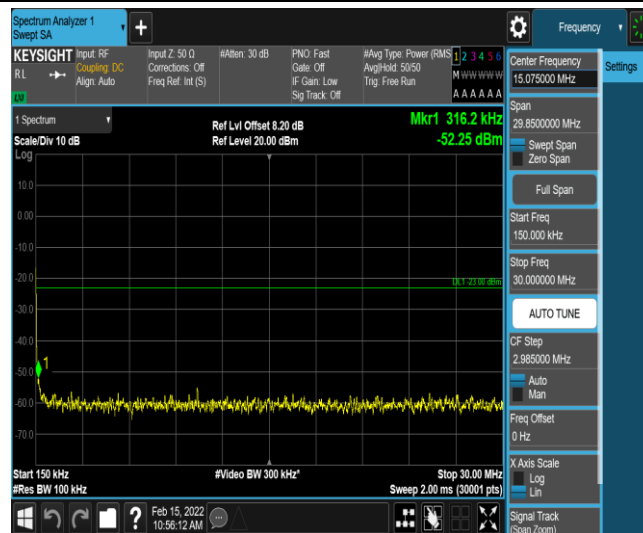
Band12-5MHz-QPSK-23155-1-0-High-0.15-30--52.25-PASS
