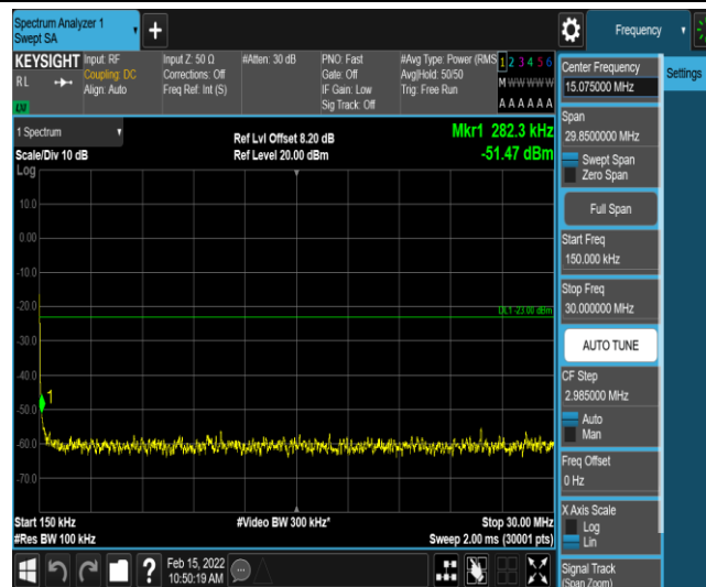
Band12-5MHz-QPSK-23035-1-0-Low-0.15-30--51.47-PASS
