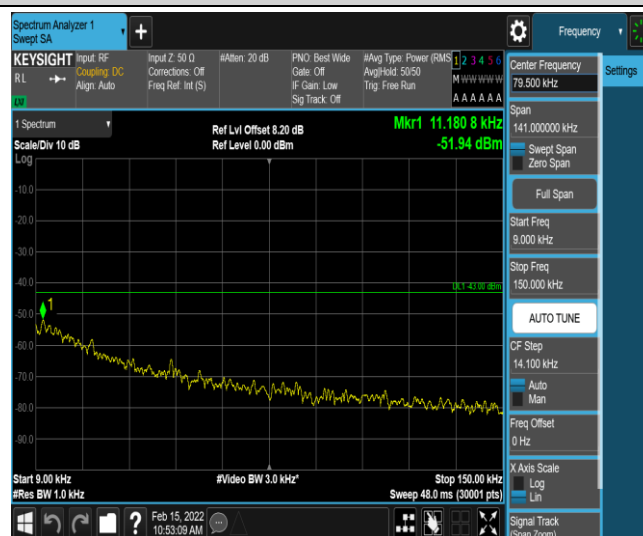
Band12-5MHz-QPSK-23095-1-0-Low-0.009-0.15--51.94-PASS
