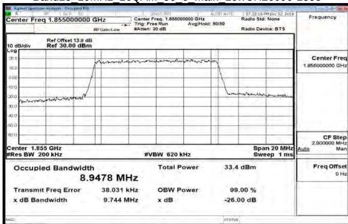
Band25 10MHz 16QAM 50 0 Main LowCH26090-1855
