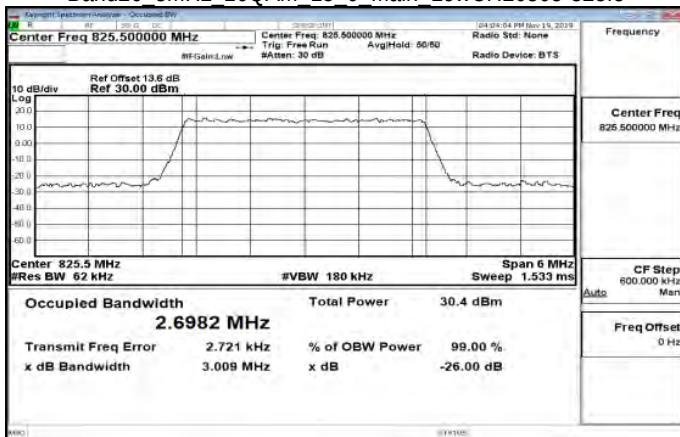
Band26 3MHz 16QAM 15 0 Main LowCH26805-825.5
