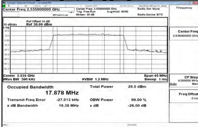
Band7 20MHz 256QAM 100 0 Main MidCH21100-2535
