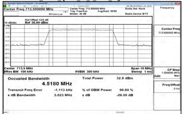
Band12 5MHz QPSK 25 0 Main HighCH23155-713.5
