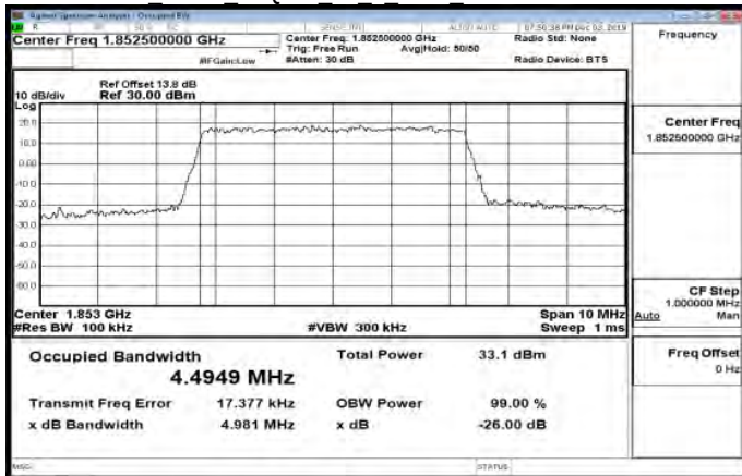
Band25 5MHz 16QAM 25 0 Main LowCH26065-1852.5
