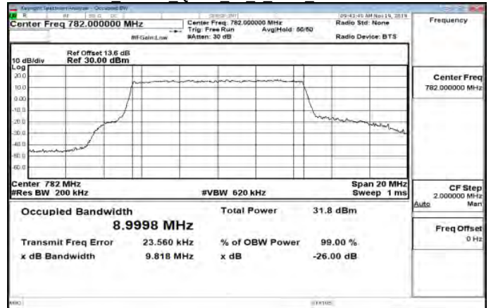
Band13 10MHz 16QAM 50 0 Main MidCH23230-782
