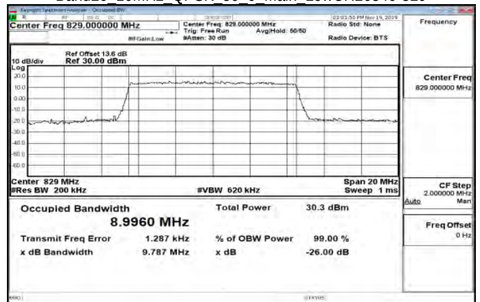
Band26 10MHz QPSK 50 0 Main LowCH26840-829
