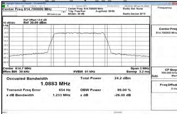
Band26 Part90s 1 4MHz 256QAM 6 0 Main LowCH26697-814.7
