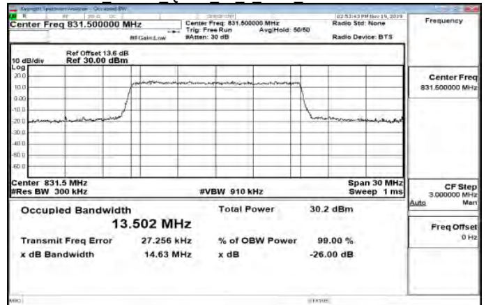
Band26 15MHz QPSK 75 0 Main LowCH26865-831.5
