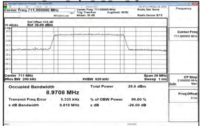
Band12 10MHz 64QAM 50 0 Main HighCH23130-711
