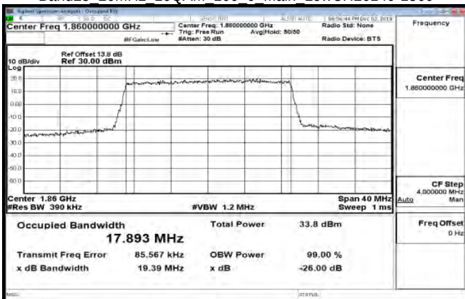
Band25 20MHz 16QAM 100 0 Main LowCH26140-1860
