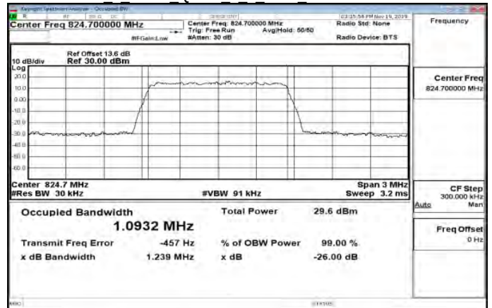
Band26 1 4MHz QPSK 6 0 Main LowCH26797-824.7
