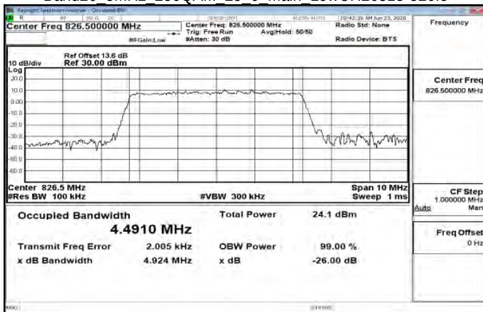
Band26 5MHz 256QAM 25 0 Main LowCH26815-826.5
