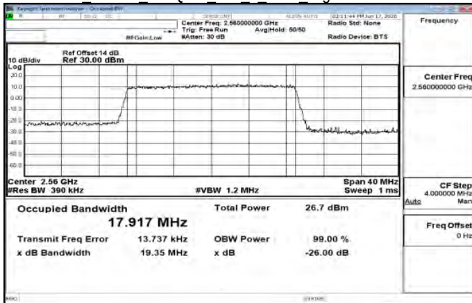
Band7 20MHz 256QAM 100 0 Main HighCH21350-2560
