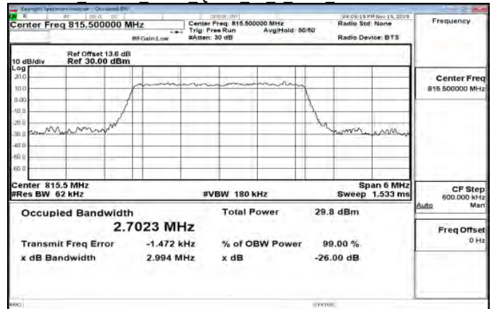
Band26 Part90s 3MHz QPSK 15 0 Main LowCH26705-815.5
