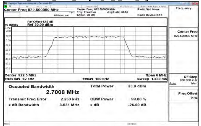
Band26 Part90s 3MHz 256QAM 15 0 Main HighCH26775-822.5
