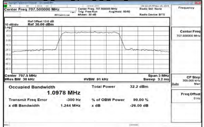
Band12 1 4MHz QPSK 6 0 Main MidCH23095-707.5
