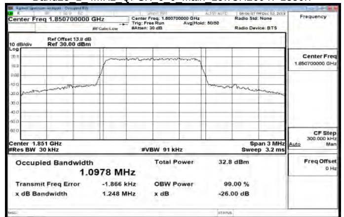
Band25 1 4MHz QPSK 6 0 Main LowCH26047-1850.7
