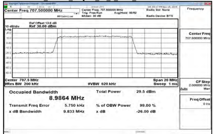
Band12 10MHz 64QAM 50 0 Main MidCH23095-707.5
