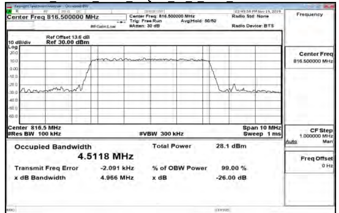
Band26 Part90s 5MHz 64QAM 25 0 Main LowCH26715-816.5
