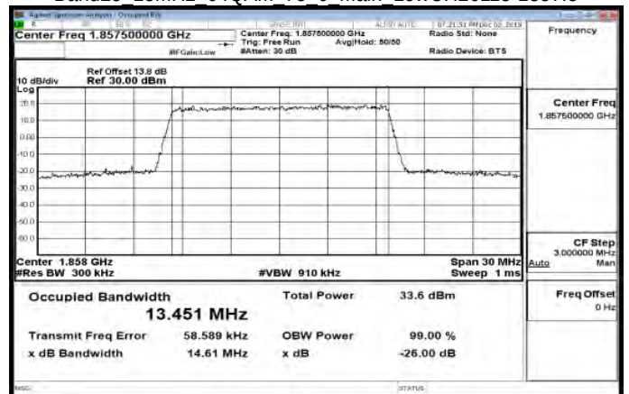
Band25 15MHz 64QAM 75 0 Main LowCH26115-1857.5
