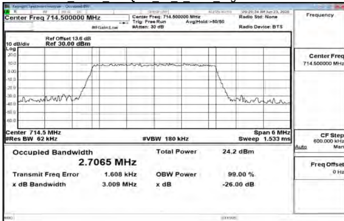
Band12 3MHz 256QAM 15 0 Main HighCH23165-714.5
