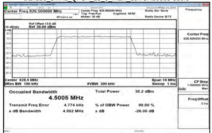
Band26 5MHz QPSK 25 0 Main LowCH26815-826.5
