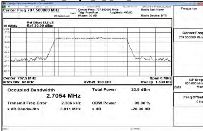
Band12 3MHz 256QAM 15 0 Main MidCH23095-707.5
