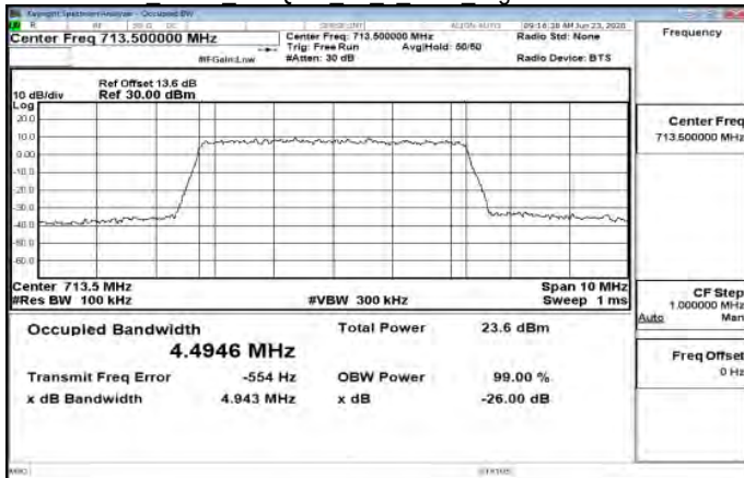
Band12 5MHz 256QAM 25 0 Main HighCH23155-713.5
