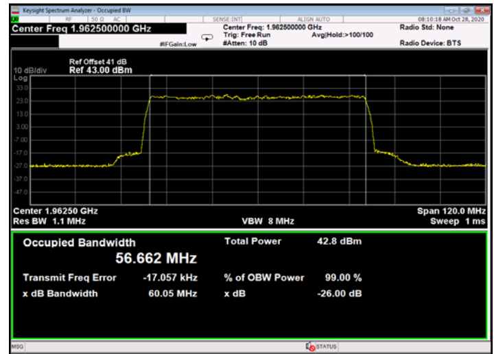
Figure 666: 64QAM 60MHz B.W.; 1962.5MHz, 60kHz - Output
