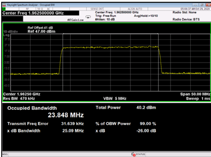
Figure 705: 256QAM 25MHz B.W.; 1962.5MHz, 15kHz - Output
