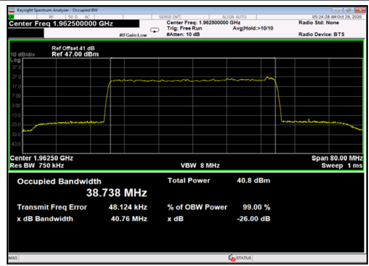
Figure 714: 256QAM 40MHz B.W.; 1962.5MHz, 15kHz - Output
