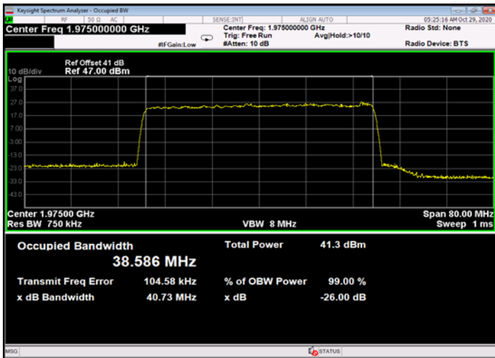
Figure 717: 256QAM 40MHz B.W.; 1975.0MHz, 15kHz - Output
