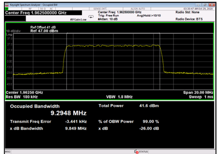
Figure 678: 256QAM 10MHz B.W.; 1962.5MHz, 15kHz - Output
