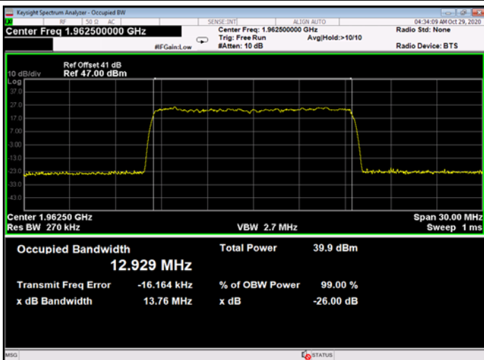
Figure 689: 256QAM 15MHz B.W.; 1962.5MHz, 60kHz - Output
