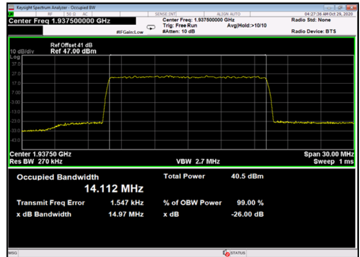
Figure 684: 256QAM 15MHz B.W.; 1937.5MHz, 15kHz - Output
