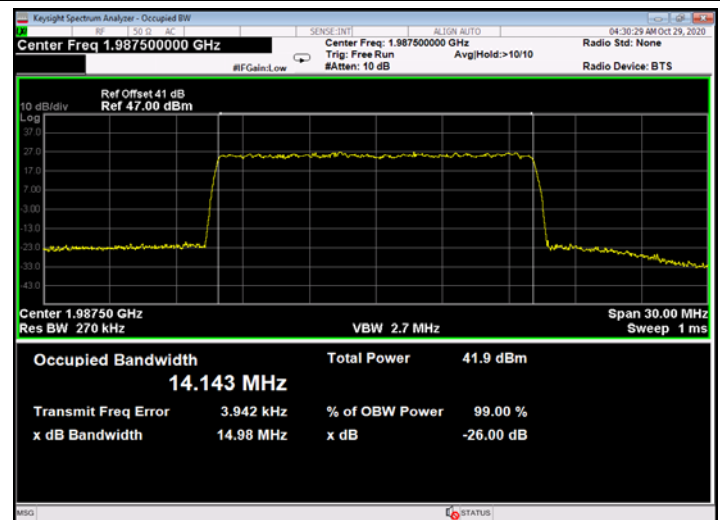
Figure 690: 256QAM 15MHz B.W.; 1987.5MHz, 15kHz - Output
