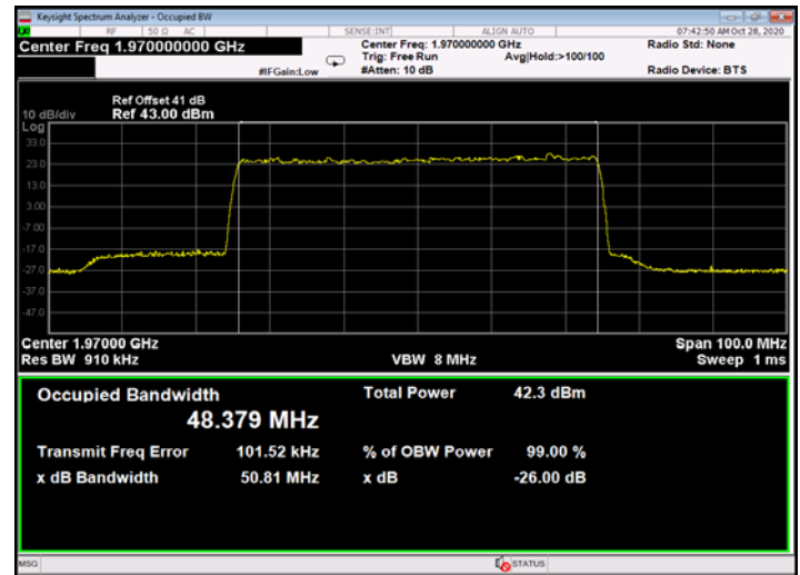
Figure 660: 64QAM 50MHz B.W.; 1970.0MHz, 15kHz - Output
