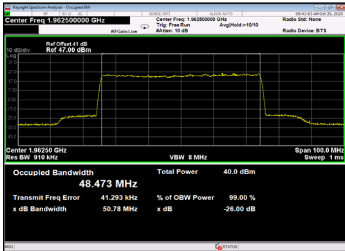
Figure 723: 256QAM 50MHz B.W.; 1962.5MHz, 15kHz - Output
