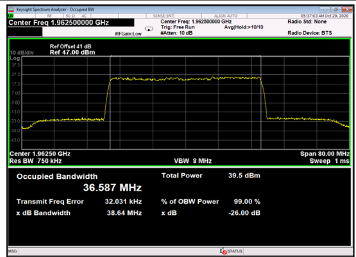
Figure 716: 256QAM 40MHz B.W.; 1962.5MHz, 60kHz - Output
