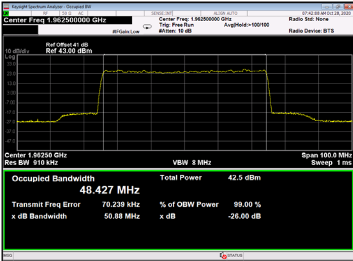
Figure 657: 64QAM 50MHz B.W.; 1962.5MHz, 15kHz - Output
