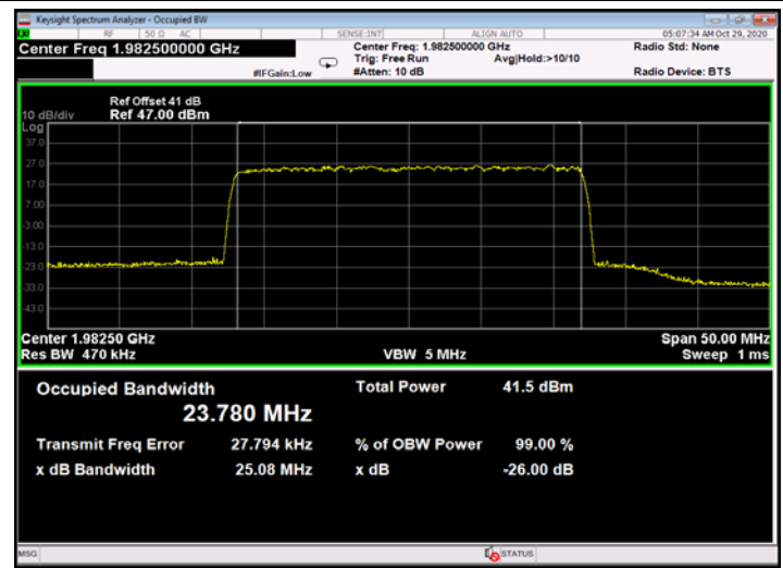
Figure 708: 256QAM 25MHz B.W.; 1982.5MHz, 15kHz - Output
