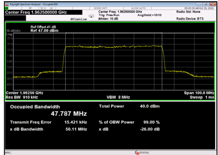
Figure 724: 256QAM 50MHz B.W.; 1962.5MHz, 30kHz - Output
