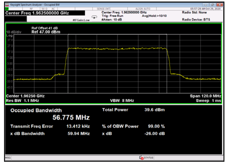
Figure 732: 256QAM 60MHz B.W.; 1962.5MHz, 60kHz - Output
