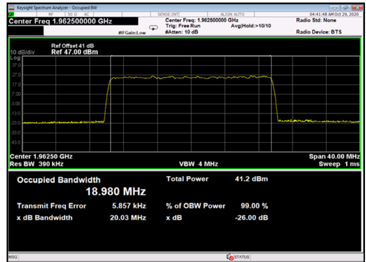
Figure 696: 256QAM 20MHz B.W.; 1962.5MHz, 15kHz - Output
