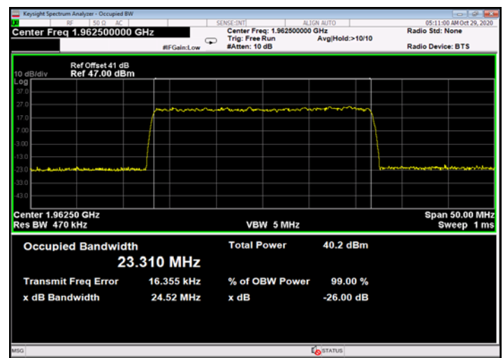
Figure 706: 256QAM 25MHz B.W.; 1962.5MHz, 30kHz - Output
