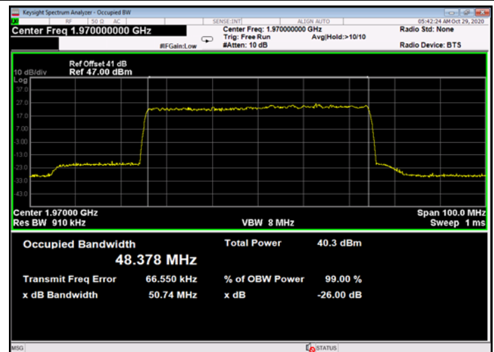
Figure 726: 256QAM 50MHz B.W.; 1970.0MHz, 15kHz - Output
