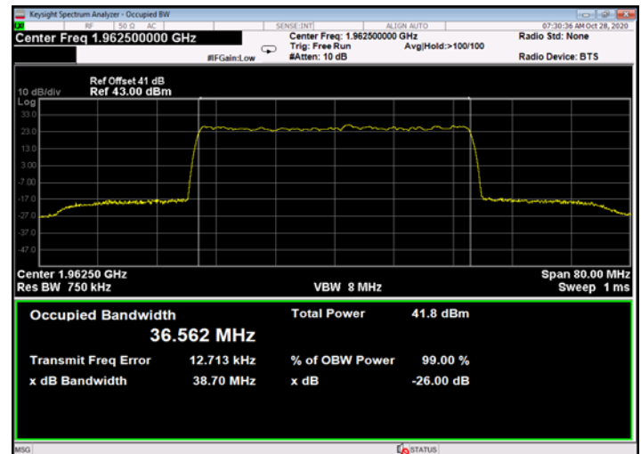
Figure 650: 64QAM 40MHz B.W.; 1962.5MHz, 60kHz - Output
