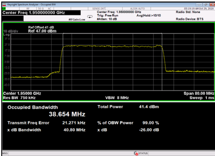
Figure 711: 256QAM 40MHz B.W.; 1950.0MHz, 15kHz - Output
