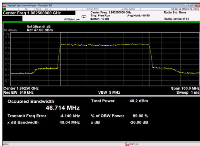
Figure 725: 256QAM 50MHz B.W.; 1962.5MHz, 60kHz - Output
