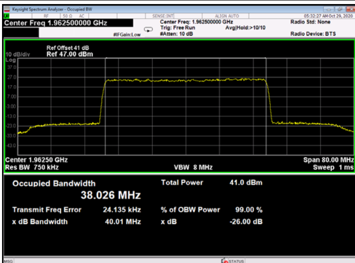
Figure 715: 256QAM 40MHz B.W.; 1962.5MHz, 30kHz - Output
