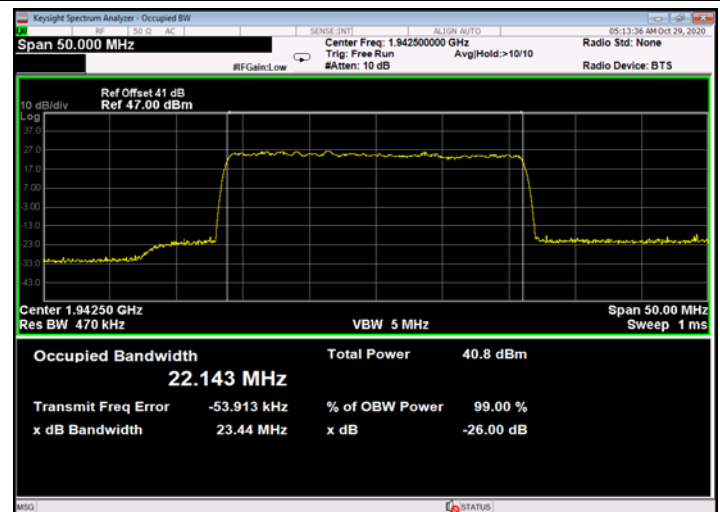
Figure 704: 256QAM 25MHz B.W.; 1942.5MHz, 60kHz - Output
