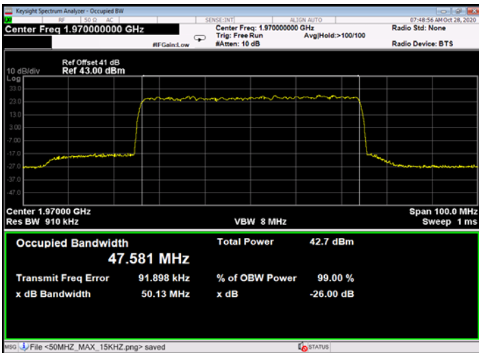
Figure 661: 64QAM 50MHz B.W.; 1970.0MHz, 30kHz - Output
