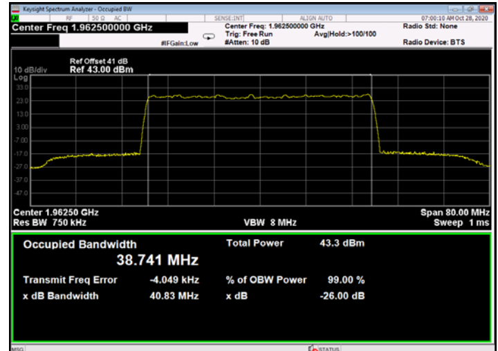
Figure 648: 64QAM 40MHz B.W.; 1962.5MHz, 15kHz - Output
