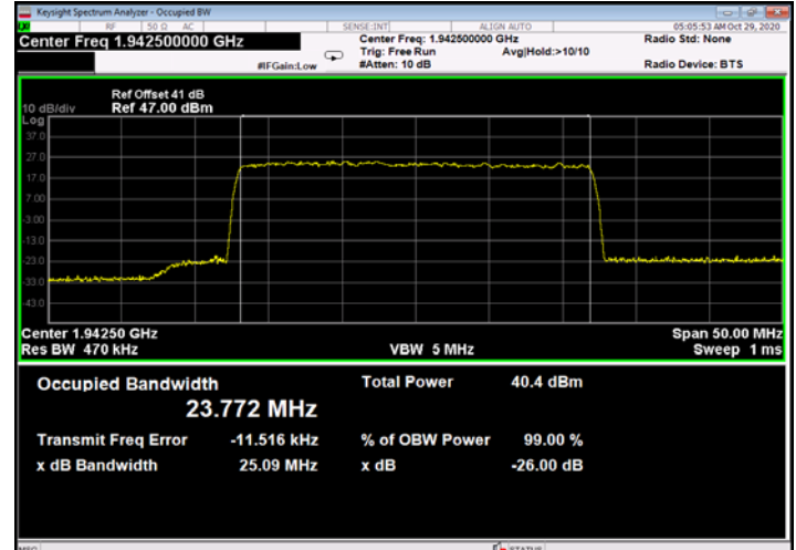
Figure 702: 256QAM 25MHz B.W.; 1942.5MHz, 15kHz - Output
