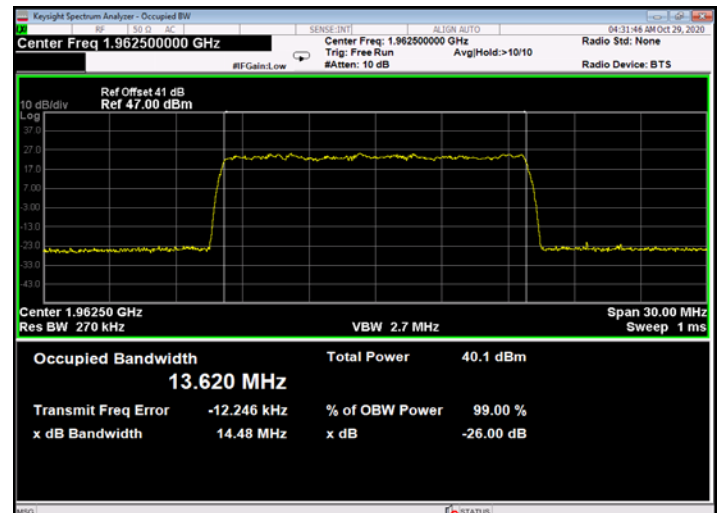
Figure 688: 256QAM 15MHz B.W.; 1962.5MHz, 30kHz - Output
