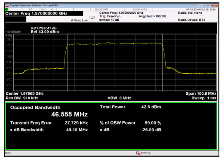
Figure 662: 64QAM 50MHz B.W.; 1970.0MHz, 60kHz - Output
