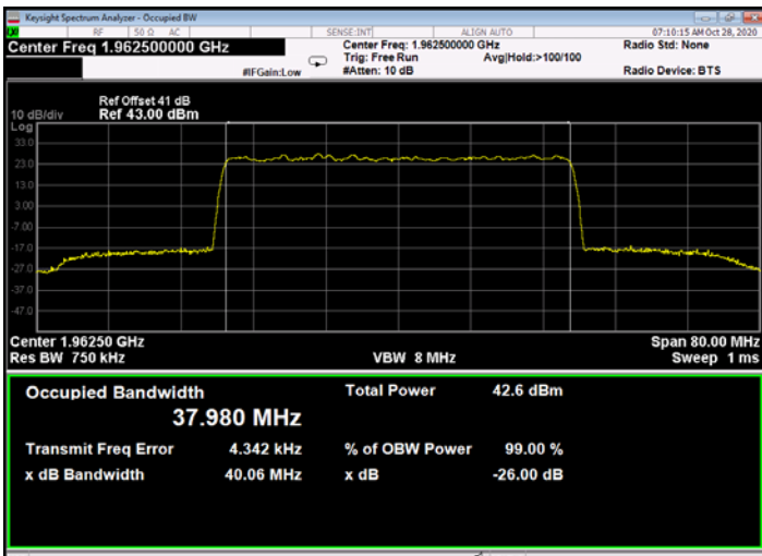
Figure 649: 64QAM 40MHz B.W.; 1962.5MHz, 30kHz - Output
