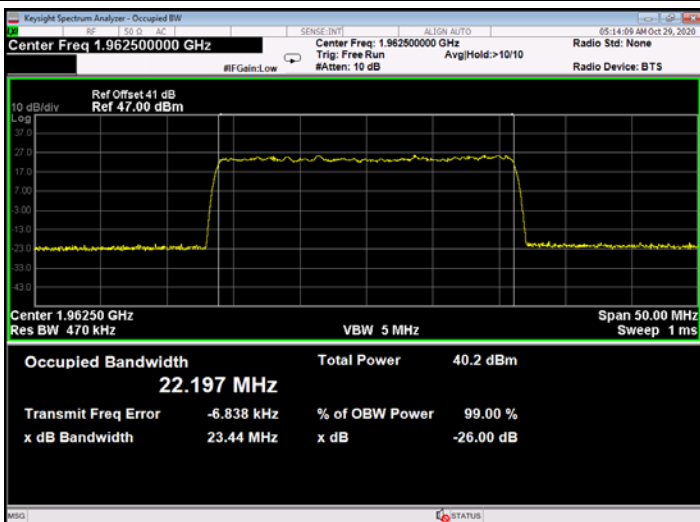
Figure 707: 256QAM 25MHz B.W.; 1962.5MHz, 60kHz - Output
