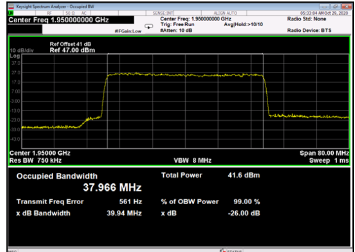
Figure 712: 256QAM 40MHz B.W.; 1950.0MHz, 30kHz - Output
