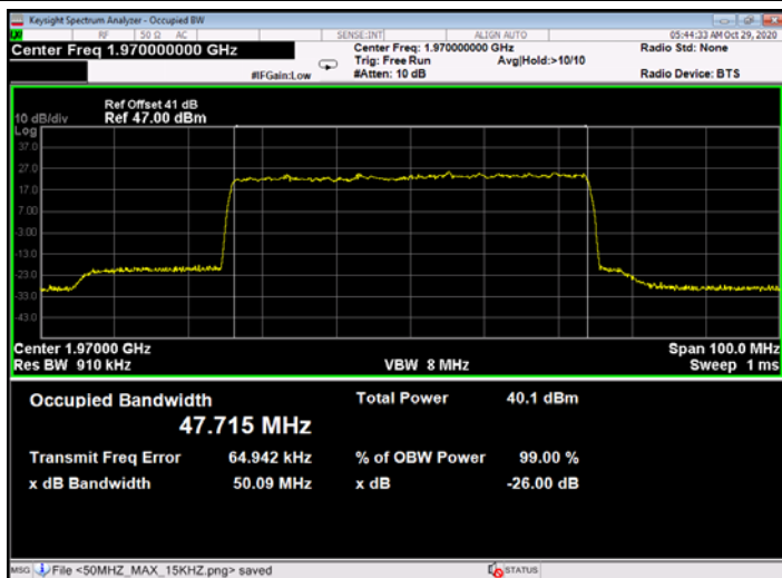
Figure 727: 256QAM 50MHz B.W.; 1970.0MHz, 30kHz - Output
