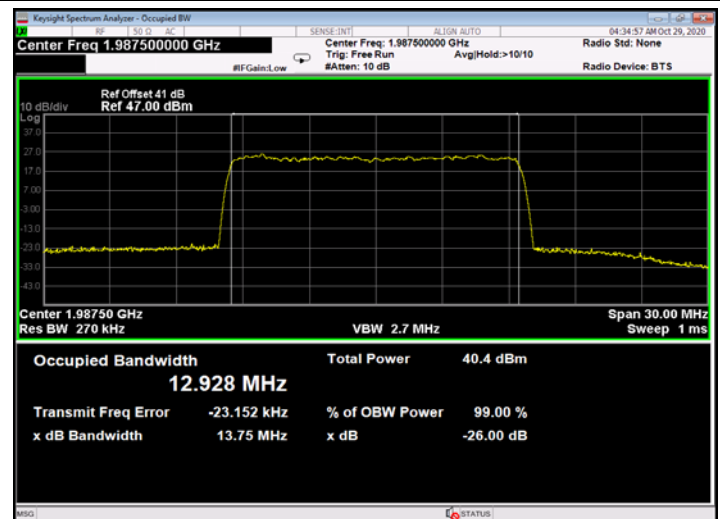
Figure 692: 256QAM 15MHz B.W.; 1987.5MHz, 60kHz - Output
