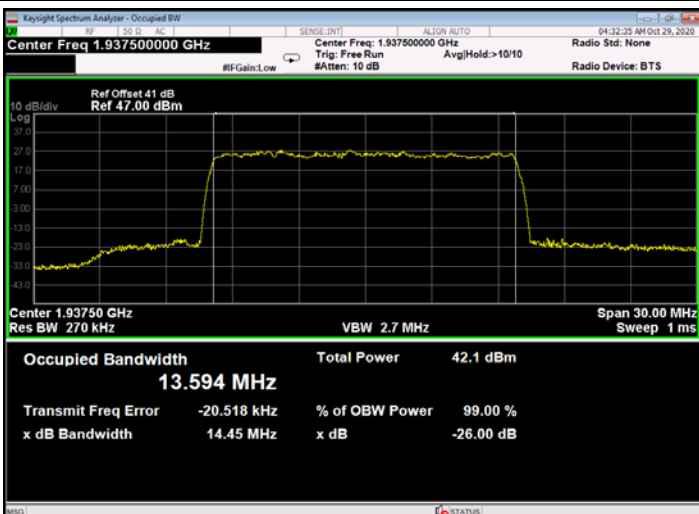
Figure 685: 256QAM 15MHz B.W.; 1937.5MHz, 30kHz - Output
