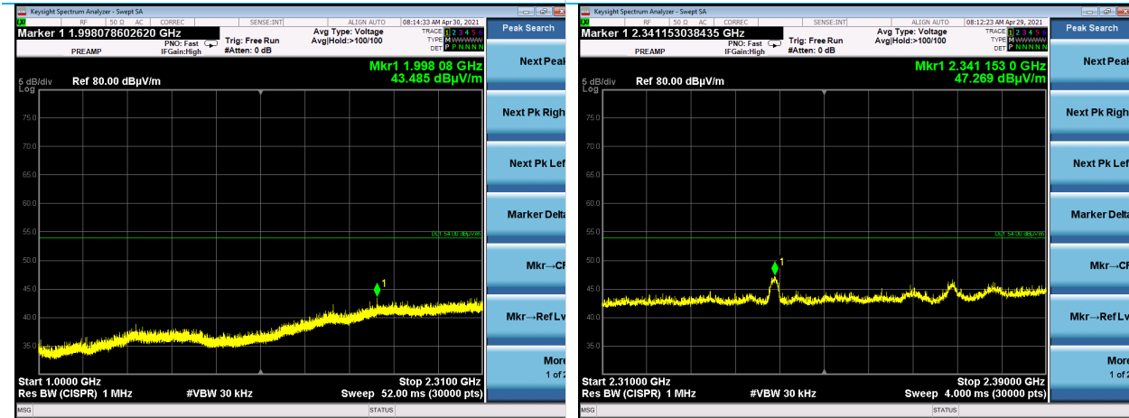
1-2.31 GHz, Horizontal Antenna Vertical EUT, Channel 25
