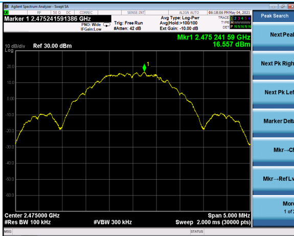
Neg4dBm, channel 25, reference plot 16.6 dBm
