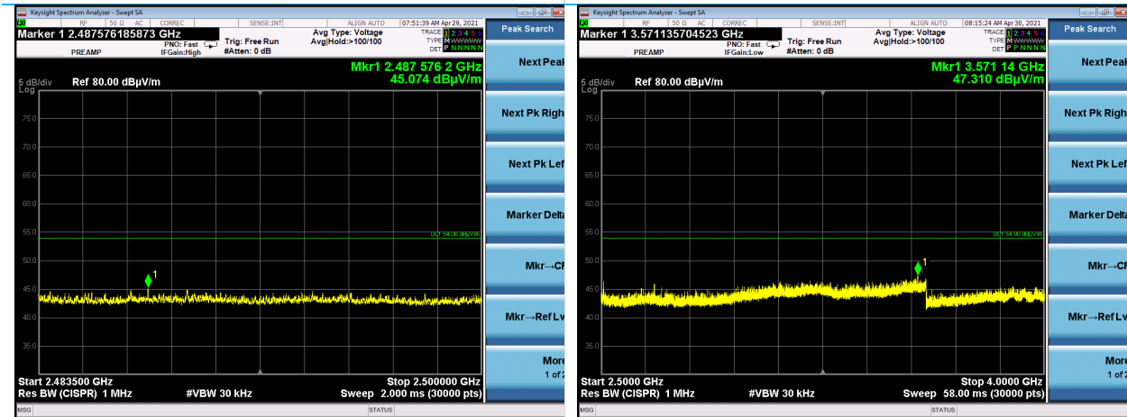
2.4835-2.5 GHz, Horizontal Antenna Vertical EUT, Channel 25
