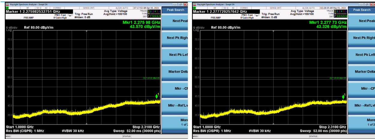
1-2.31 GHz, Horizontal Antenna Vertical EUT, Channel 11
