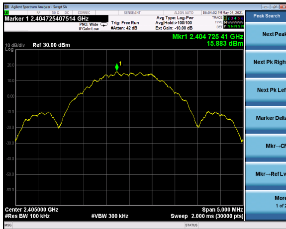
Neg4dBm, channel 11, reference plot 15.9 dBm
