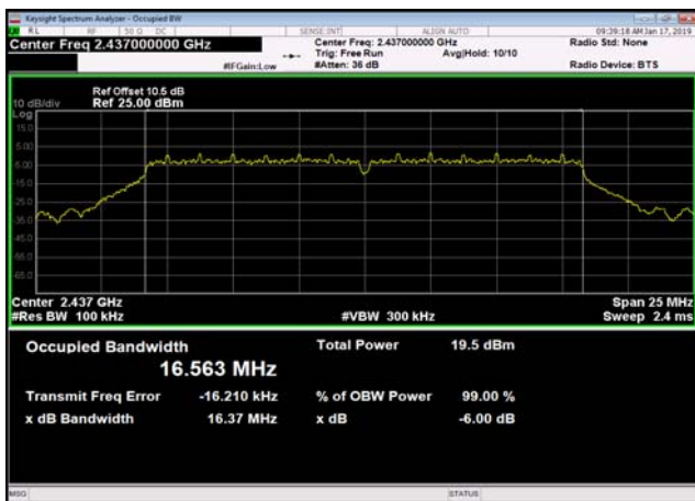
6dB Bandwidth-802.11g,2437MHz
