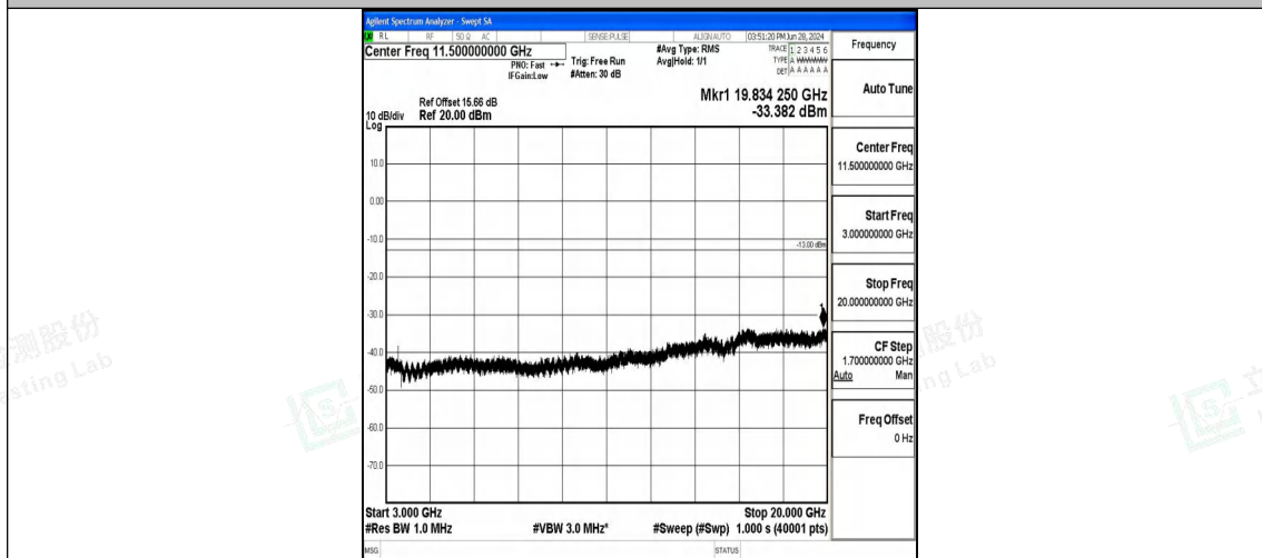
Band66_15MHz_QPSK_132322_1RB#0_3000~20000_3000~20000
