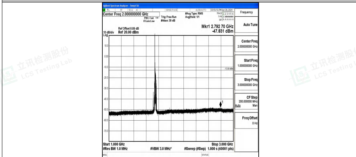
Band66_15MHz_16QAM_132322_1RB#0_1000~3000_1000~3000
