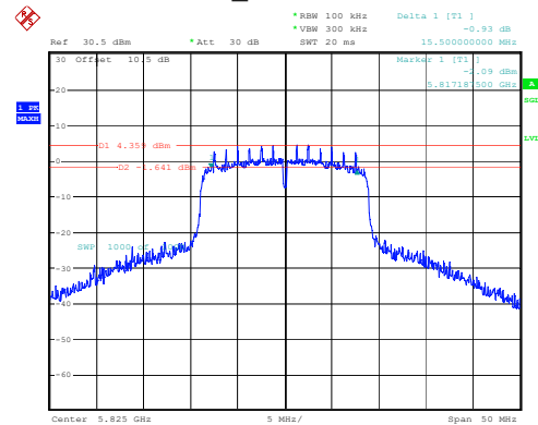
802.11n20_5825MHz 15.500MHz
