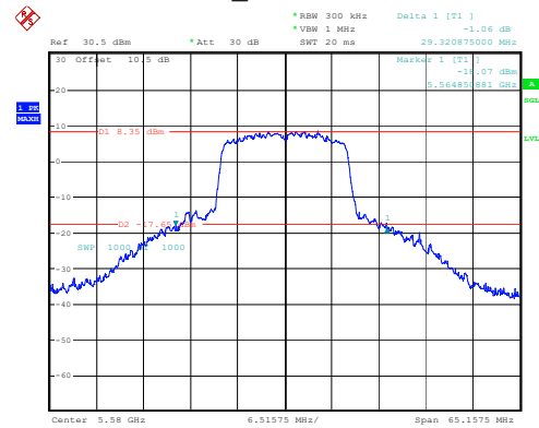
802.11n20_5580MHz 29.321MHz
