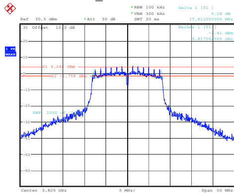
802.11a_5825MHz 15.813MHz
