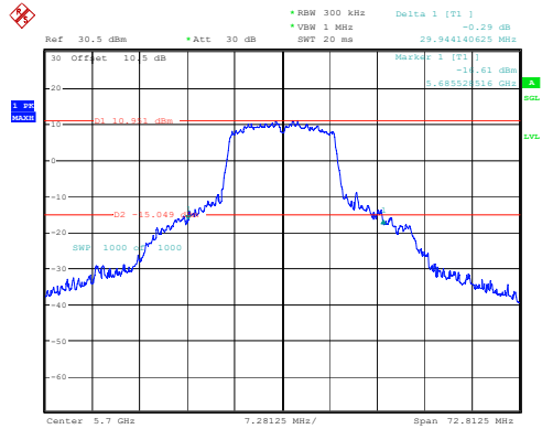
802.11a_5700MHz 29.944MHz
