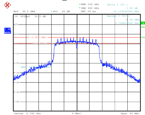
802.11n20_5745MHz 16.125MHz
