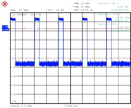
802.11a_5200MHz 1.346ms,6.905ms
