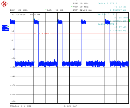
802.11n20_5200MHz 1.236ms,6.462ms
