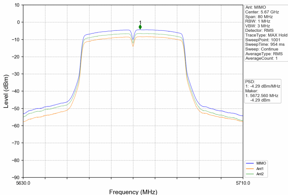
802.11ac(VHT40)_HCH_5670MHz_MIMO_NTNV
