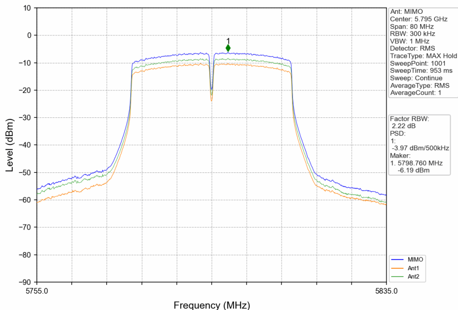
802.11ac(VHT40)_HCH_5795MHz_MIMO_NTNV
