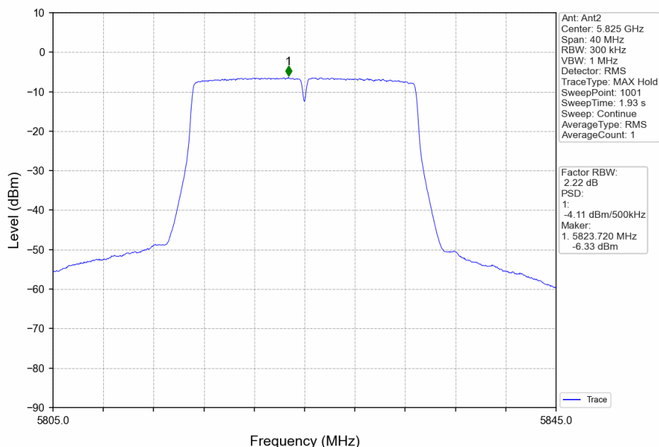
802.11ac(VHT20)_HCH_5825MHz_MIMO_NTNV
