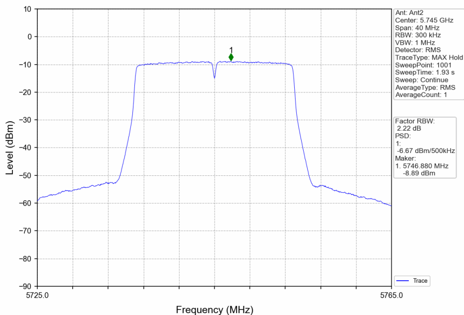
802.11ac(VHT20)_LCH_5745MHz_MIMO_NTNV
