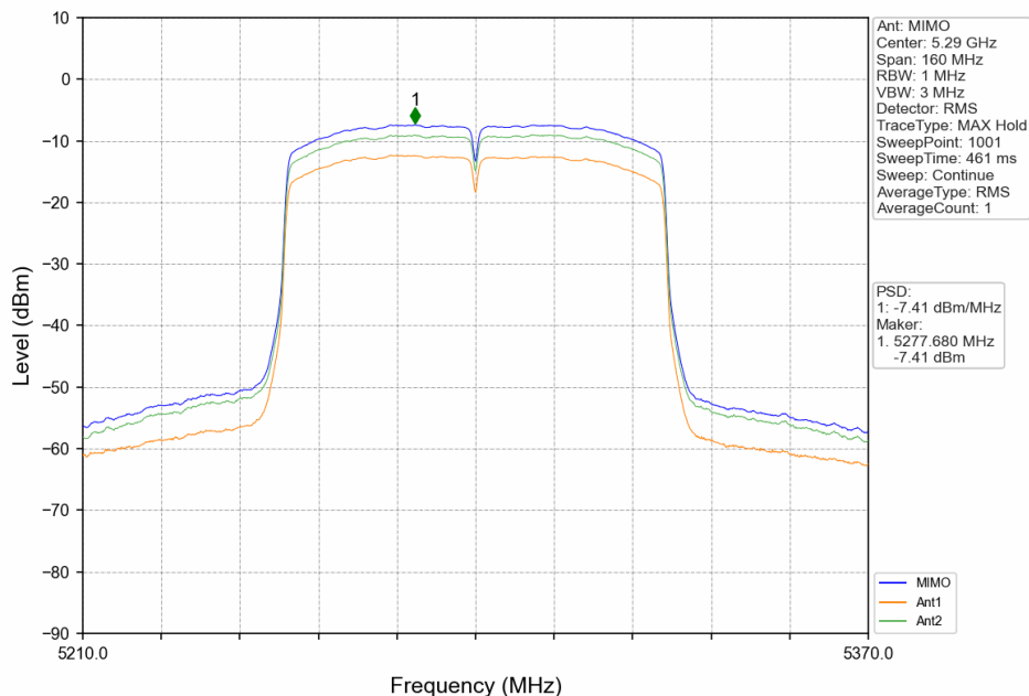
802.11ac(VHT80)_MCH_5290MHz_MIMO_NTNV
