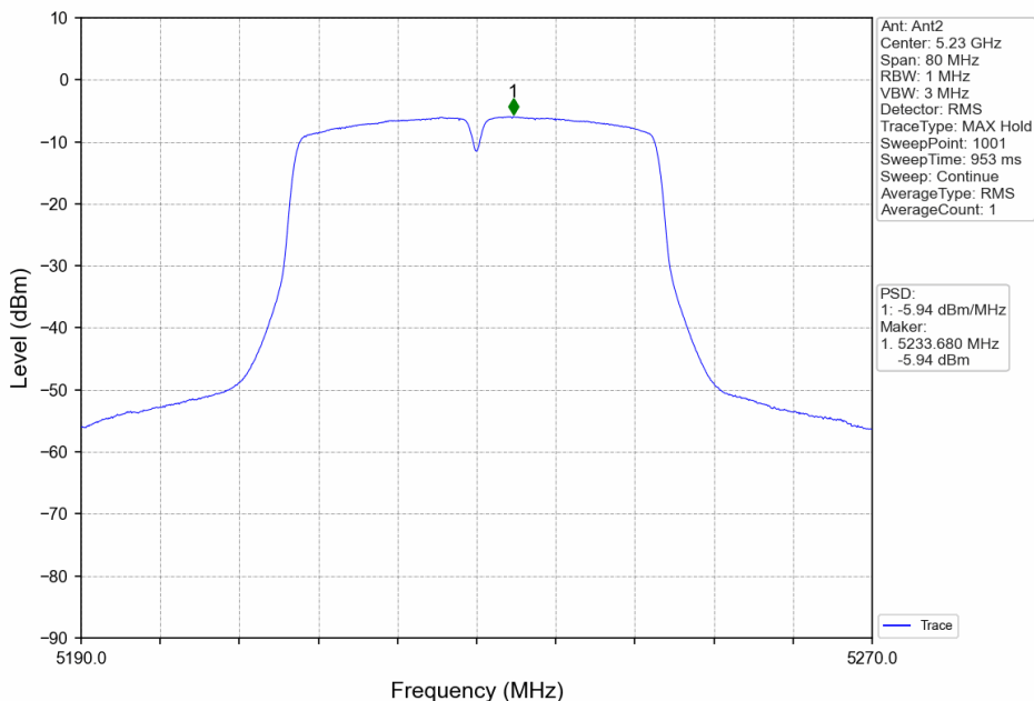
802.11ac(VHT40)_HCH_5230MHz_Ant2_NTNV
