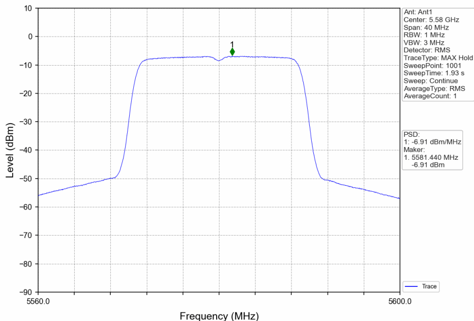
802.11ac(VHT20)_MCH_5580MHz_Ant1_NTNV
