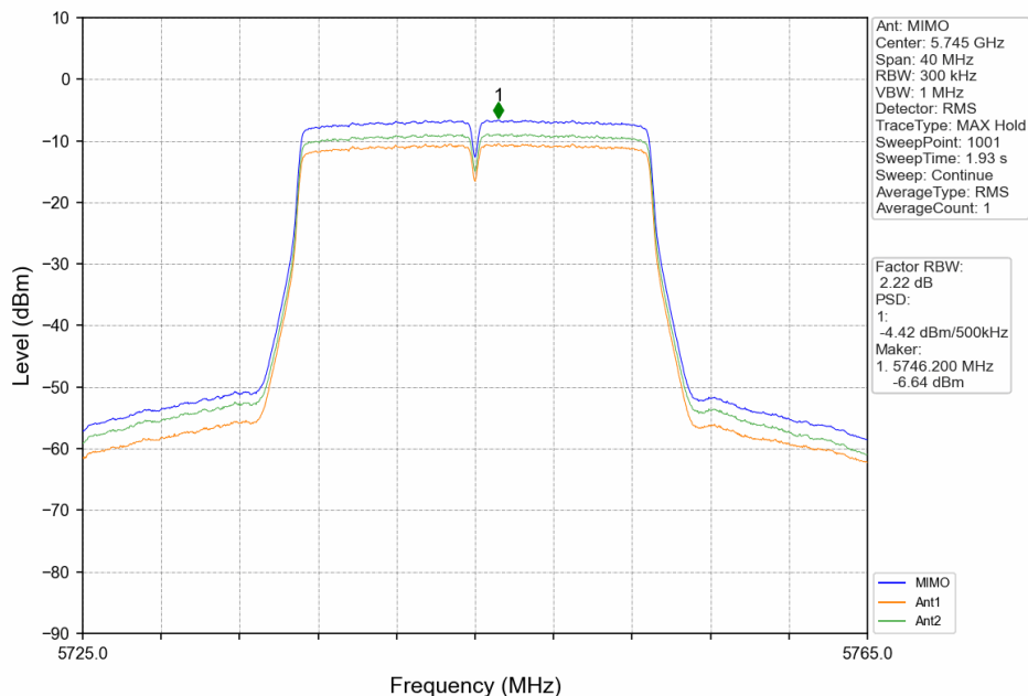
802.11ac(VHT20)_LCH_5745MHz_MIMO_NTNV
