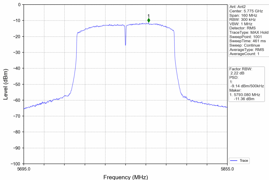
802.11ac(VHT80)_MCH_5775MHz_Ant2_NTNV
