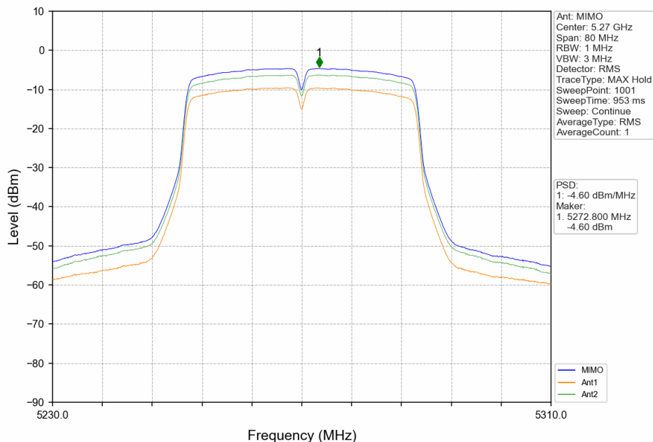
802.11ac(VHT40)_LCH_5270MHz_MIMO_NTNV
