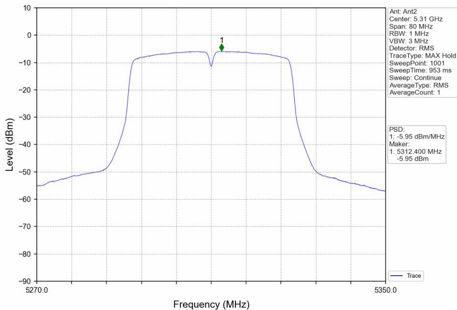
802.11ac(VHT40)_HCH_5310MHz_Ant2_NTNV
