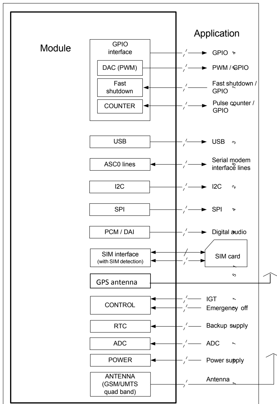
Figure 1: PDS8 system overview
