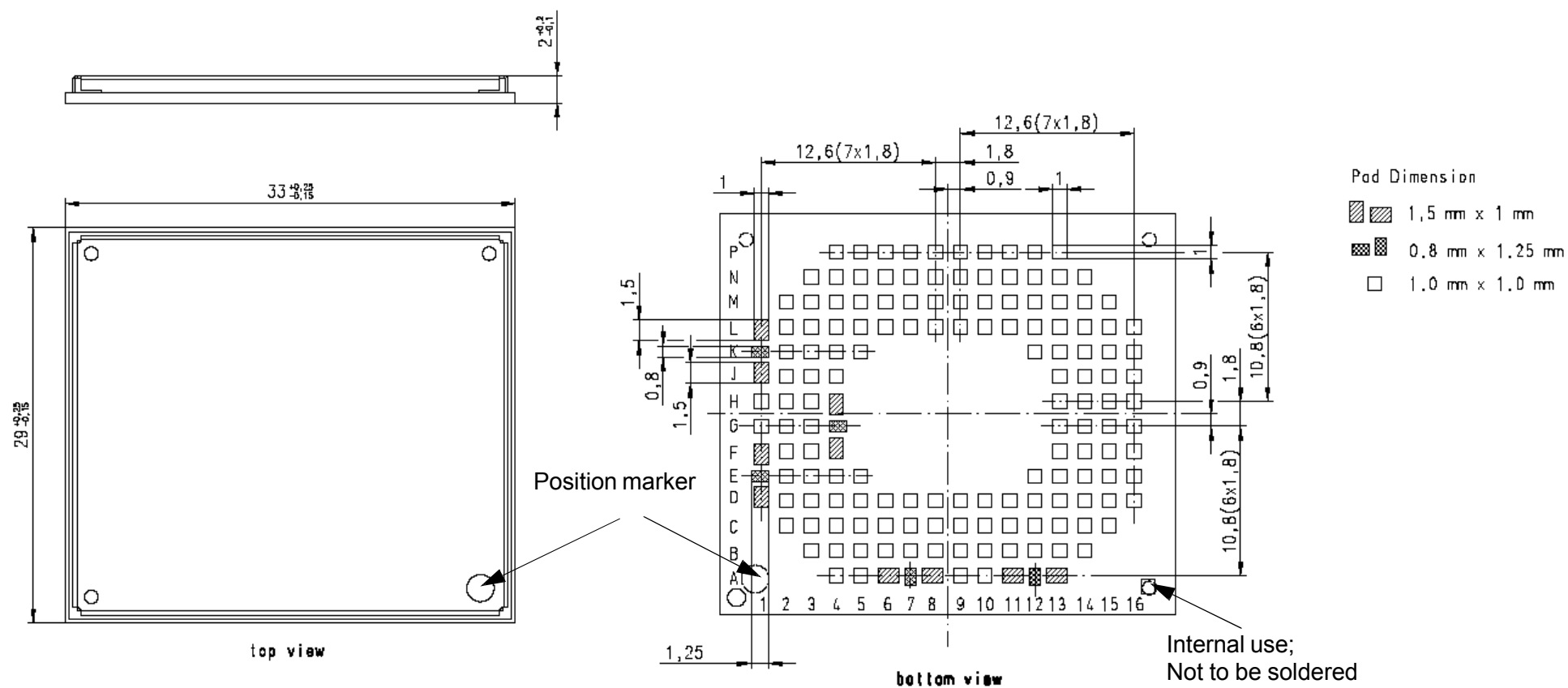
Figure 6: Dimensions of PDS8 (all dimensions in mm)
