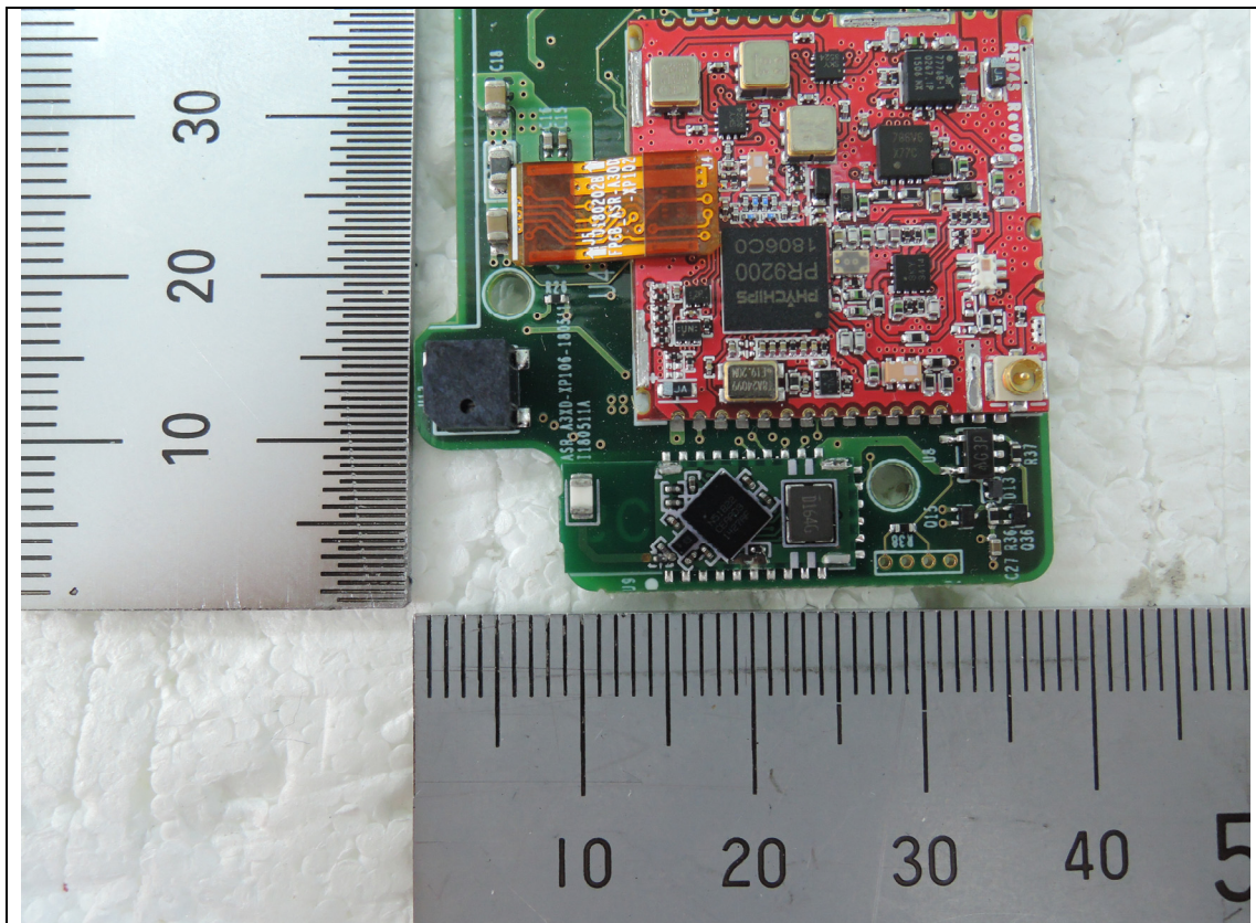
&lt;BLE Antenna&gt;
