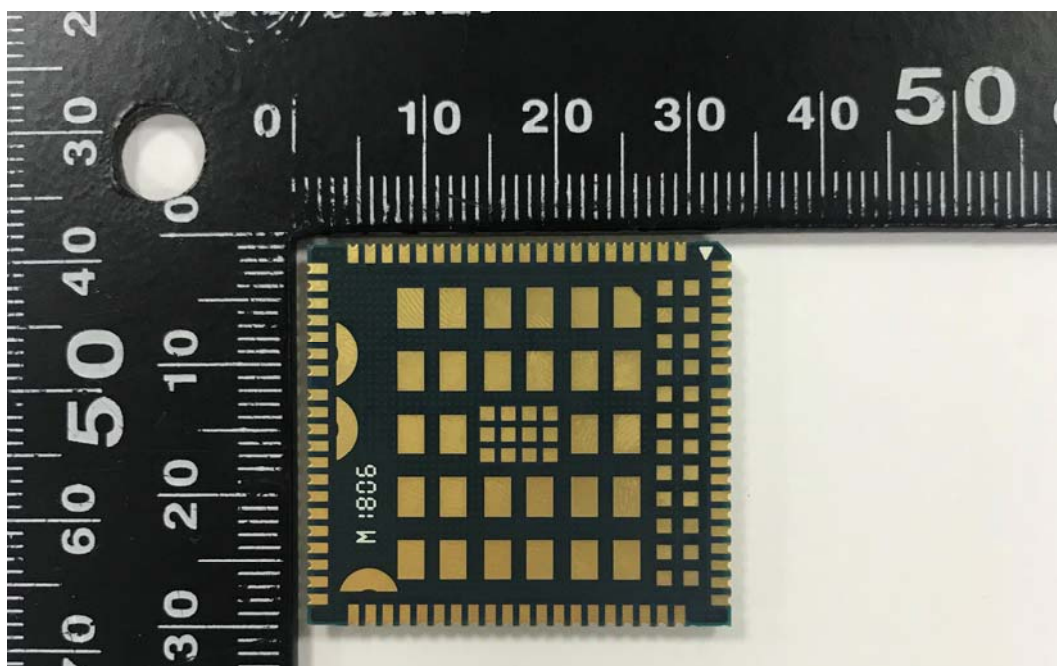
Back Side
