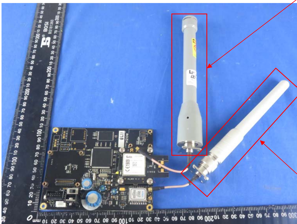
2G/3G/4G ANT
