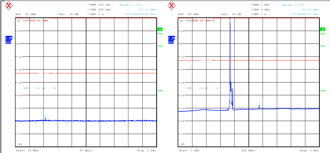
Date: 24.SEP.2024 06:42:21 Band66-20MHz-QPSK-132322-1RB#0-30~1000-PASS Date: 24.SEP.2024 06:42:35 Band66-20MHz-QPSK-132322-1RB#0-1000~3000-PASS
