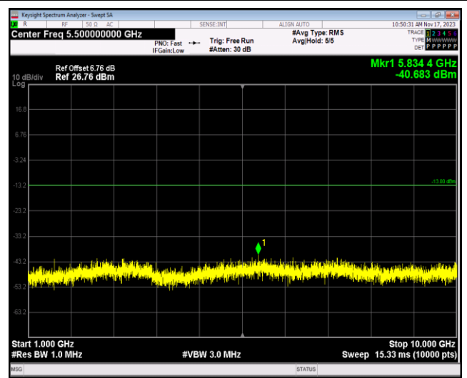
Band13-10MHz-QPSK-23230-1RB#0-Range4:1000~10000MHz
