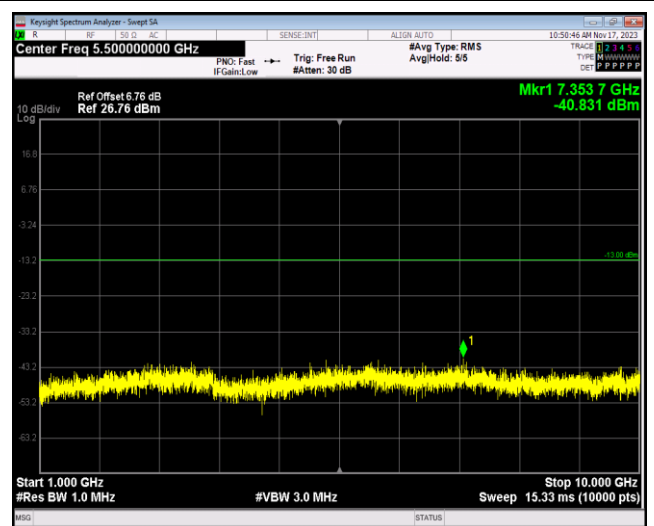
Band13-10MHz-16QAM-23230-1RB#0-Range2:1000 ~10000MHz
