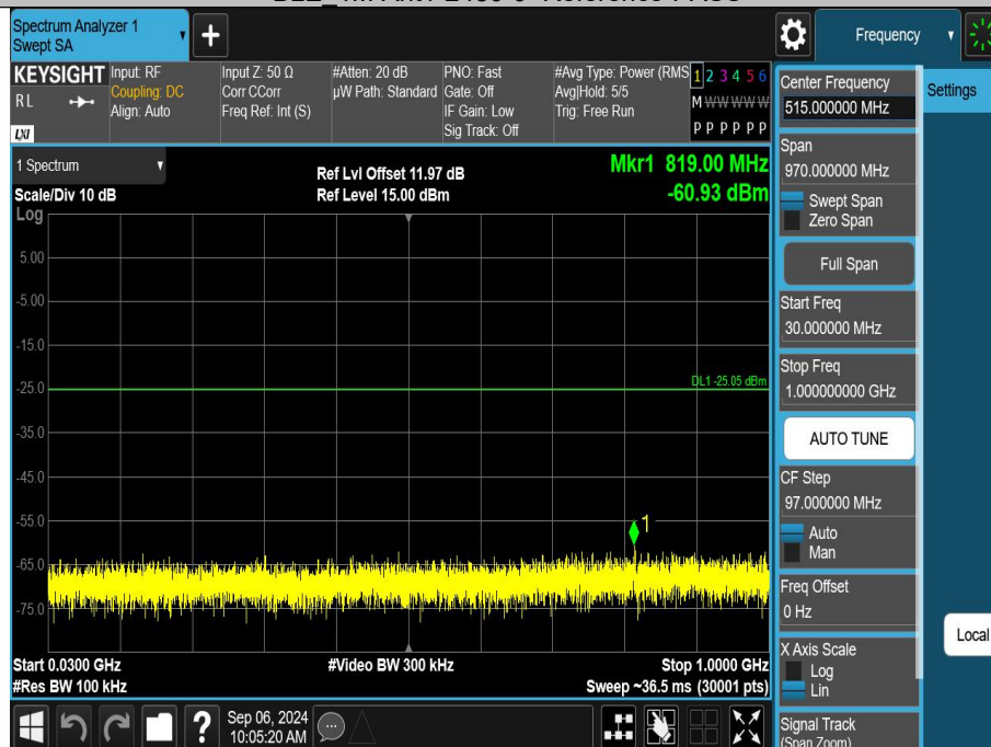
BLE_1M-Ant1-2480-30~1000-PASS
