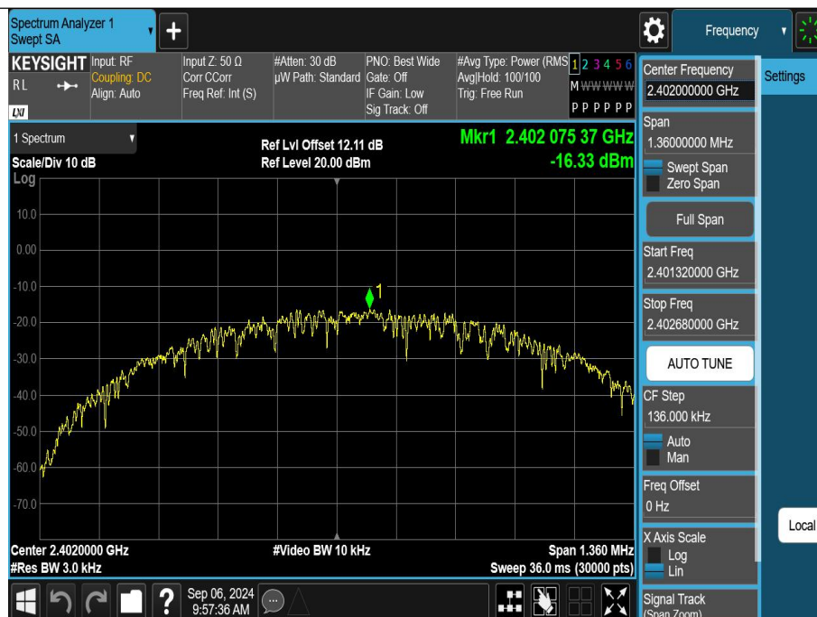
BLE_1M-Ant1-2402-PASS
