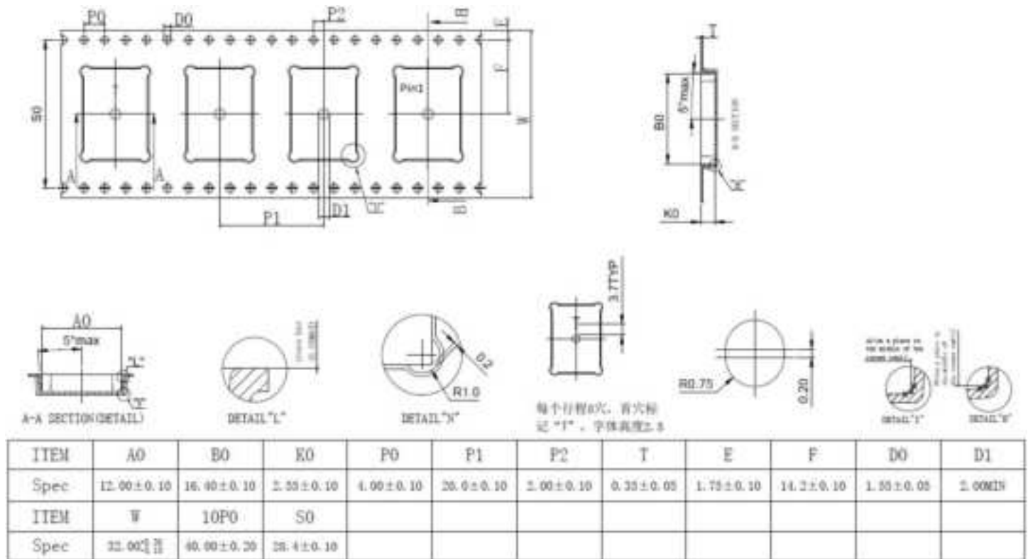
Figure 15.2. Tape Dimensions
