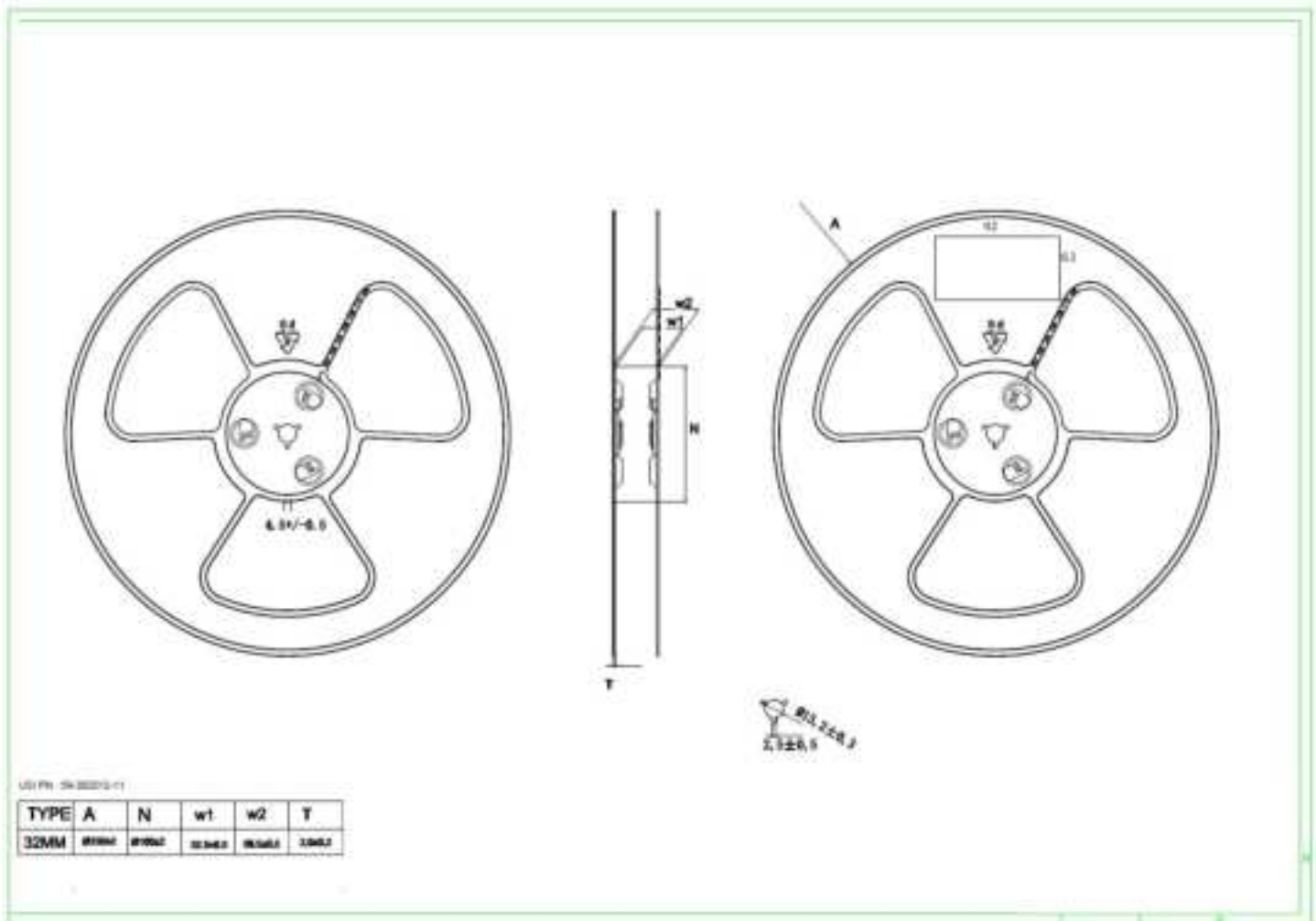
Figure 15.1. Reel Dimensions
