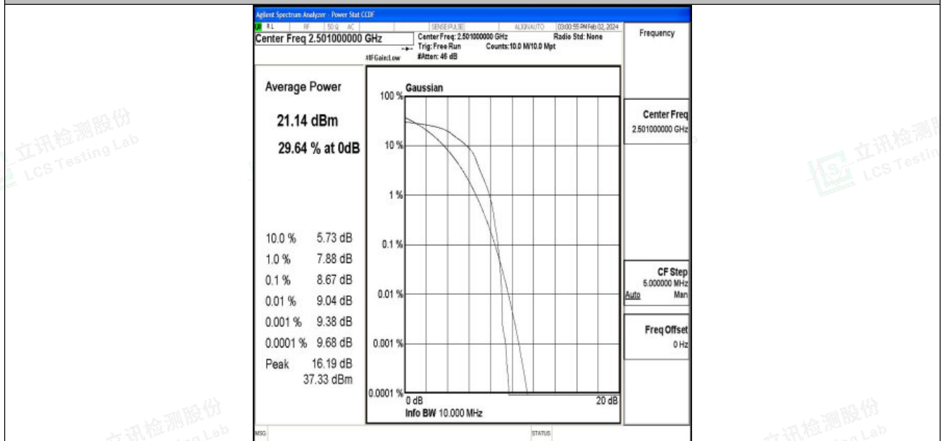
Band41-10MHz-16QAM-39700-1RB#0-PASS
