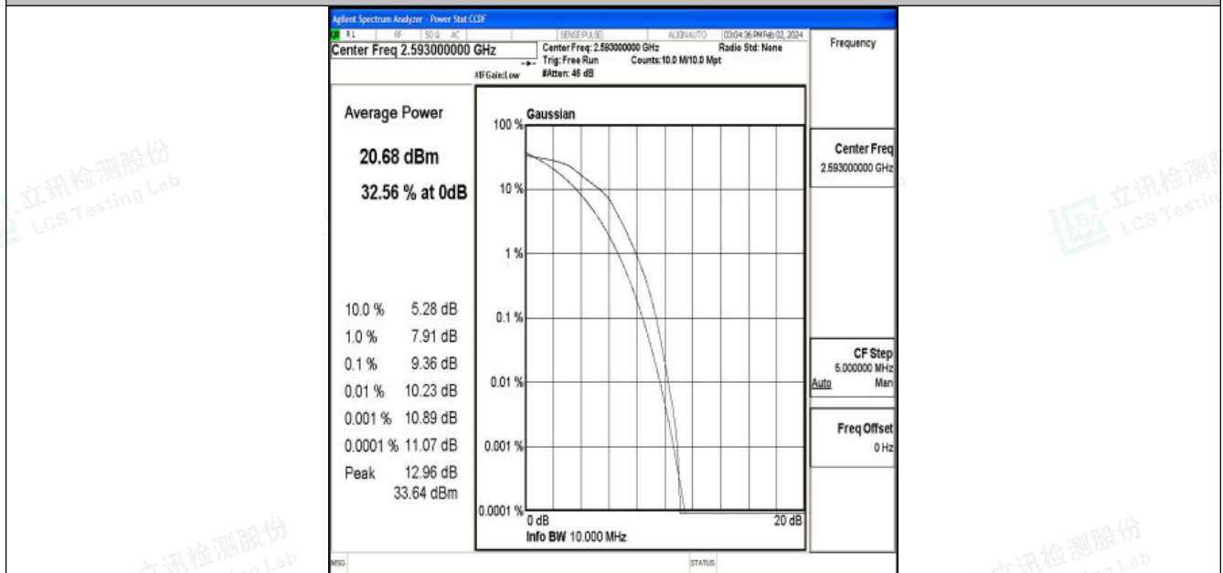
Band41-10MHz-16QAM-40620-50RB#0-PASS
