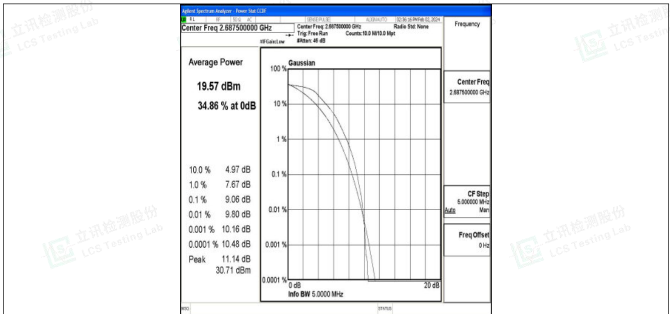
Band41-5MHz-QPSK-41565-25RB#0-PASS
