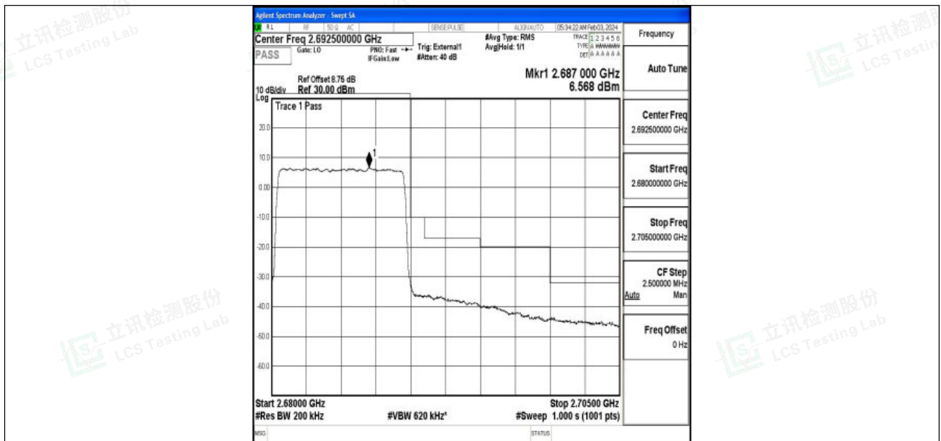
Band41_10MHz_16QAM_41540_50RB#0
