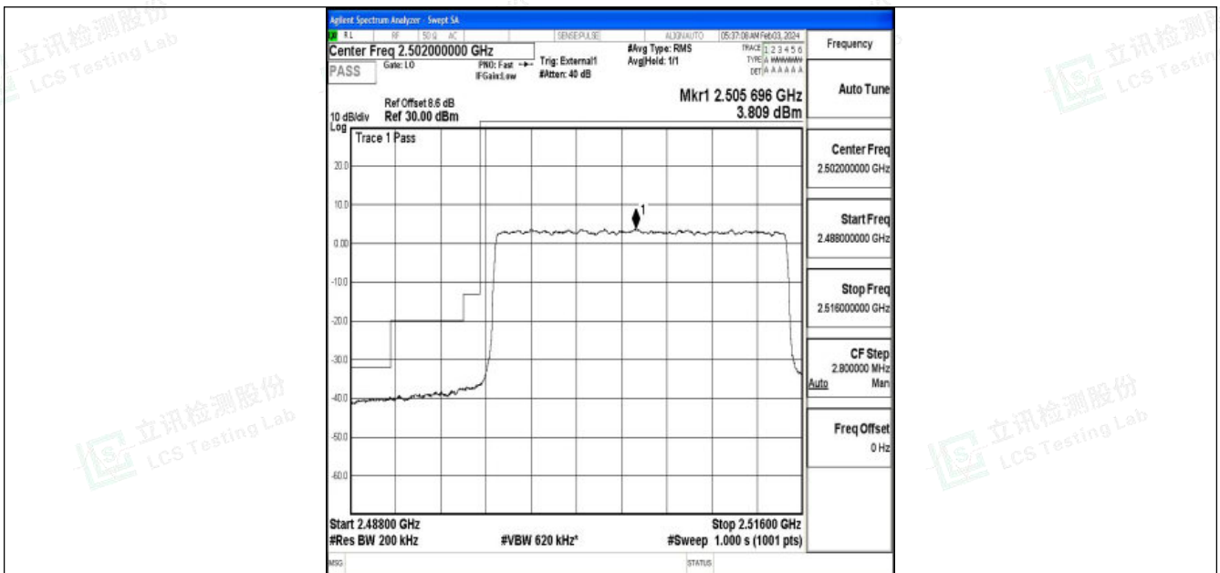
Band41_20MHz_16QAM_39750_100RB#0
