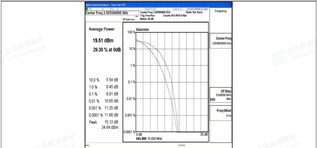
Band41-15MHz-16QAM-39725-75RB#0-PASS
