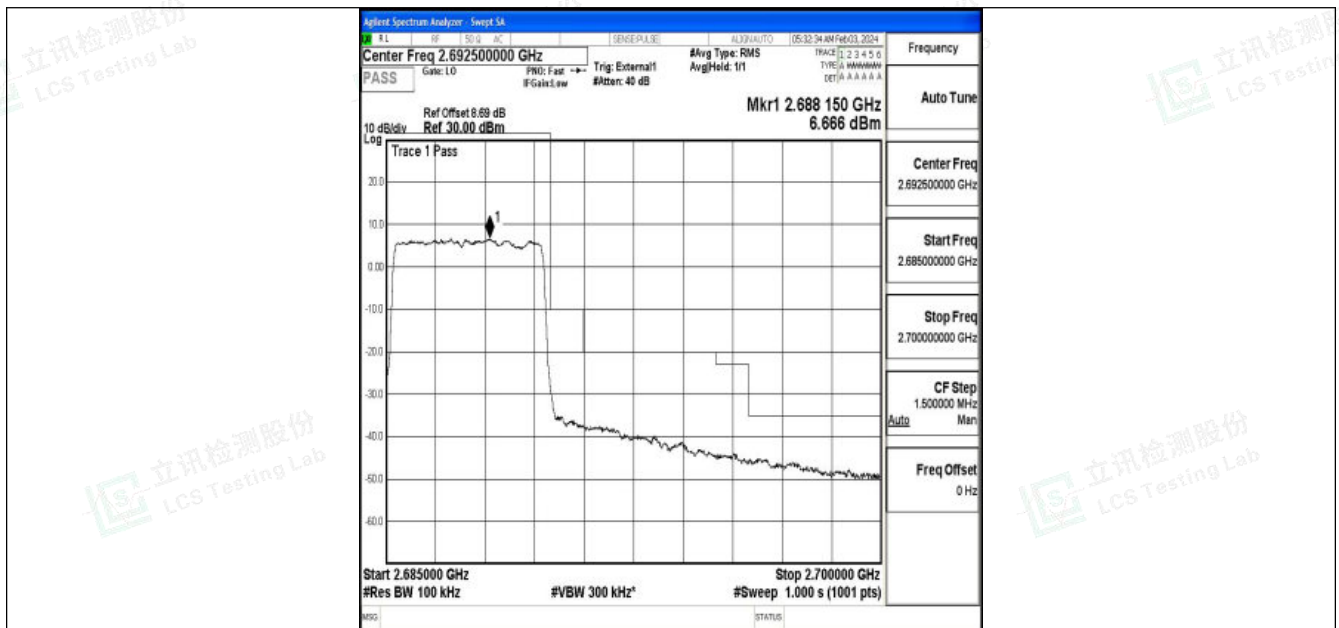
Band41_5MHz_16QAM_41565_25RB#0
