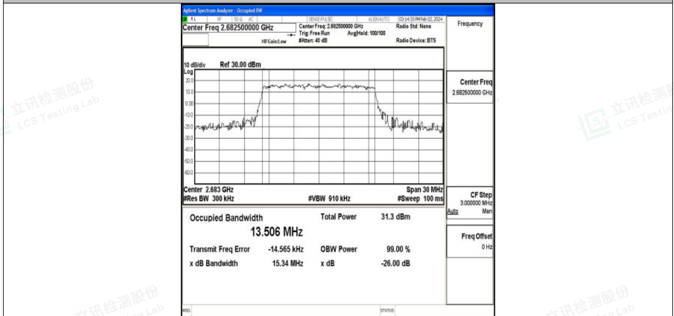
Band41-15MHz-16QAM-41515-75RB#0-PASS
