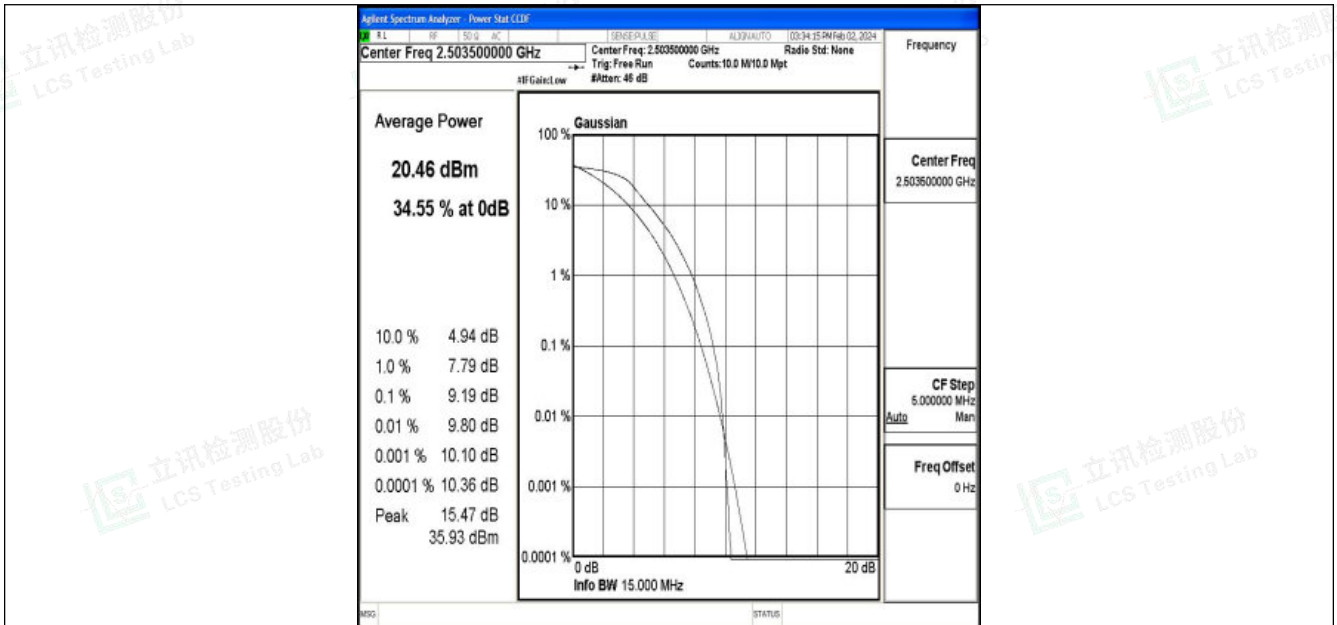
Band41-15MHz-QPSK-39725-75RB#0-PASS
