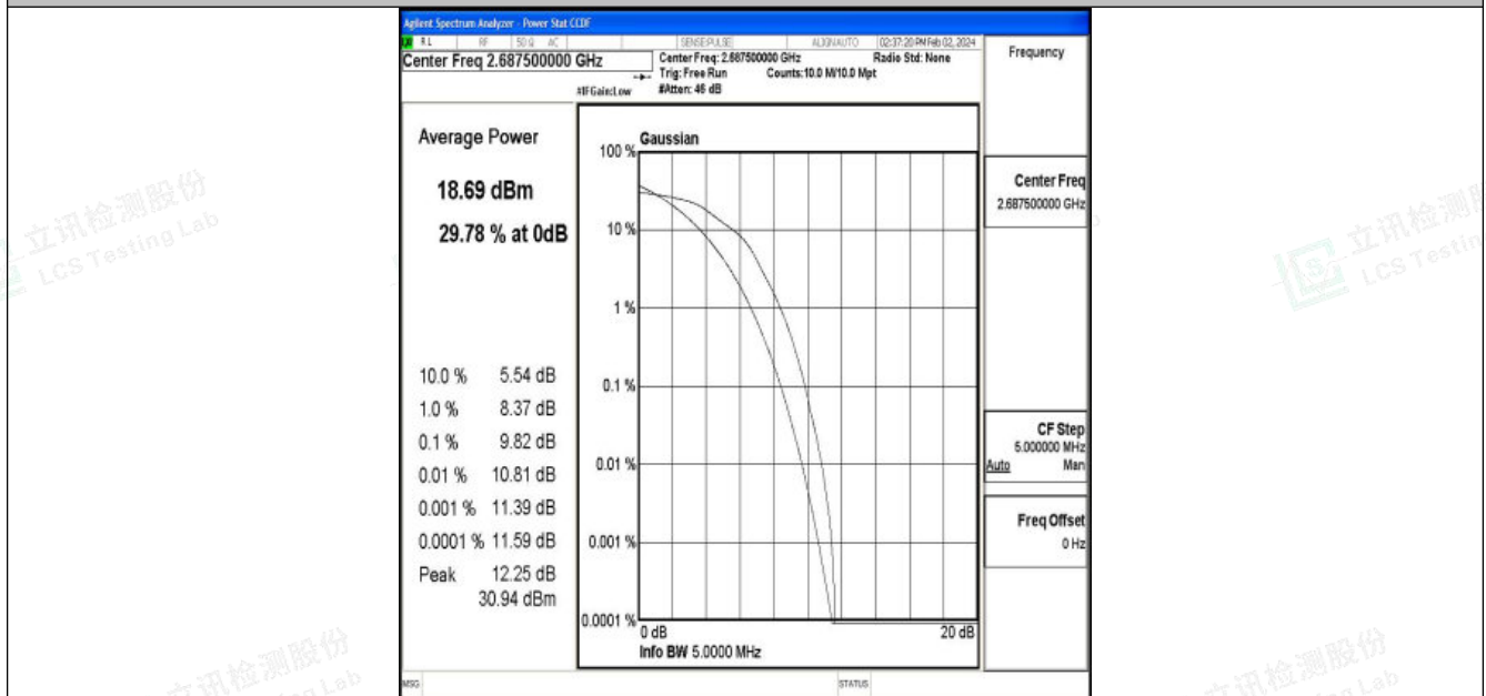
Band41-5MHz-16QAM-41565-25RB#0-PASS
