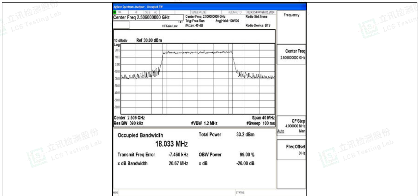
Band41-20MHz-QPSK-39750-100RB#0-PASS
