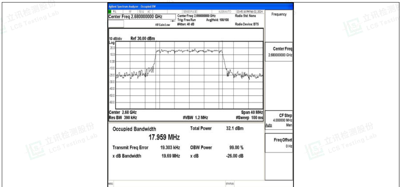
Band41-20MHz-QPSK-41490-100RB#0-PASS
