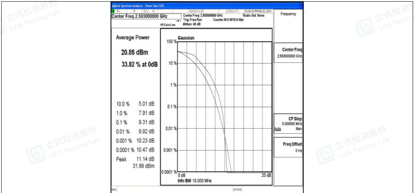
Band41-15MHz-QPSK-40620-75RB#0-PASS
