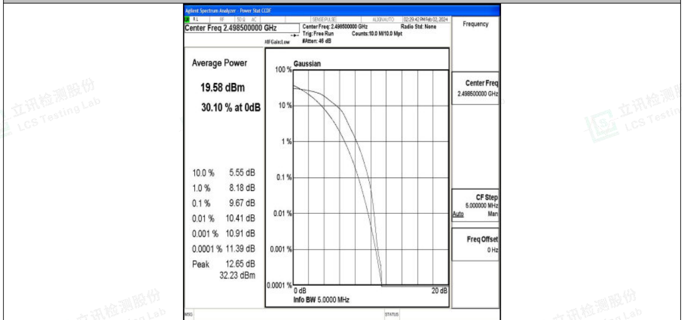
Band41-5MHz-16QAM-39675-25RB#0-PASS
