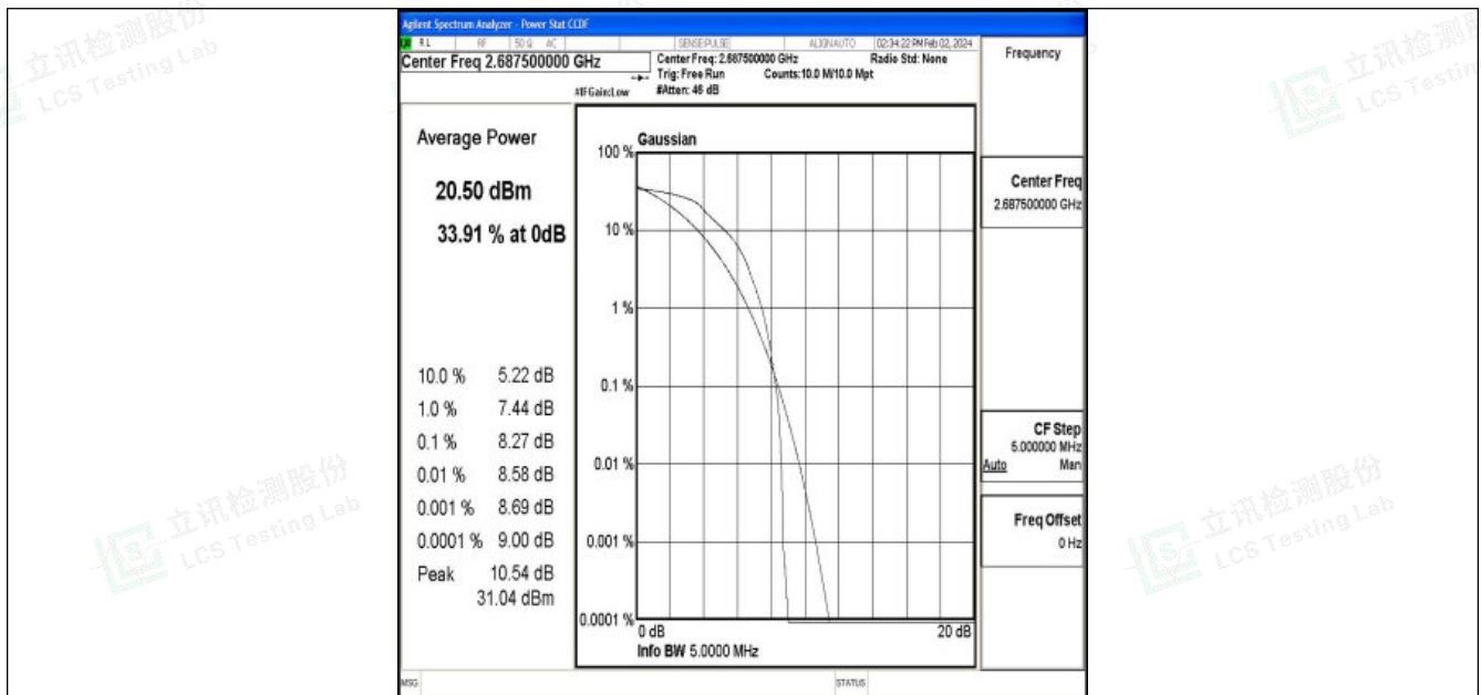
Band41-5MHz-QPSK-41565-1RB#0-PASS
