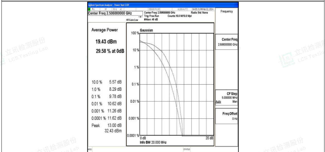
Band41-20MHz-16QAM-39750-100RB#0-PASS
