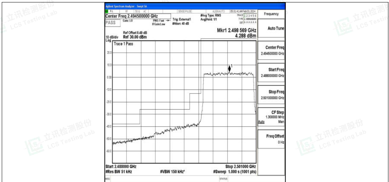
Band41_5MHz_16QAM_39675_25RB#0
