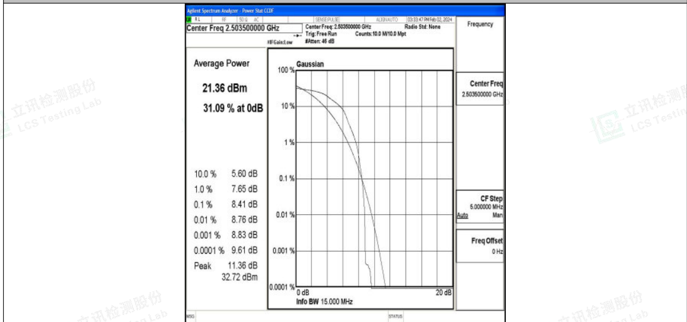
Band41-15MHz-16QAM-39725-1RB#0-PASS
