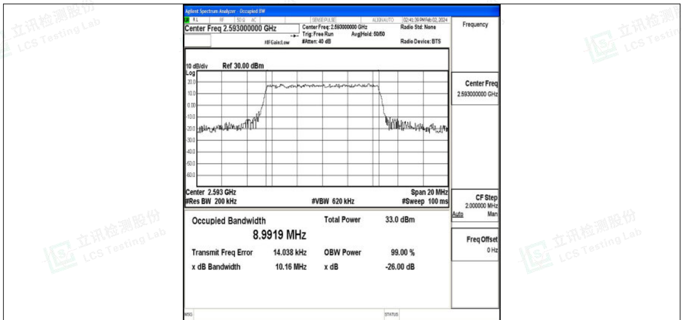
Band41-10MHz-QPSK-40620-50RB#0-PASS
