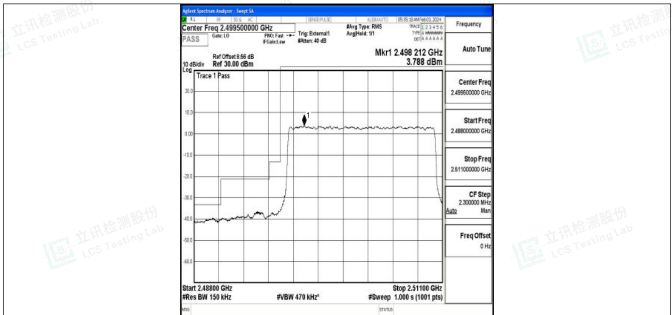
Band41_15MHz_16QAM_39725_75RB#0
