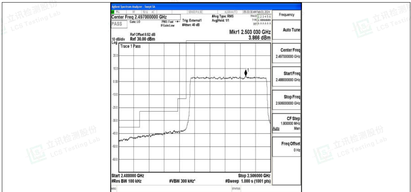
Band41_10MHz_16QAM_39700_50RB#0
