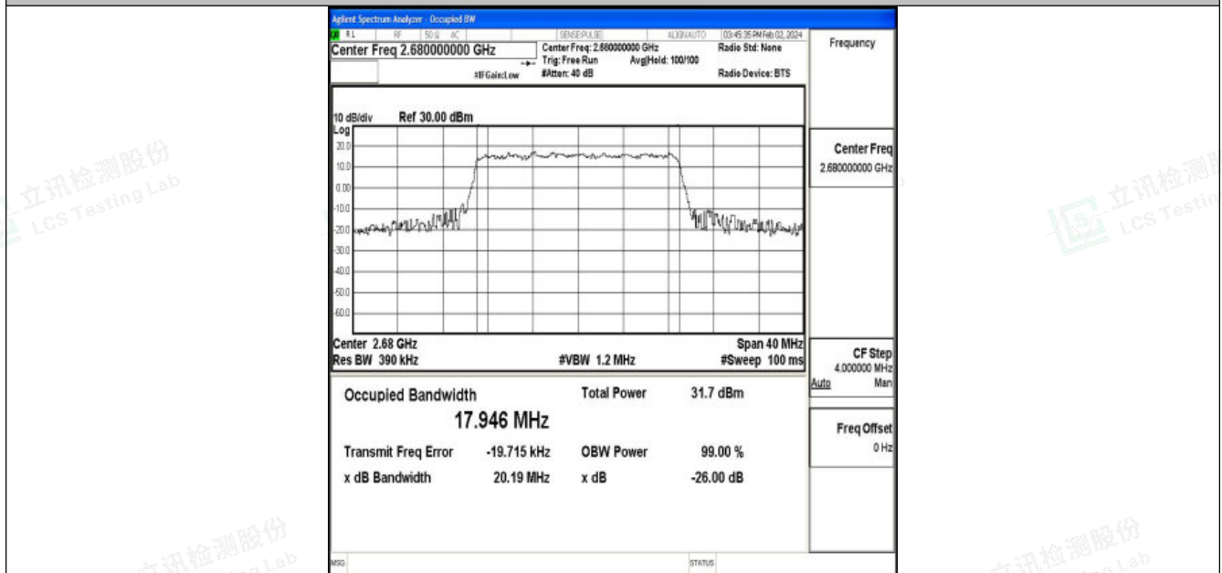
Band41-20MHz-16QAM-41490-100RB#0-PASS
