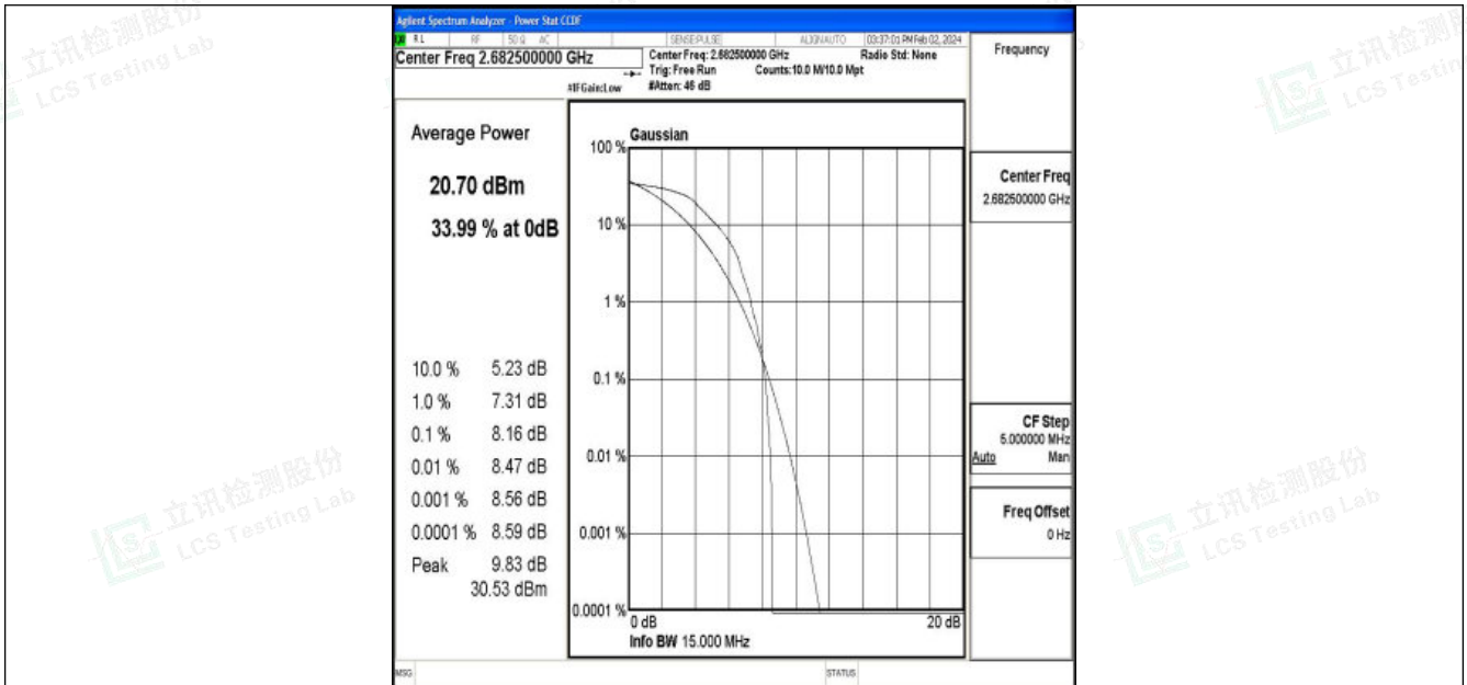
Band41-15MHz-QPSK-41515-1RB#0-PASS
