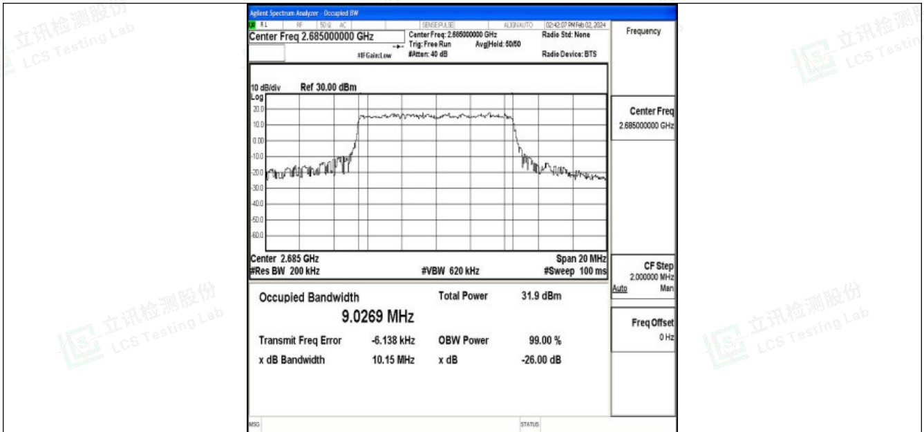
Band41-10MHz-QPSK-41540-50RB#0-PASS
