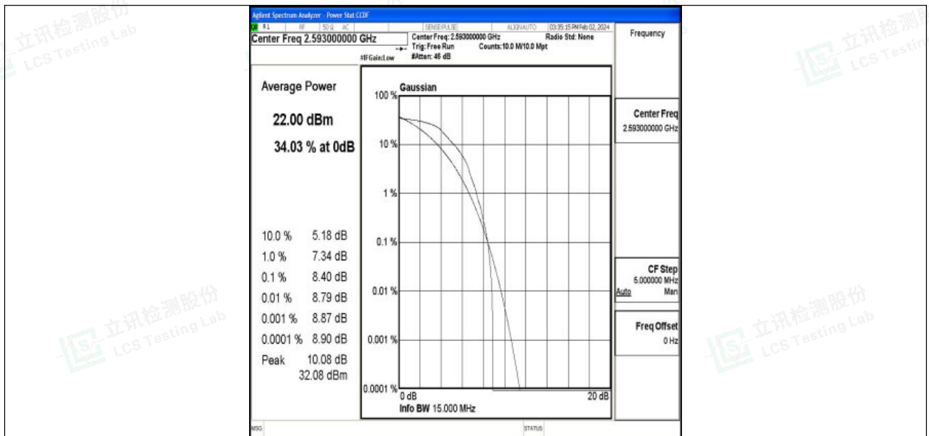
Band41-15MHz-QPSK-40620-1RB#0-PASS
