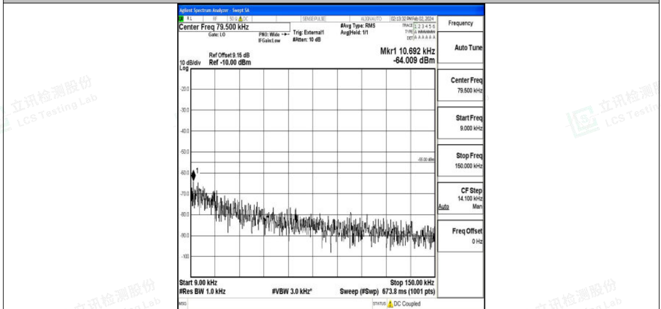
Band41_5MHz_16QAM_39675_1RB#0_0.009~0.15_0.009~0.15
