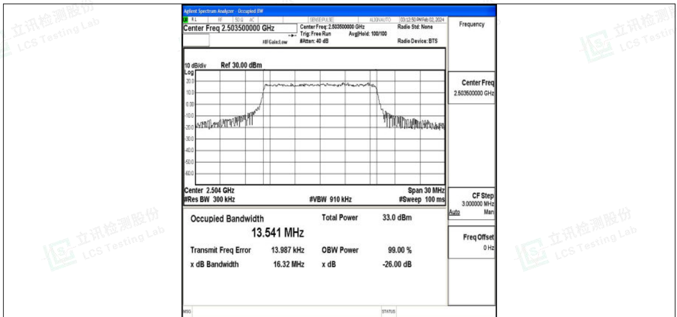
Band41-15MHz-QPSK-39725-75RB#0-PASS
