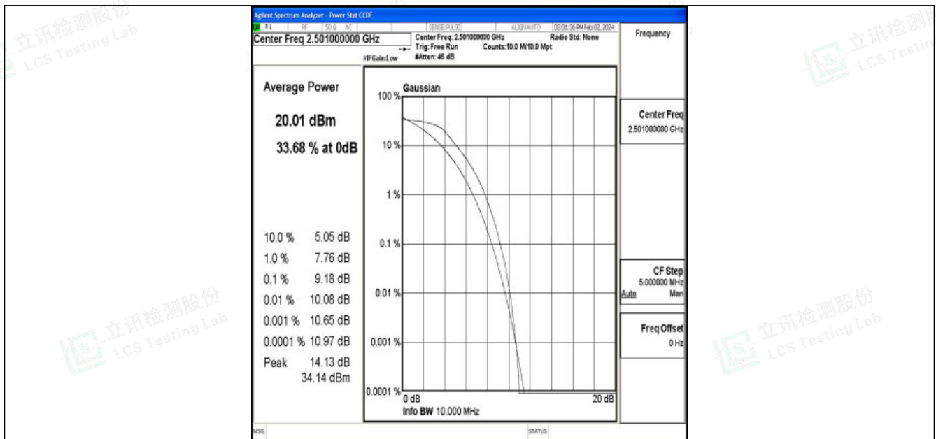
Band41-10MHz-QPSK-39700-50RB#0-PASS
