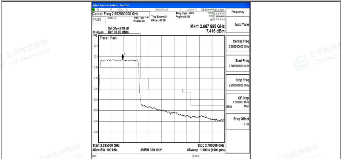
Band41_5MHz_QPSK_41565_25RB#0
