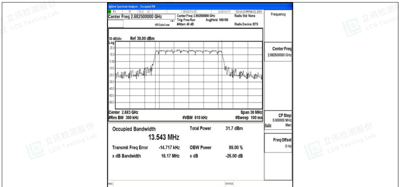
Band41-15MHz-QPSK-41515-75RB#0-PASS
