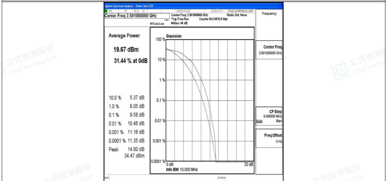
Band41-10MHz-16QAM-39700-50RB#0-PASS
