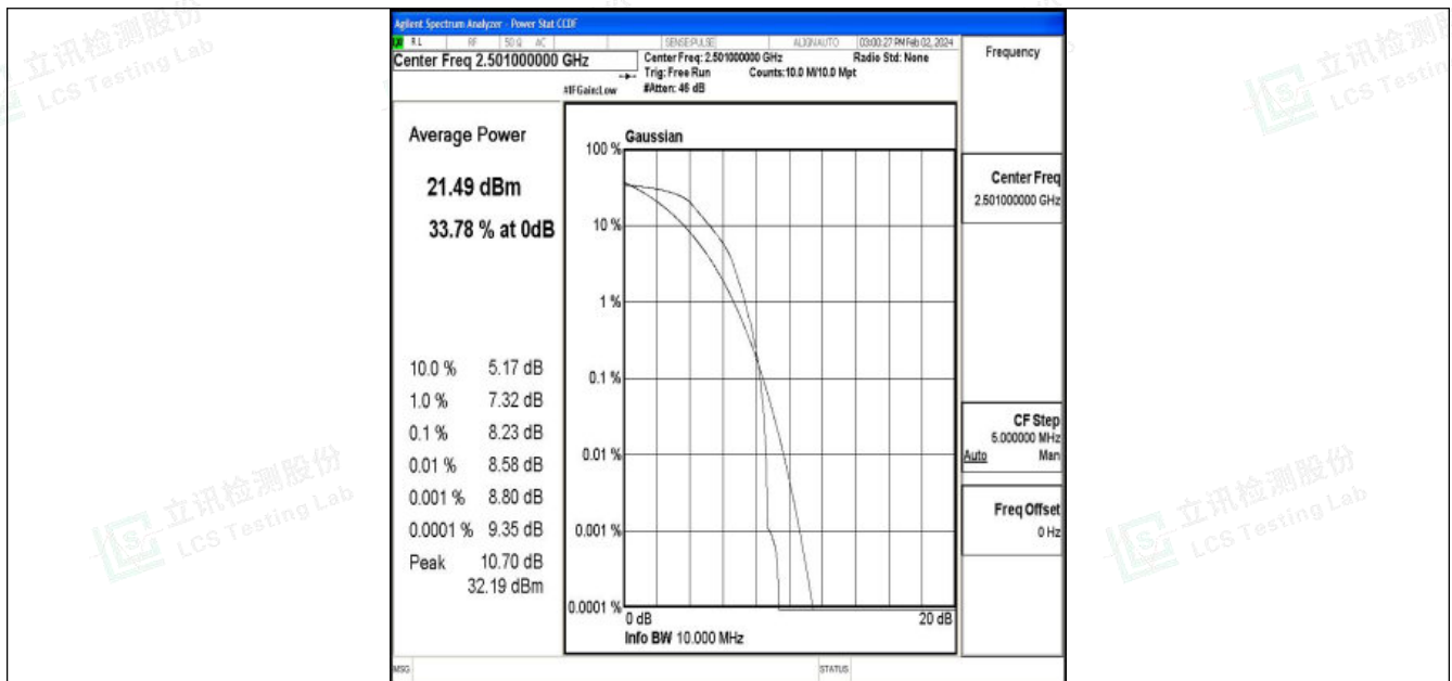
Band41-10MHz-QPSK-39700-1RB#0-PASS
