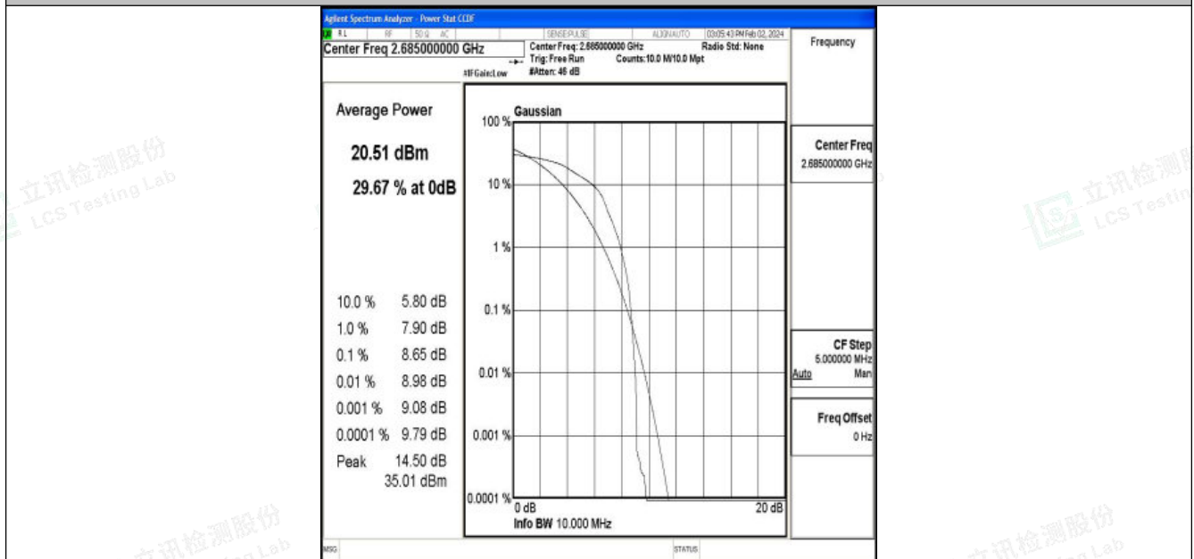
Band41-10MHz-16QAM-41540-1RB#0-PASS
