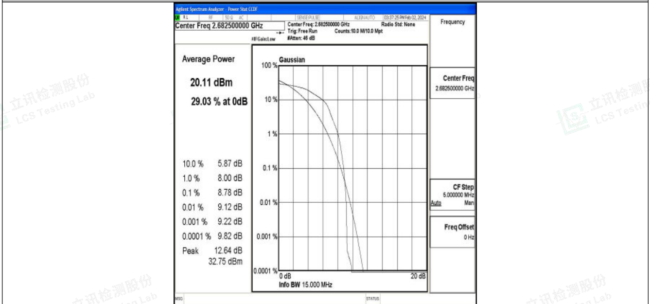
Band41-15MHz-16QAM-41515-1RB#0-PASS
