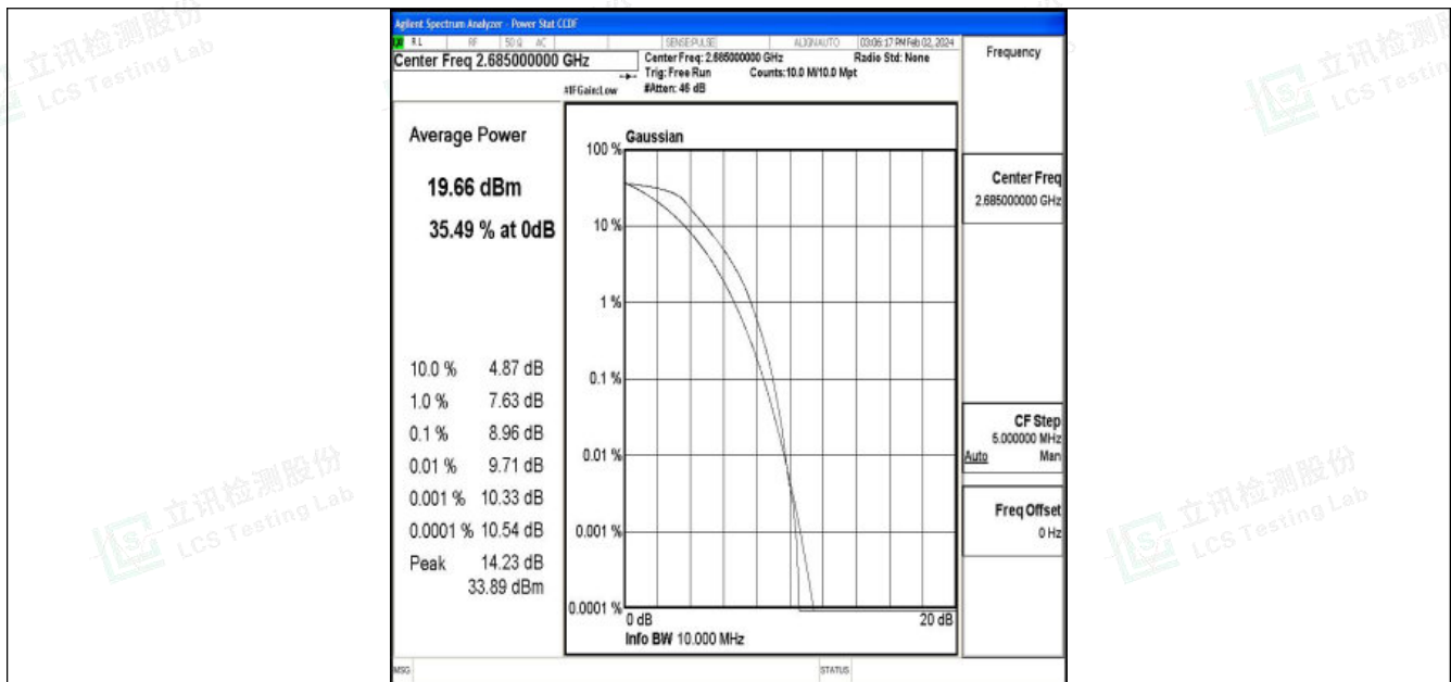
Band41-10MHz-QPSK-41540-50RB#0-PASS
