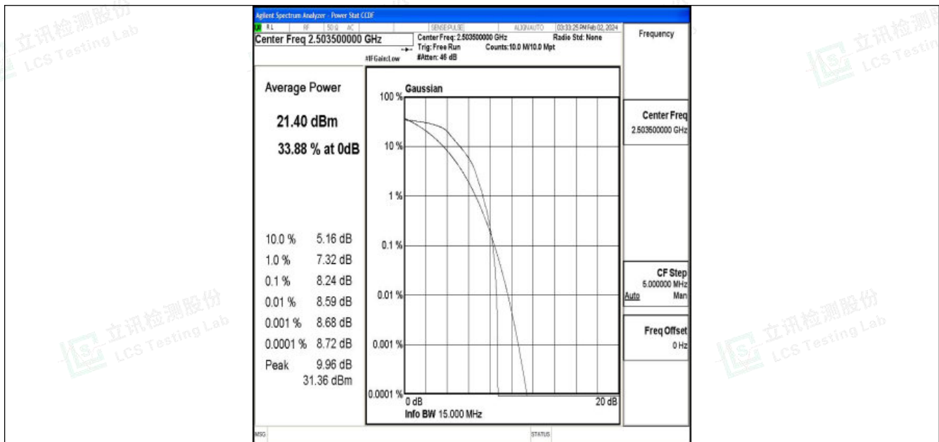
Band41-15MHz-QPSK-39725-1RB#0-PASS
