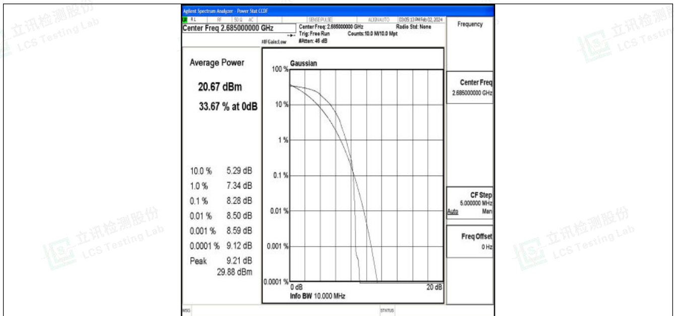
Band41-10MHz-QPSK-41540-1RB#0-PASS
