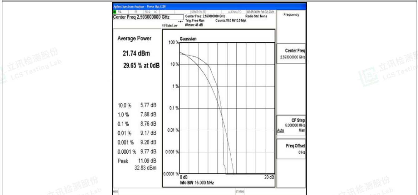
Band41-15MHz-16QAM-40620-1RB#0-PASS
