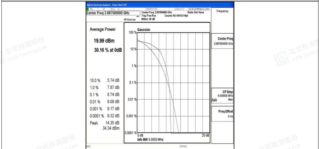
Band41-5MHz-16QAM-41565-1RB#0-PASS
