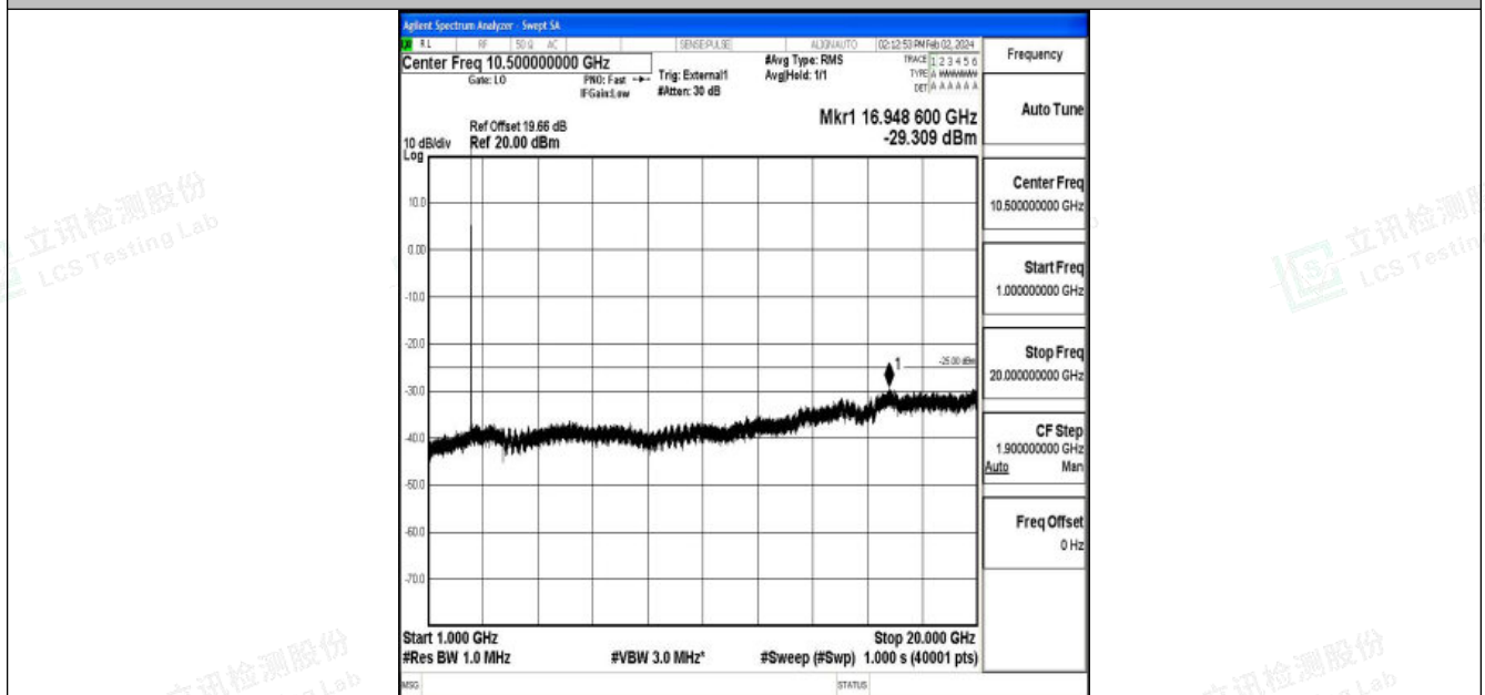
Band41_5MHz_QPSK_39675_1RB#0_1000~20000_1000~20000
