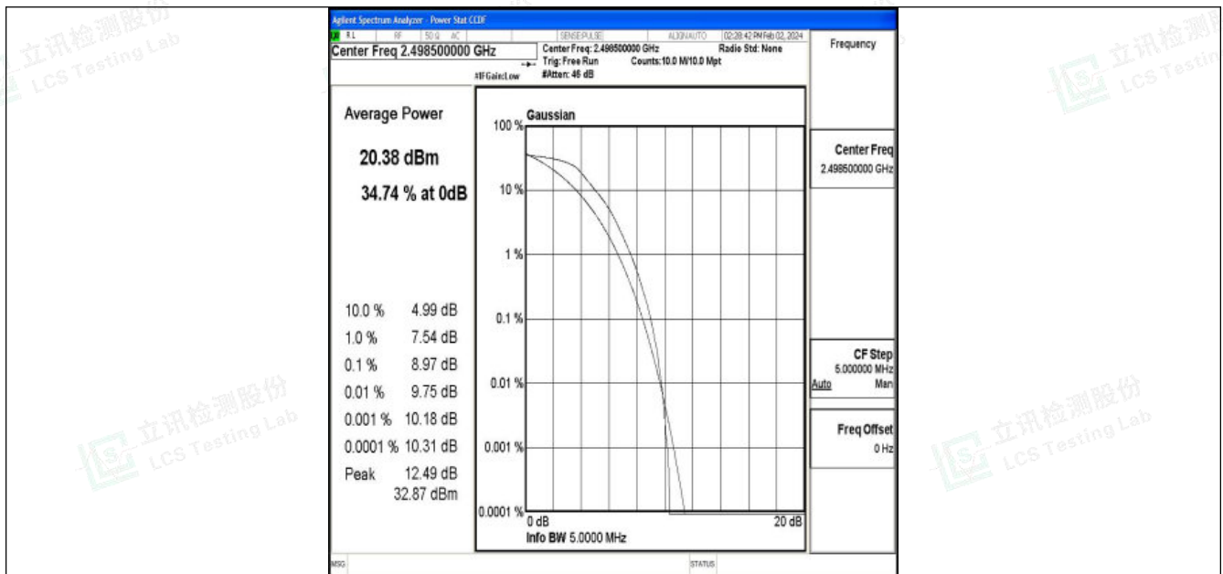
Band41-5MHz-QPSK-39675-25RB#0-PASS
