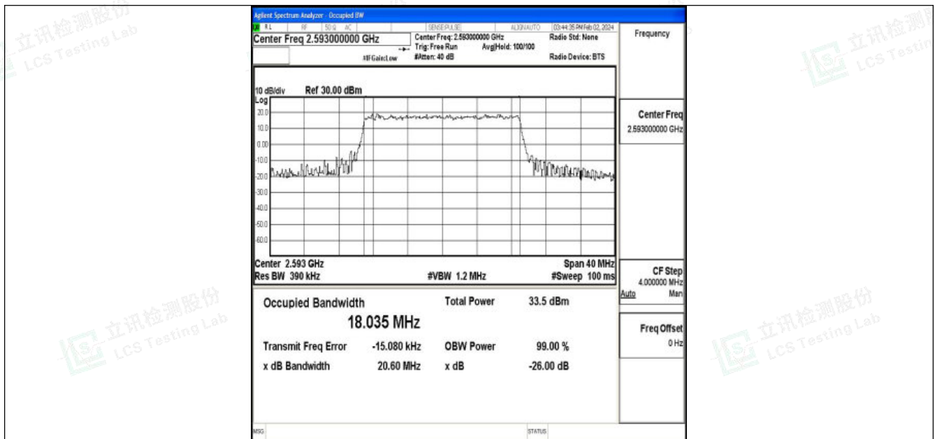
Band41-20MHz-QPSK-40620-100RB#0-PASS
