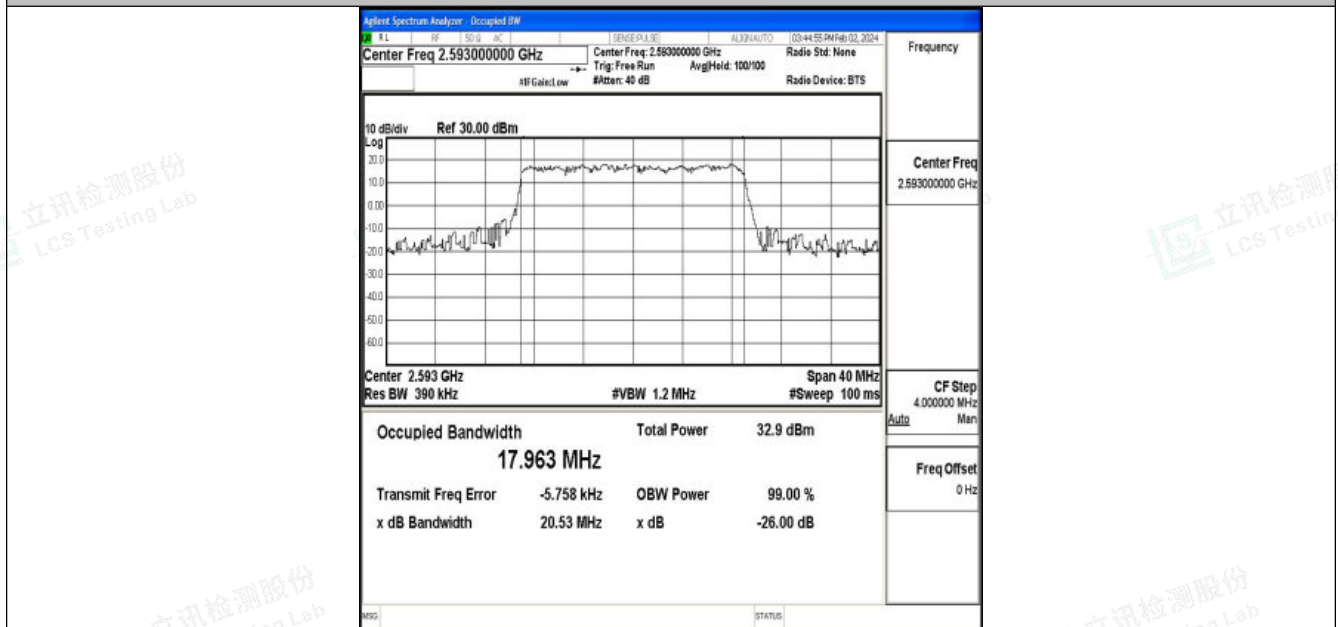
Band41-20MHz-16QAM-40620-100RB#0-PASS
