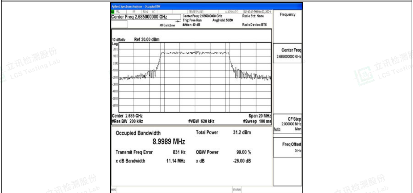
Band41-10MHz-16QAM-41540-50RB#0-PASS
