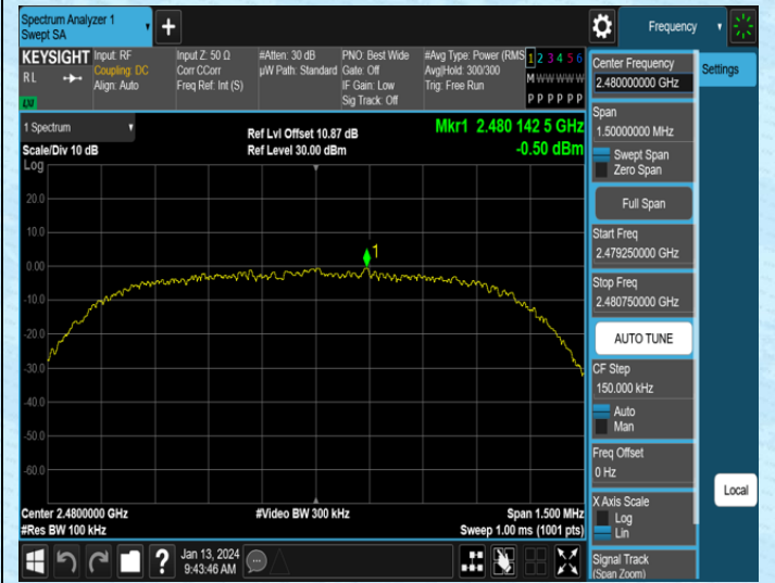
3DH5-Ant1-2480-0~Reference
