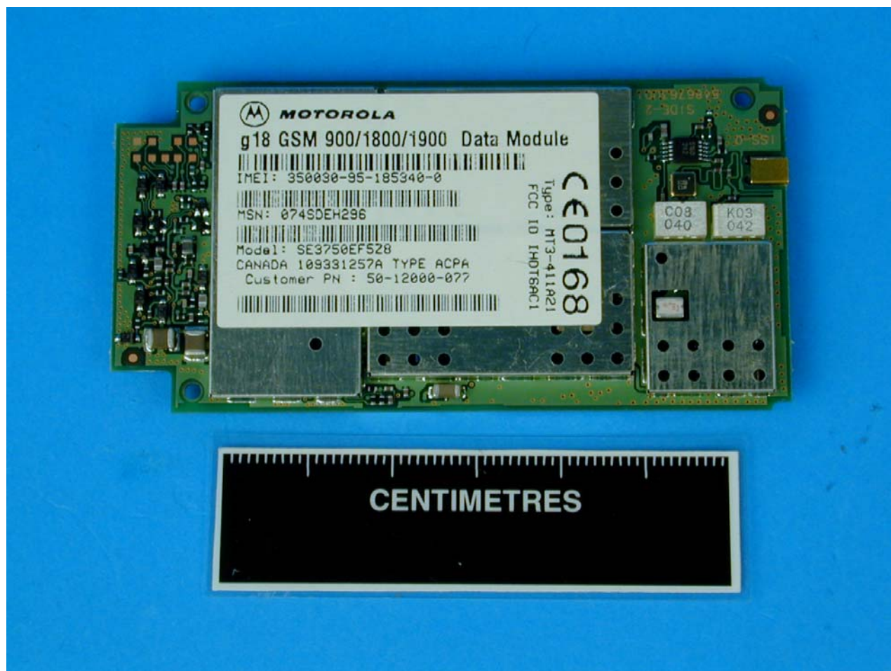
Photograph 14 4111-GPRS Front view of G18 GSM/GPRS Module
