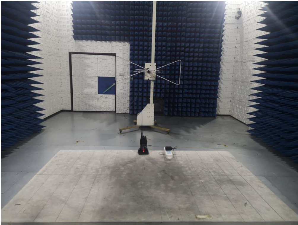
RADIATED EMISSION TEST SETUP-BELOW 1GHZ-SHORT ANTENNA
