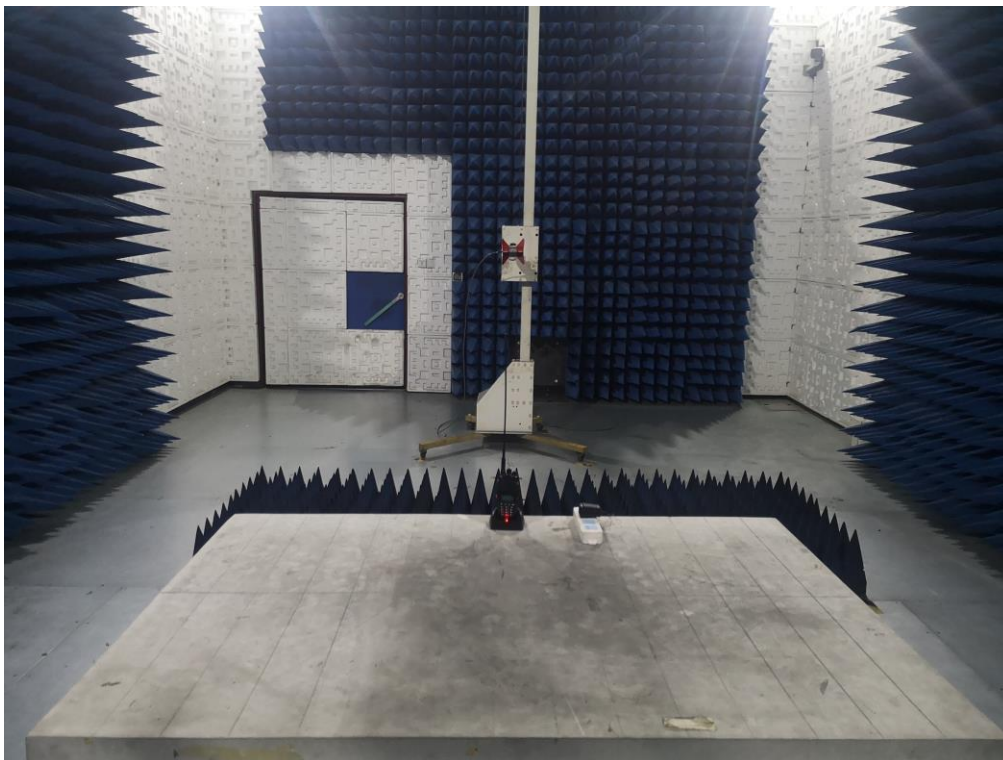
RADIATED EMISSION TEST SETUP-ABOVE 1GHZ-SHORT ANTENNA
