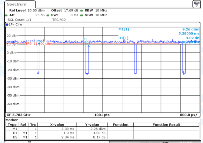
NTNV-11AC20SISO-Ant1-5785
