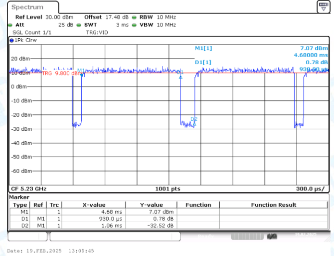
NTNV-11N40SISO-Ant1-5230
