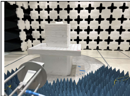
Radiated Emission Test 18-40GHz Front View
