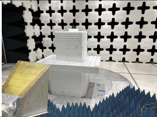
Radiated Emission Test 1-18GHz Front View
