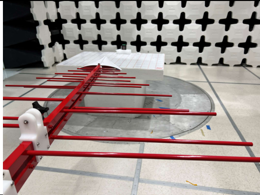
Radiated Emission Test below 1GHz Front View
