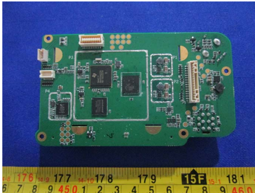
EUT –Control Panel Bottom Unshielded View
