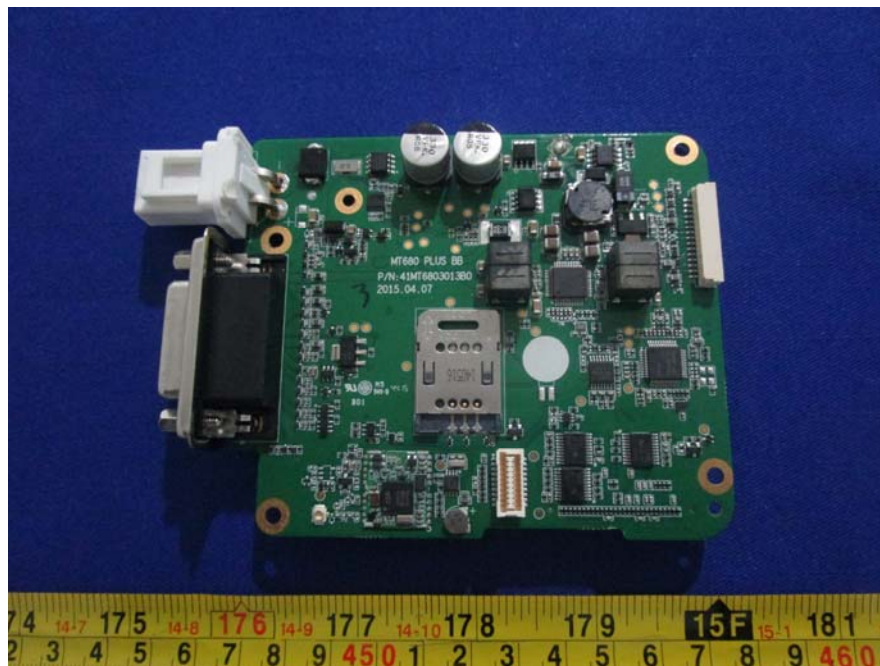
EUT –Sub Board Top Unshielded View
