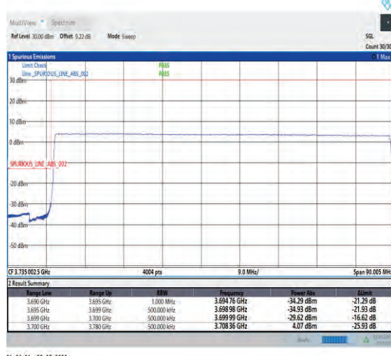
1-N77-3700-3980-PC1-30-80-L-6-CP-QPSK-Outer_Full-217@0-Ant1-1--PASS-see graph
