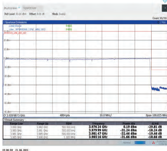
1-N77-3700-3980--30-90-H-6-CP-QPSK-Outer_Full-245@0-Ant1-PASS-see graph
