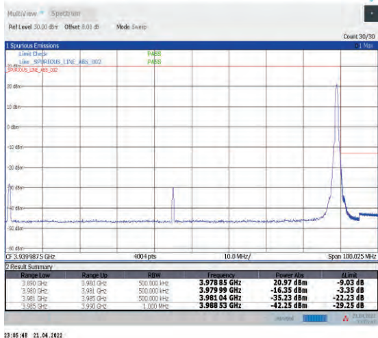
1-N77-3700-3980--30-90-H-2-DFT-PI2BPSK-Edge_1R_B_Right-1@244-Ant1-PASS-see graph
