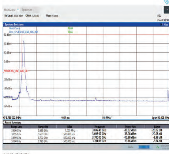
1-N77-3700-3980-PC1-30-80-L-4-CP-QPSK-Edge_1RB_Left-1@0-Ant1-1--PASS-see graph
