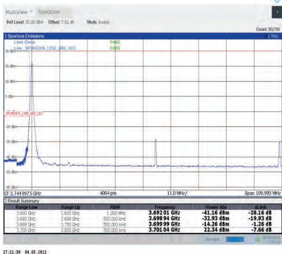
1-N77-3700-3980--30-100-L-1-DFT-PI2BPSK-Edge_1 RB_Left-1@0-Ant1-PASS-see graph
