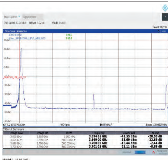
1-N77-3700-3980--30-90-L-1-DFT-PI2BPSK-Edge_1R_B_Left-1@0-Ant1-PASS-see graph
