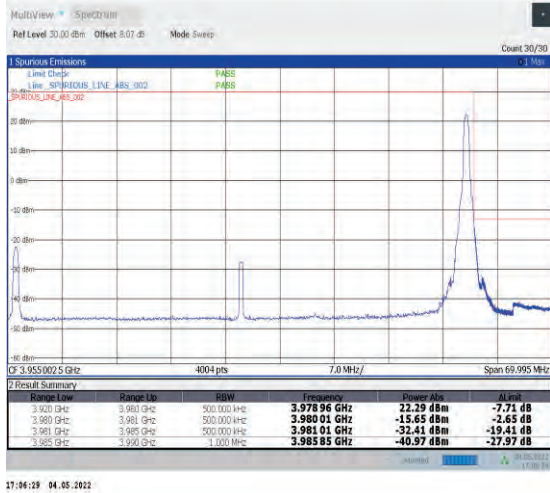
1-N77-3700-3980--30-60-H-2-DFT-PI2BPSK-Edge_1R_B_Right-1@161-Ant1-PASS-see graph
