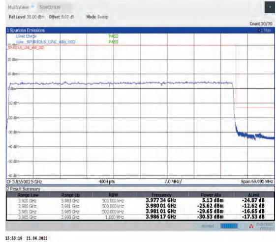
1-N77-3700-3980--30-60-H-3-DFT-PI2BPSK-Outer_Full-162@0-Ant1-PASS-see graph
