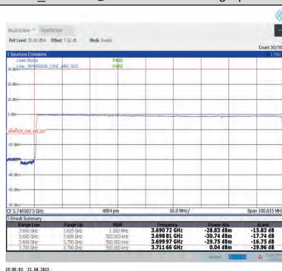
1-N77-3700-3980--30-90-L-6-CP-QPSK-Outer_Ful I-245@0-Ant1-PASS-see graph
