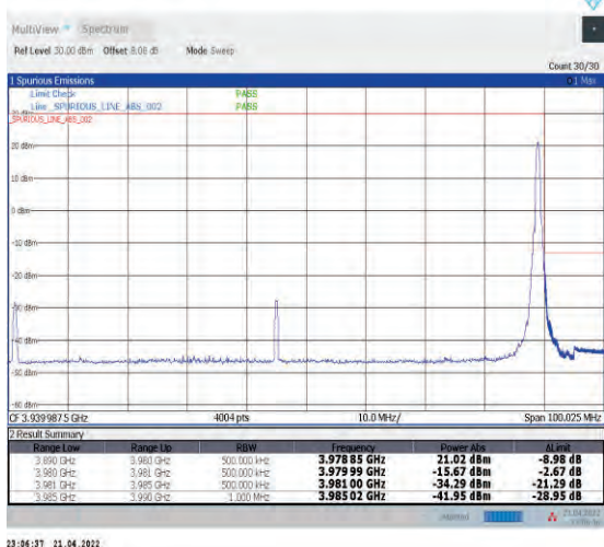
1-N77-3700-3980--30-90-H-5-CP-QPSK-Edge_1RB_Right-1@244-Ant1-PASS-see graph
