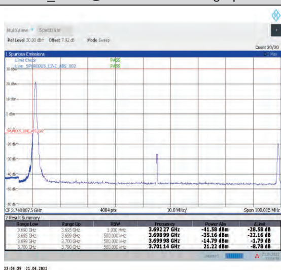
1-N77-3700-3980--30-90-L-4-CP-QPSK-Edge_1RB_L eft-1@0-Ant1-PASS-see graph
