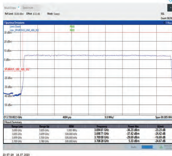
1-N77-3700-3980-PC1-30-80-L-3-DFT-PI2BPSK-Outer_Full-216@0-Ant1-1--PASS-see graph
