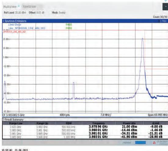
1-N77-3700-3980--30-60-H-5-CP-QPSK-Edge_1RB_Right-1@161-Ant1-PASS-see graph
