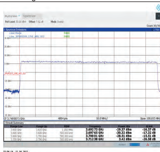
1-N77-3700-3980--30-90-L-3-DFT-PI2BPSK-Outer_Full-240@0-Ant1-PASS-see graph
