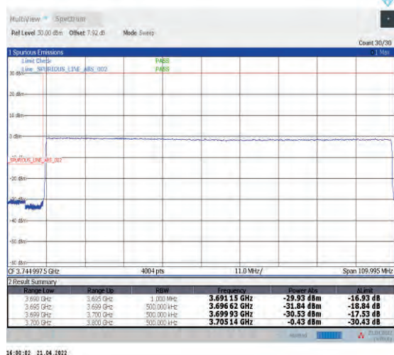
1-N77-3700-3980--30-100-L-6-CP-QPSK-Outer_F ull-273@0-Ant1-PASS-see graph
