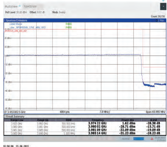
1-N77-3700-3980--30-60-H-6-CP-QPSK-Outer_Full-162@0-Ant1-PASS-see graph
