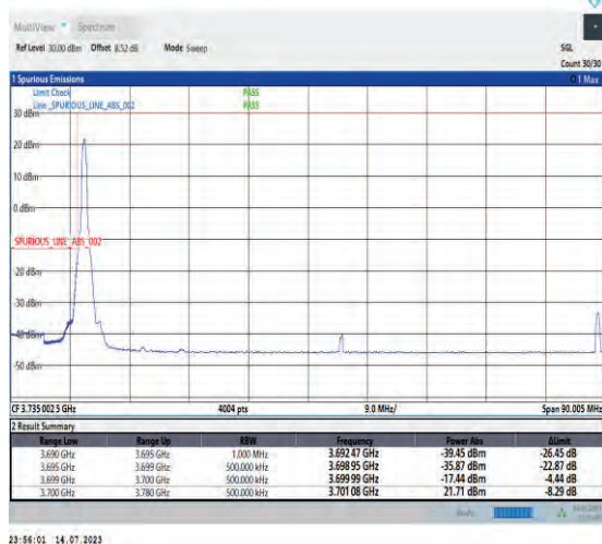
1-N77-3700-3980-PC1-30-80-L-1-DFT-PI2BPSK-Edg_e_1RB_Left-1@0-Ant1-1--PASS-see graph
